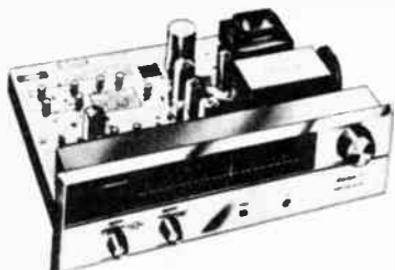
MODEL 312 FM STEREO TUNER
