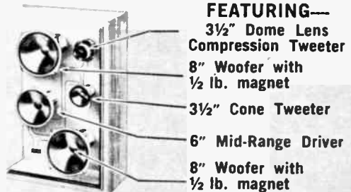
SK-270 DECORETTE II
