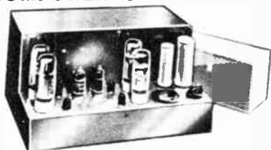
DUAL 35-WATT STEREOPHONIC POWER AMPLIFIER
