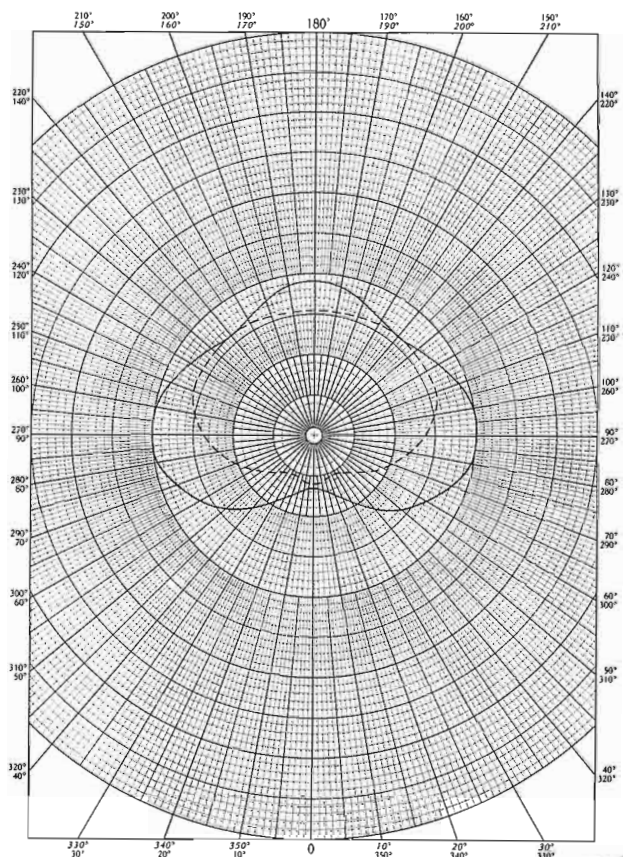
PATTERN "B" Horizontal Relative Field Patterns Solid line—horizontal polarization VRMS 0.798 Dashed line—vertical polarization VRMS 0.619
