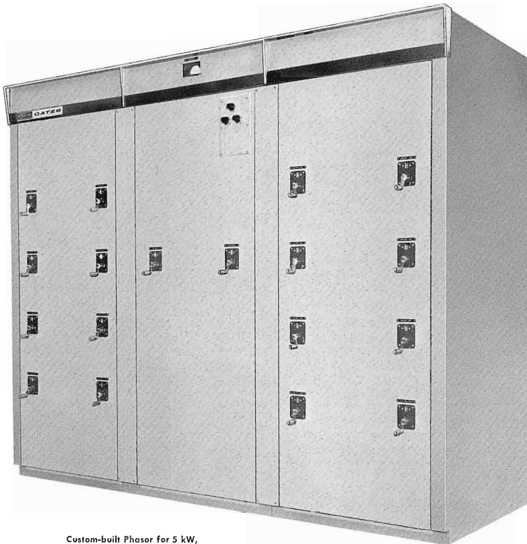
Custom-built Phasor for 5 kW, 5-tower directional AM station.
