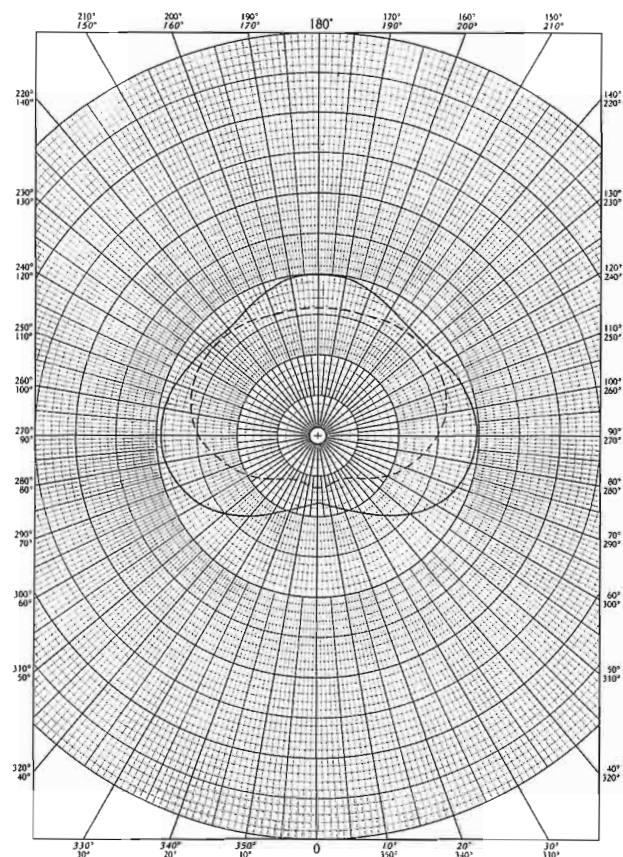
PATTERN "A" Horizontal Relative Field Patterns Solid line—horizontal polarization HRMS 0.830 Dashed line—vertical polarization HRMS 0.659
