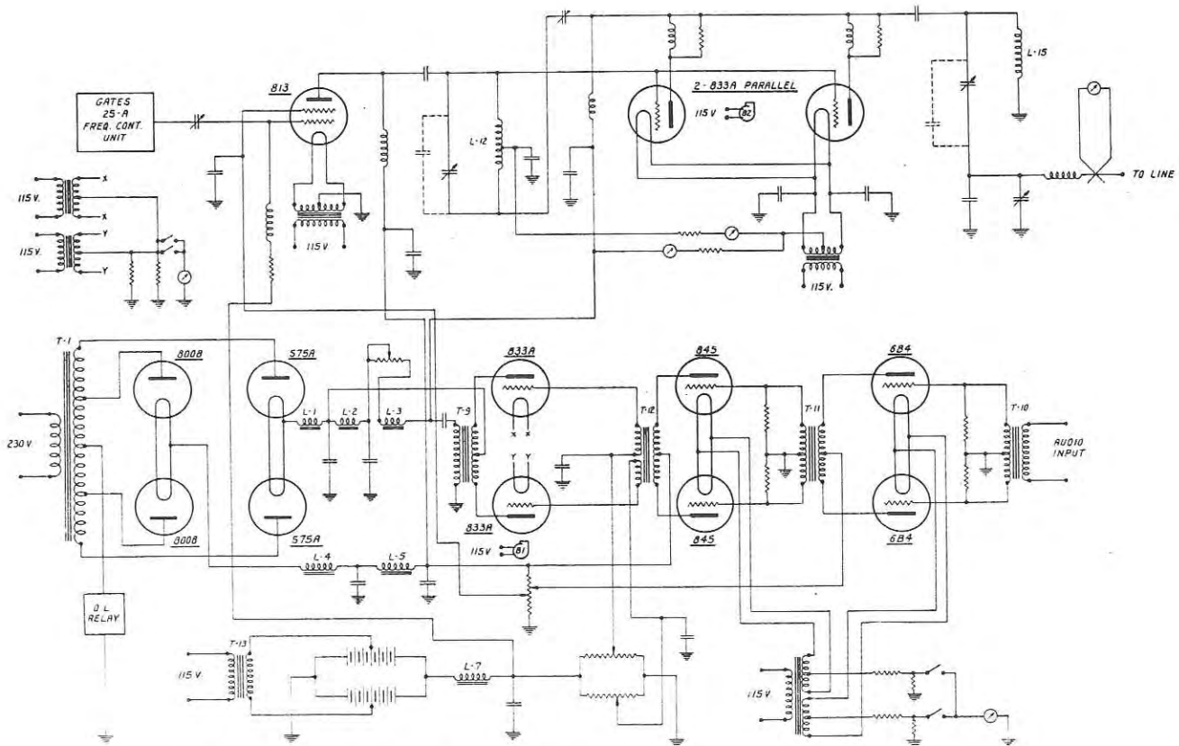
This simplified schematic of the BC-1E transmitter shows the fundamental electrical arrangement.
