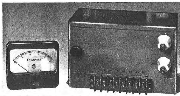
Remote antenna current diode unit, MO-2765-A. The meter provided matches those along the top of the BC-1E transmitter.
