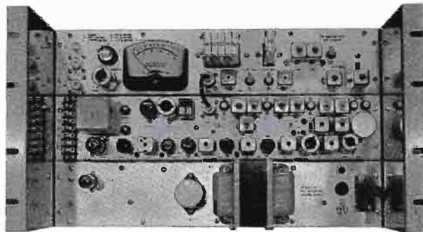
MR-200/942-952 Receiver.
