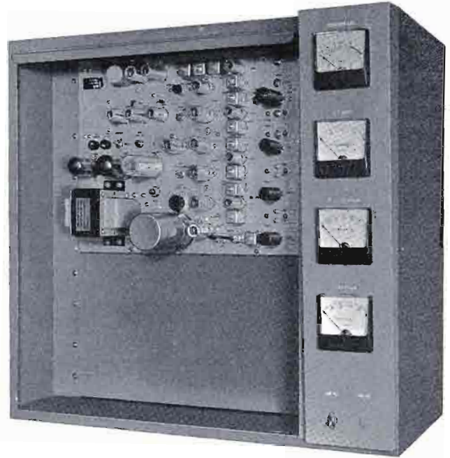
Front view (cover removed) of Model BFE-10C, ten watt FM transmitter. Models BFE-50C and BFR-50C are essentially the same in appearance.
