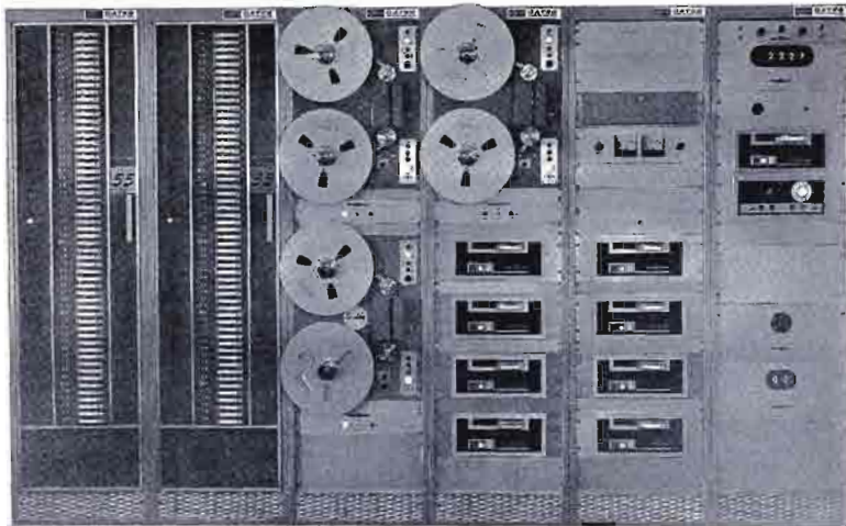
Top adult rated west coast AM/FM station with middle-of-the-road format carries its large commercial load in two Criterion 55's (capacity 55 cartridges each), with music on reel-to-reel tape. Time announcements are automatic, from two Criterion cartridge tape decks, and program logging is handled by an automatic logger (not shown).
