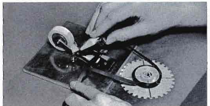
"Magnifying glass" attention is given to splicing tolerances to minimize "drop out" upon playback.
