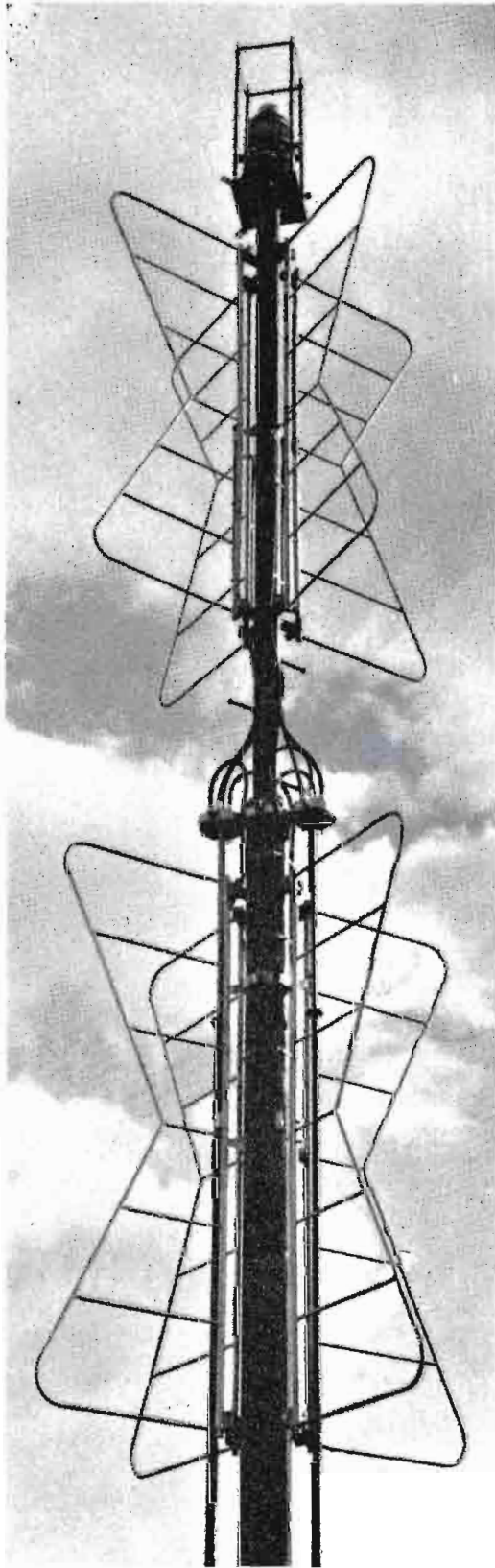
Jampro JAT 2/5 two bay Channel 5 batwing antenna.
