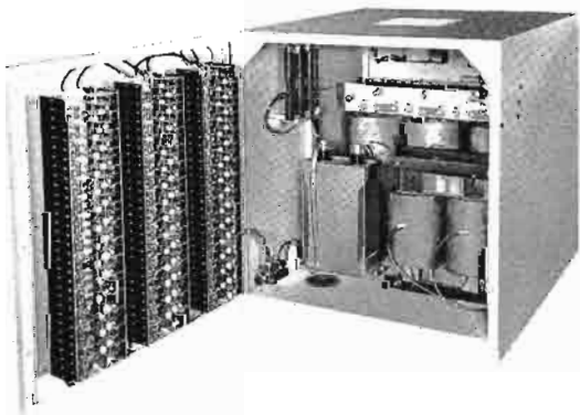
Compact high voltage power supply cubicle may be installed adjacent or at a distance from the FM-20G transmitter proper. Note silicon rectifiers and heavy duty components for long life and insured reliability.
