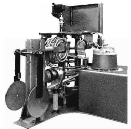
R.F. driver showing type 4CX15000 stage with grid circuits and cooling plenum.
