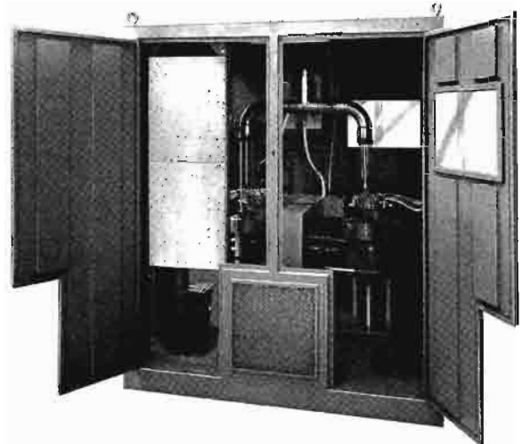
Modulator cabinet showing 4CV100,000C tubes and vapor phase cooling system.
