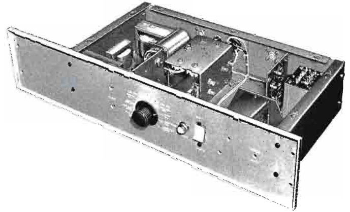
Built-in multimeter constantly monitors the operating conditions of the complete driver/modulator. A front panel switch permits instant switching from one oscillator to the other.
