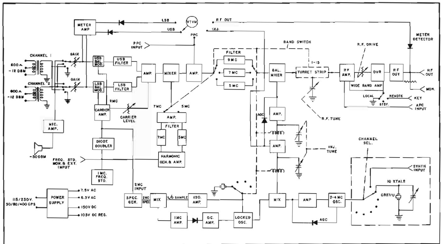
BLOCK DIAGRAM—SG-70
