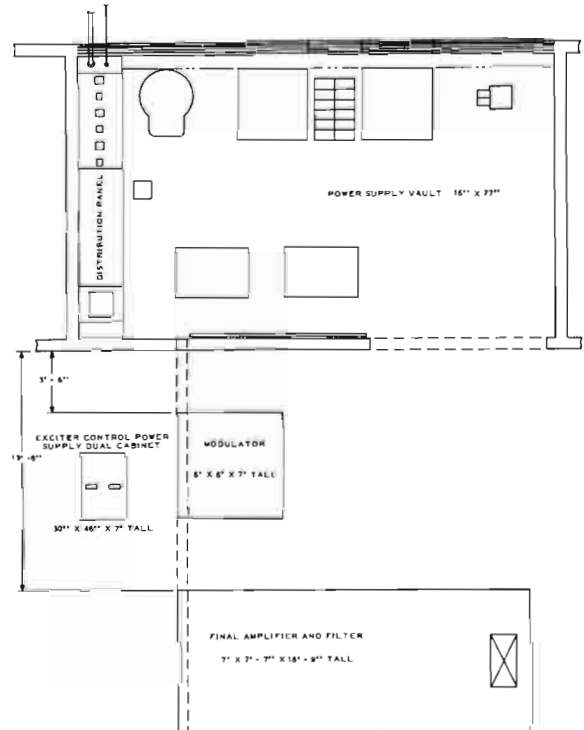
FIGURE 1-5. PROPOSED FLOOR PLAN.
