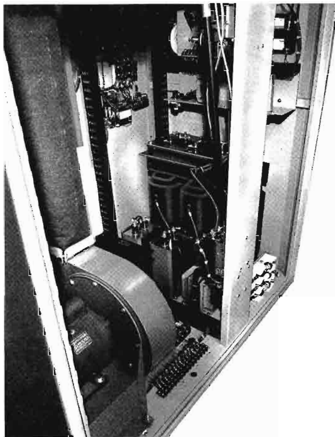
Accessibility, logical design and excellent workmanship are all illustrated in this back view with door and panel removed.
