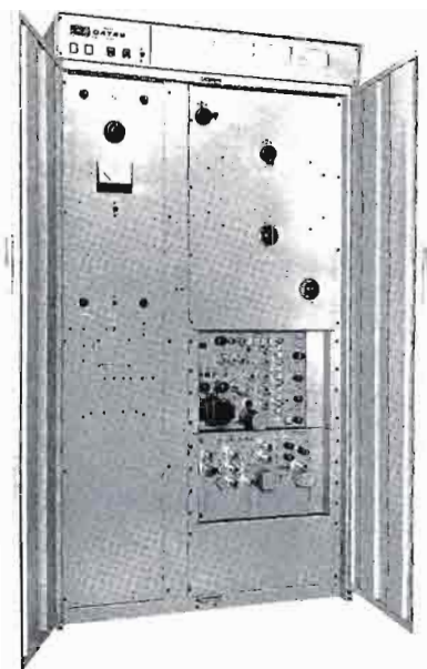
FM-20G, Front View—doors open. The optional stereo generator is shown below the cascade exciter.
