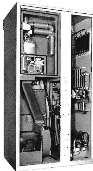
Rear view. Accessibility to all components is a major feature of the FM-20G.
