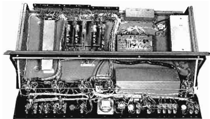
The smooth and easy to service design combined with the smaller size of transistorized components is best evidenced by the open view above. Note the plug-in amplifiers to the left, cue intercom speaker near center front and hinge down front panel and hinge up cabinet cover. "Control Center" is the shielded portion to the right of the cue speaker.
