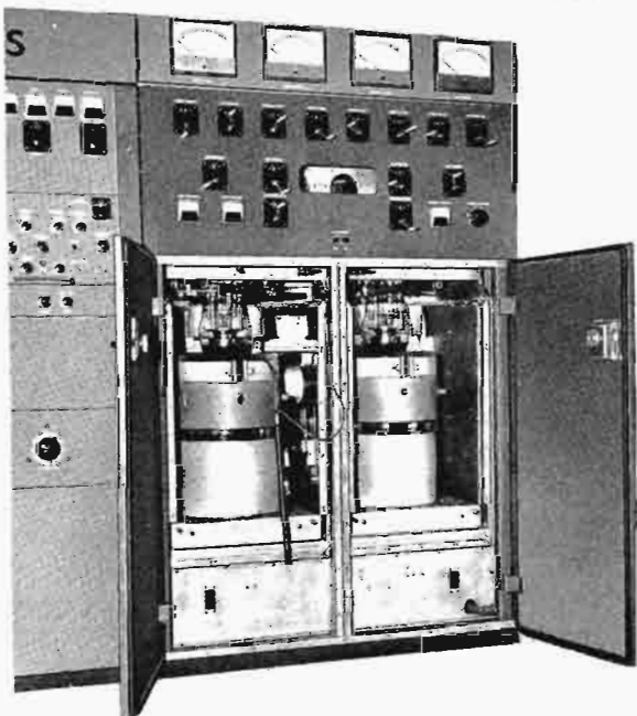
Front view PA cubicle with internal shields removed.
