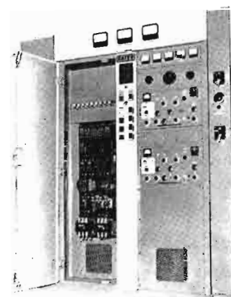
The exciter is located in the center cubicle and also includes the heart of the control system as shown above. There is sufficient space for optional dual exciters permitting operation on twenty crystal controlled channels where desired.
