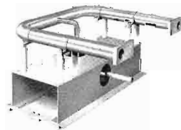
"Latch-on" 18-22 Mc. Tank coil assembly. Rapid change of tank coils permits frequency change-over to be made in three minutes.
