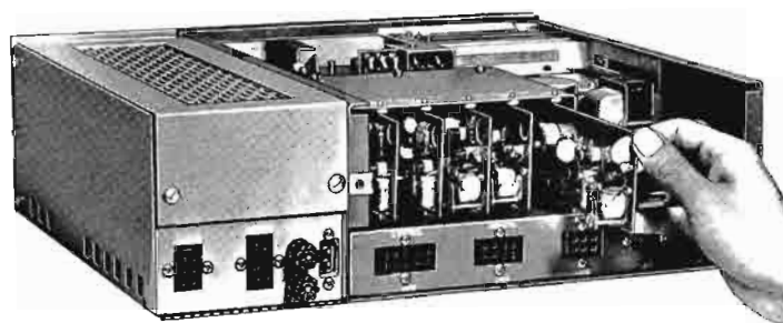
Rear view shows plug-in amplifiers which tailor system to meet individual requirements. Cartritape II can be expanded at any time with additional plug-in amplifiers. (Fig. 1).
