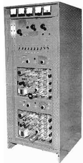
The 250 Watt FM Transmitter with dual 50 watt driver's, Model SFM-250 is shown with front panel removed.
