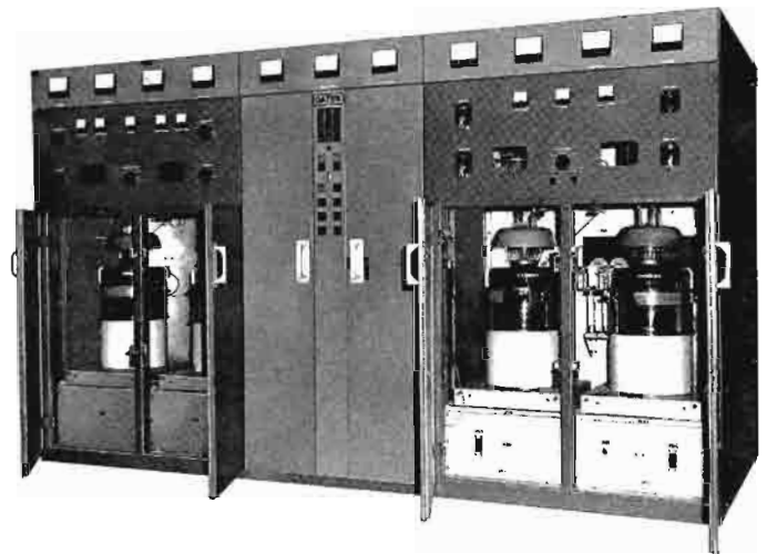
Three main transmitter cubicles house (from left to right) the modulator, RF driver, and power amplifier.
