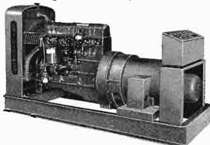
Model 25G60 Generator for 25 KW continuous duty service.
