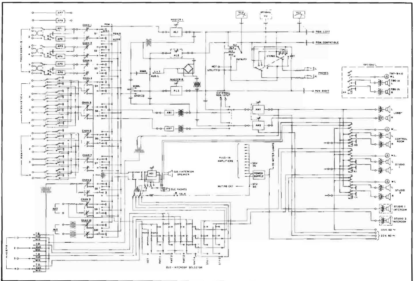
Block Diagram.
