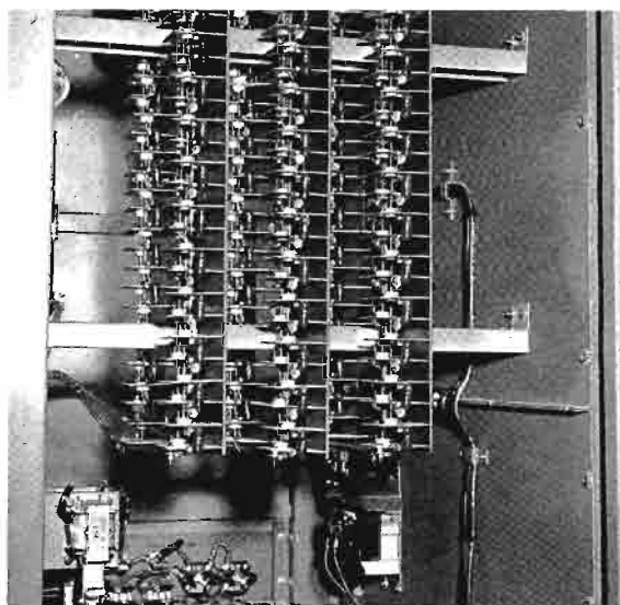
One hundred and Fifty Silicon Cells each Rated at 400 P.F.V. at 18 Amperes Provide a 3 to 1 Voltage and 10 to 1 Current Safety Factor.
