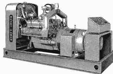
Model 50G60 Generating Plant for 50 KW continuous duty service.
