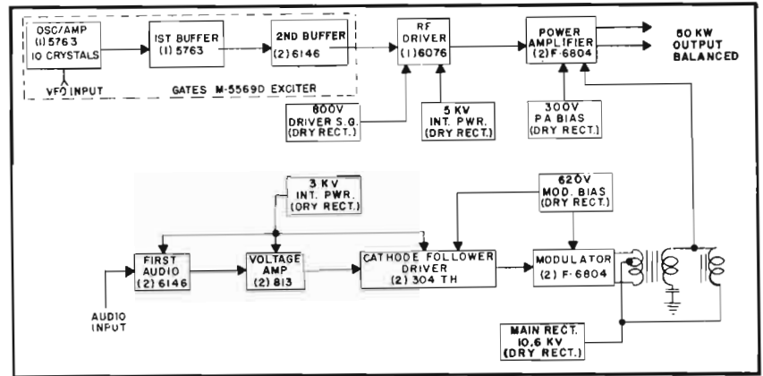
Block diagram
