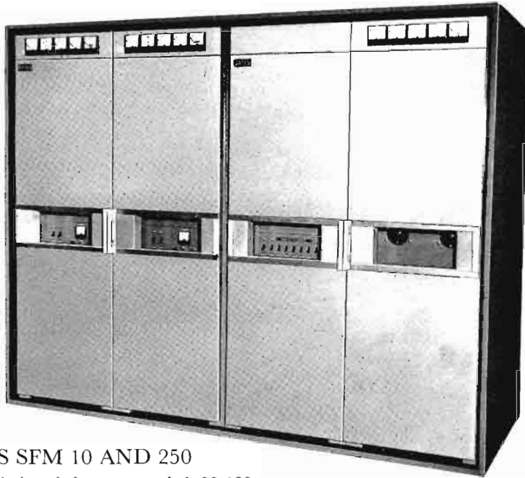
The SFM-10 FM Transmitter consists of two complete 1000 watt transmitters, (either one may be used as the driver) and the 10,000 watt amplifier.
