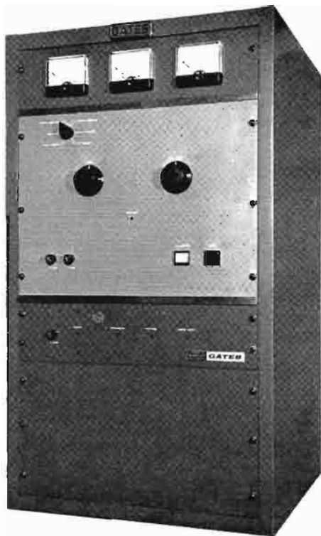
Above, the BC-01G transmitter is shown without audio input system. The audio input is 600 ohms and RF output is 50 ohms. Transmitter is fully transistorized except the single power output tube and no warm-up cycle is required.
