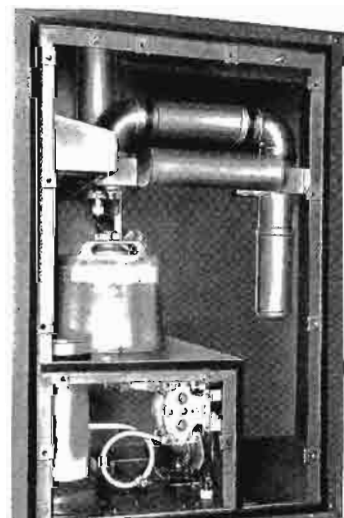
The Power Amplifier stage, which uses a 4CX15000A ceramic tube, has its driver amplifier located directly below for added efficiency of operation.
