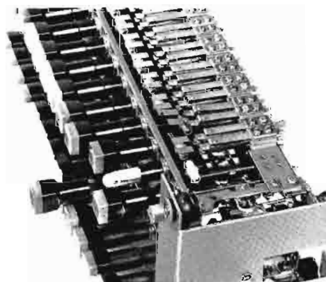
"Control Center" is built as heavy as the service demanded of it. Strong PBX type push keys with gold plated contacts automatically release if another is inserted. Handles are color coded and illuminated when circuit is in use. Control Center also provides voltage to operate mechanical devices. In "Control Center" two mixing channels do the work of 12.
