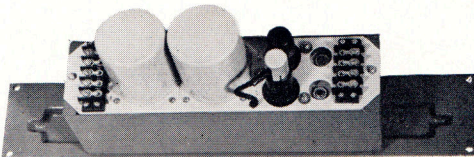
Figure D—Back view of SA-72 or SA-75 rack mount preamplifiers. Note the shock mounting of tubes, test jacks for plate current, metering and isolation of input and output terminations.
