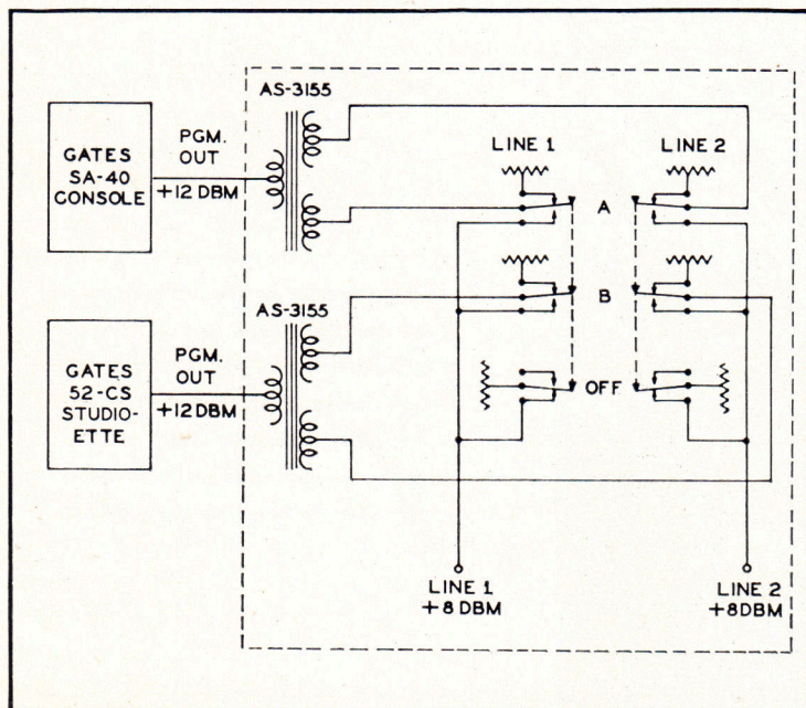
FIGURE A—The SA-104 circuit arrangement showing how two program circuits can be multiplied into two lines, adding greatly to the reserve facilities of the speech input equipment when not in use for separate AM and FM broadcasting.
