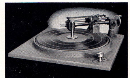
Figure B—The CB-12 recording chassis with overhead mechanism and DU4 cutter. See Page 29 for technical drive information.
