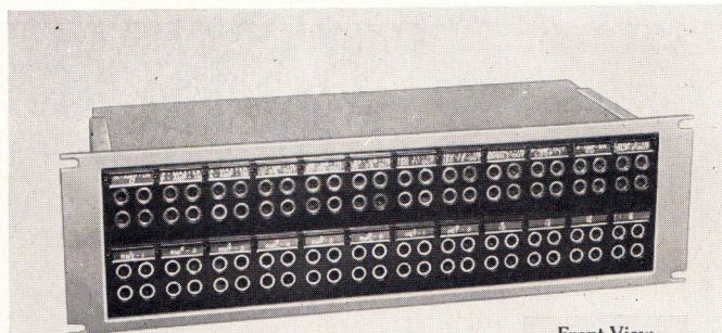
Front View C-1500-M2 and SA-1601
