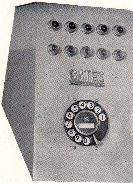
FIGURE A —Illustrates above the desk type dial circuit selector. This houses the dialing unit, circuit indicating lights and terminal connections which operate the stepping and control relays mounted on a separate rack panel. Its small size of 6\frac{3}{4} inches wide and 10\frac{1}{2} inches high makes it convenient for any type of desk mounting.
