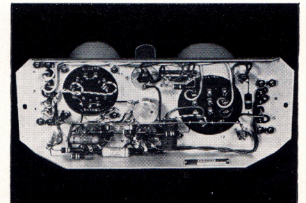
Figure G—The under chassis wiring of the SA-93 isolation amplifier illustrates the excellent workmanship of even the simplest of amplifier equipments.
