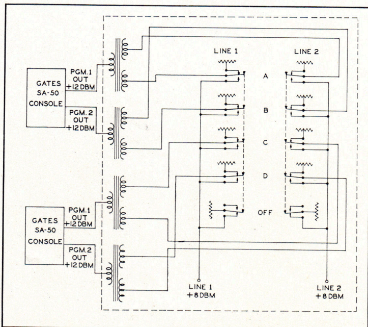
FIGURE B—Model SA-105 program switching equipment. Here four output circuits may be arranged in any combination to two program lines without danger through switch interlocking of interposing two programs on one circuit.
