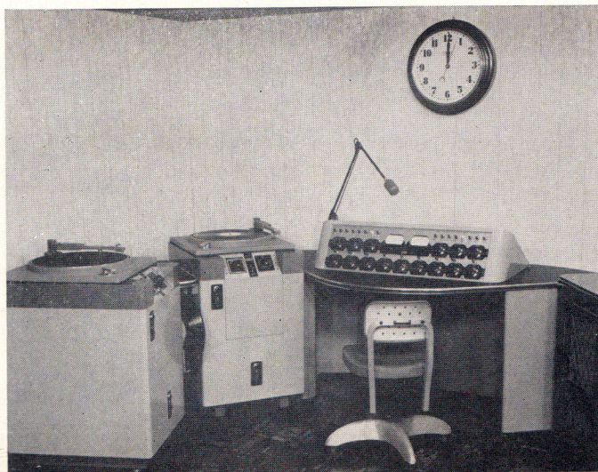
Illustration of CB-60 Desk with SA-50 Dual Console. Pages 33, 34 and 35 list many desk combinations.
