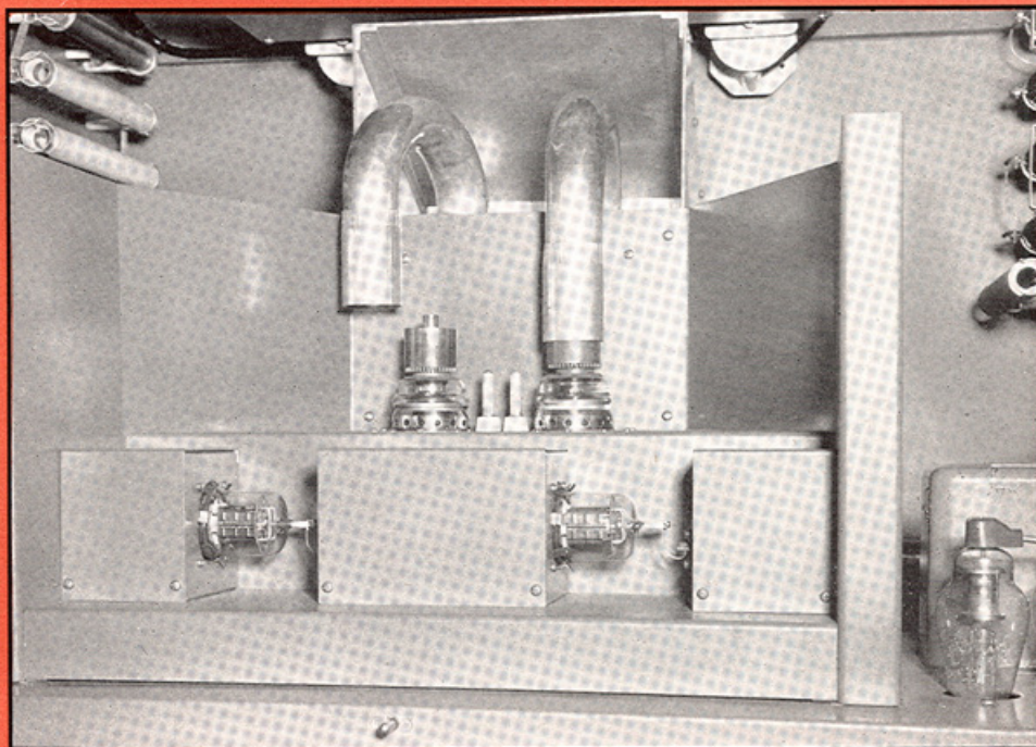
Power amplifier tubes can be removed by sliding the plate connectors upward on the tuning elements, then turning the elements to one side.
