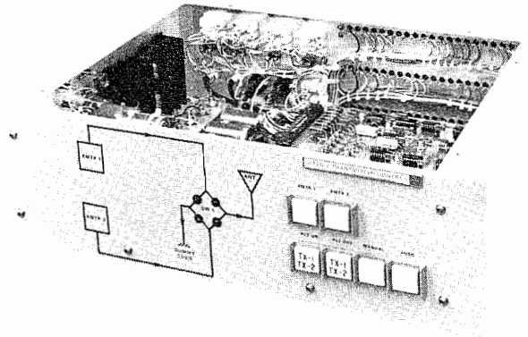
377D-2 Automatic Transmitter Switcher
