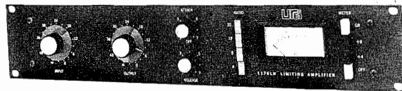
Universal Audio 1176LN Limiting Amplifier
