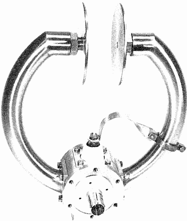
37M FM Antenna
