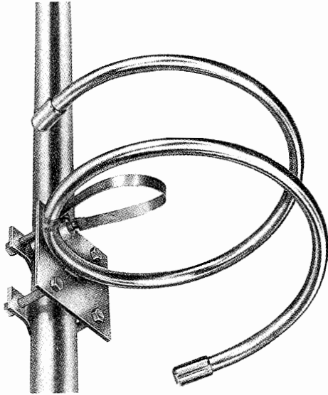
Circularly Polarized Educational Antenna
