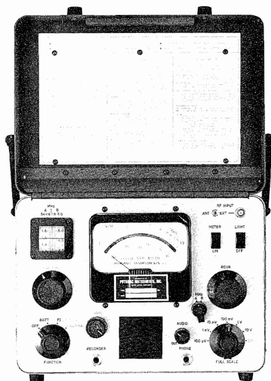
FIM-21 Field Intensity Meter
