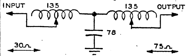
APPROXIMATE NUMBER OF TURNS REQUIRED IN T-SECTION COILS TO MATCH 75Ω LINE.
