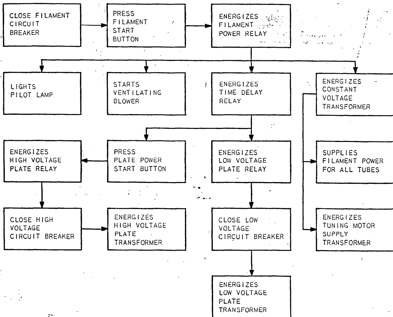
Figure 3-9. Block Diagram of Power Circuit Check
