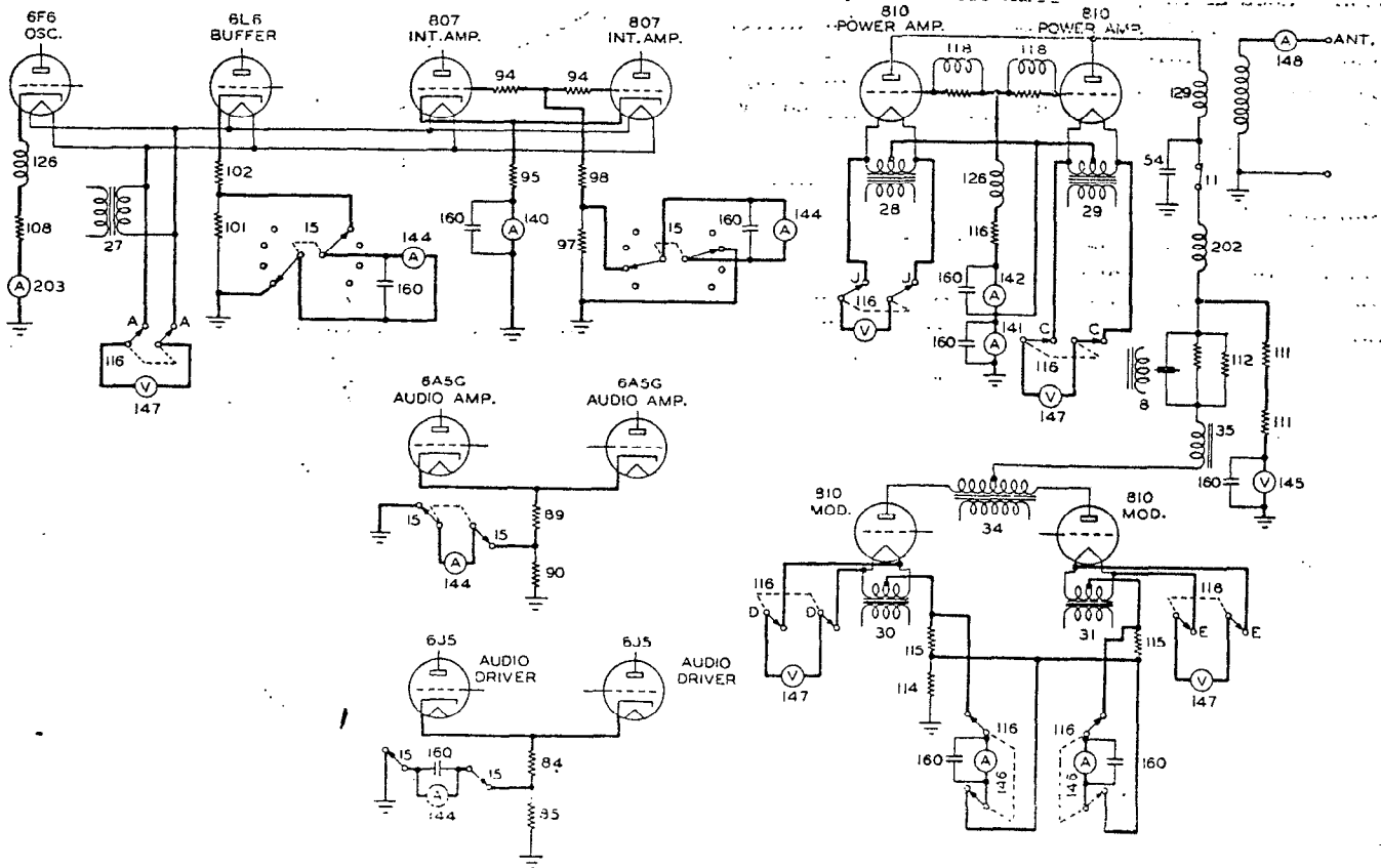
Figure 2-13. Metering Circuits
