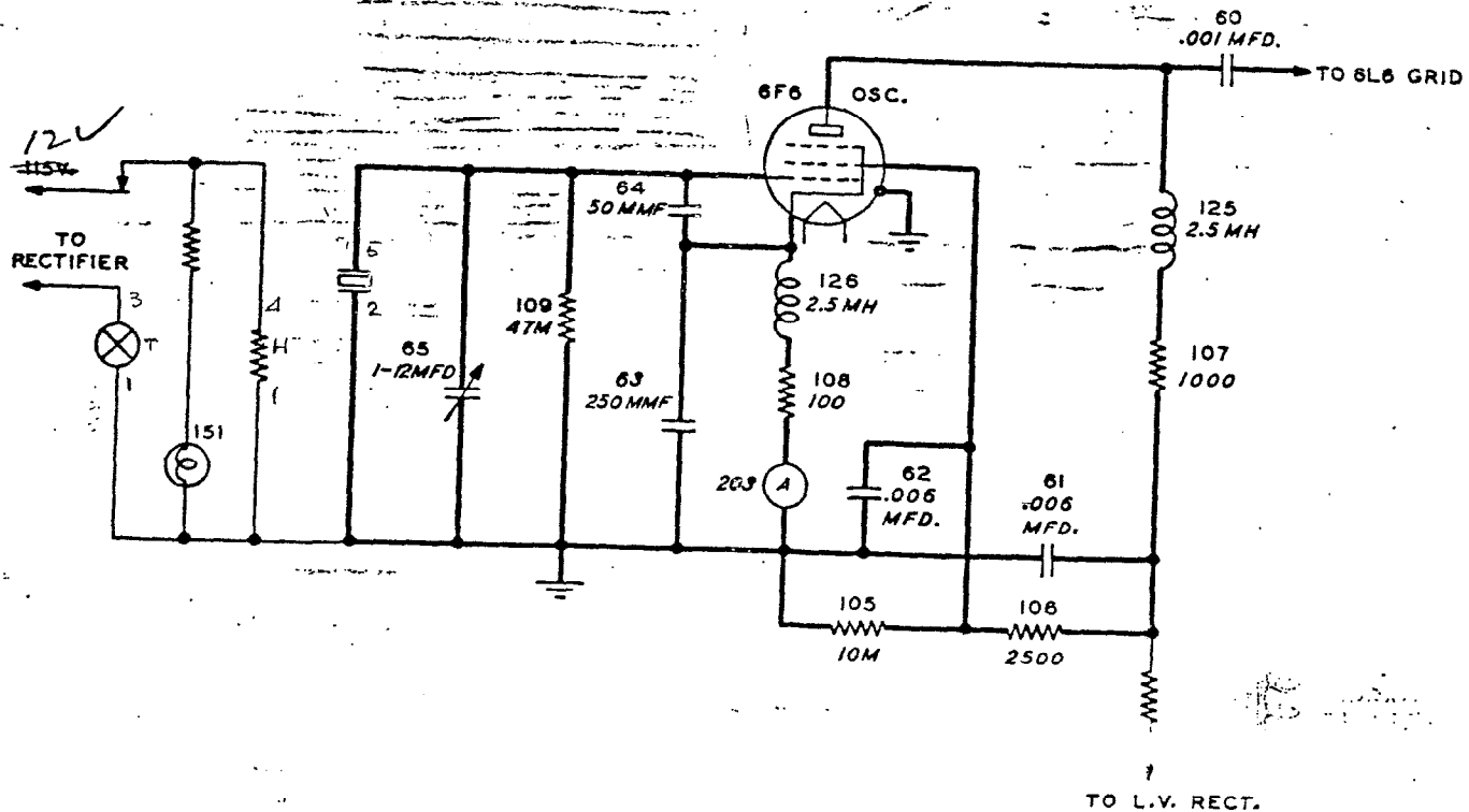
Figure 2-9. Oscillator Schematic
