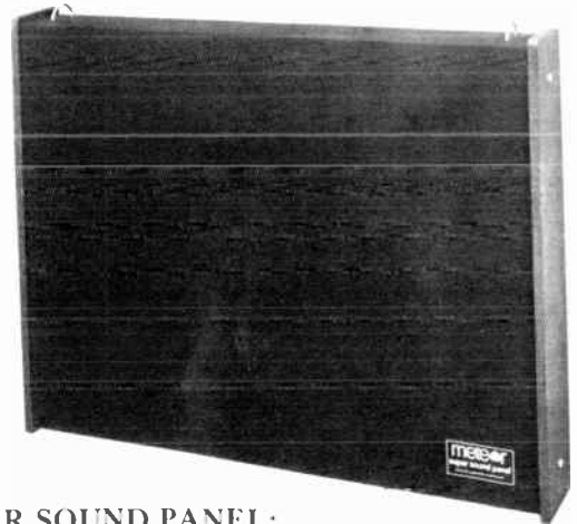
SUPER SOUND PANEL: A 4' x 3' x 5 3/4" deep speaker cabinet consisting of six 12" bass drivers, 4 mid speakers & 1 horn. CAPABLE OF 300 RMS.
