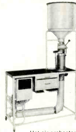
Hot-air preheater
