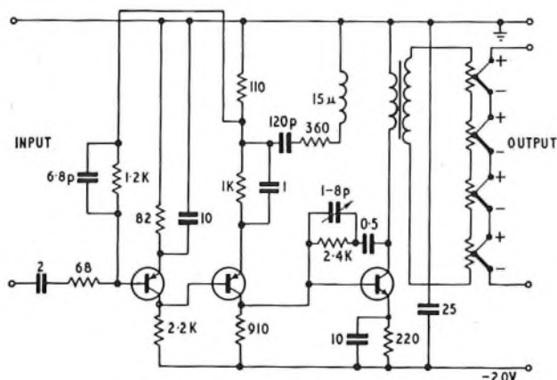
FIG. 5—ONE-SECOND-CHANNEL AMPLIFIER
