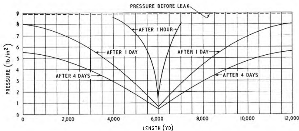
FIG. 4—FALL OF PRESSURE DUE TO LEAK IN STATIC-PRESSURE SYSTEM
