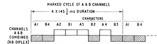
(c) Combination of (a) and (b) to Form a 2-Channel Character-Interleaved Aggregate Signal (Note that Character A1 is followed by Character B4, and so on.)
