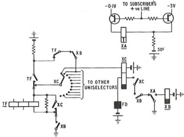
FIG. 6—PULSING AND TESTING CIRCUIT ELEMENT
