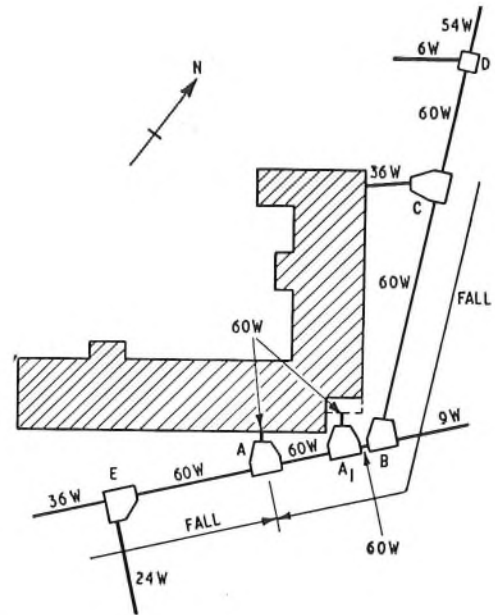
PLAN OF THE DUCT-WAYS, MANHOLES, AND EXCHANGE LEAD-IN AT SHEFFIELD CENTRAL
