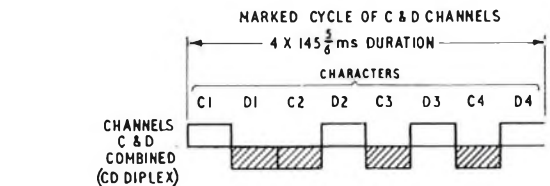
(d) Combination of Characters C2, C3 and C4 Inverted on Channel C and Character D1 Inverted on Channel D to Form a 2-Channel Signal (Note that Character C1 is followed by D1.)
