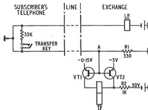
FIG. 1—BASIC CIRCUIT FOR OPERATION OF TRANSFER RELAY
