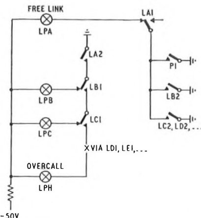
FIG. 5—FREE-LINK-SIGNALLING CIRCUIT ELEMENT
