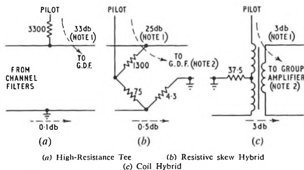
FIG. 2—METHODS OF INJECTING THE PILOT SIGNAL
