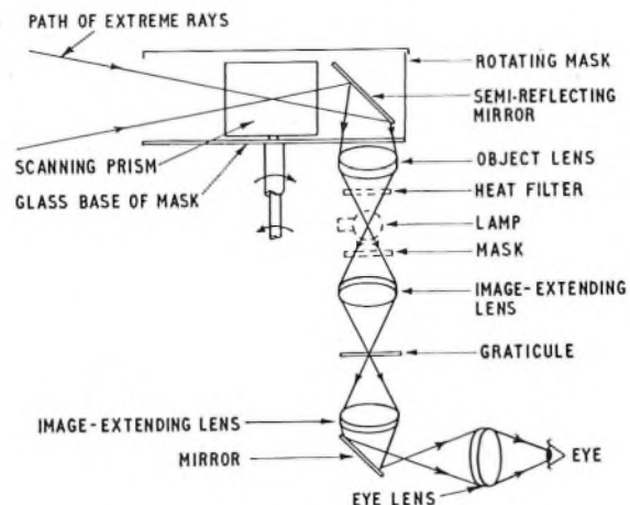
FIG. 5—PRINCIPLE OF OPTICAL SYSTEM
