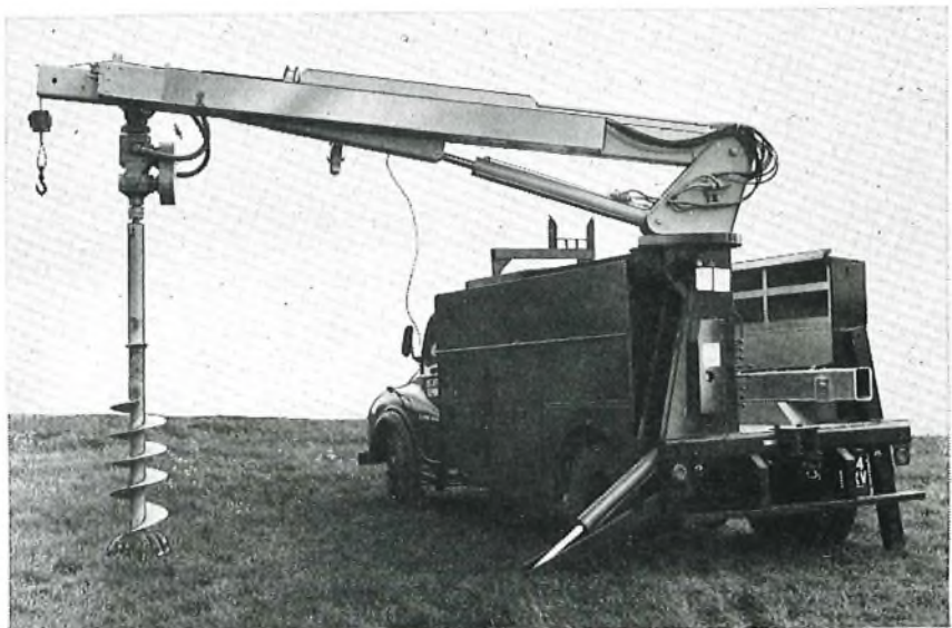
FIG. 3—POLE-HOLE BORER AND VEHICLE STABILIZERS
