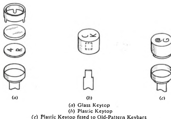
(a) Glass Keytop (b) Plastic Keytop (c) Plastic Keytop fitted to Old-Pattern Keybars FIG. 5—ATTACHMENT OF KEYTOPS TO KEYBARS
