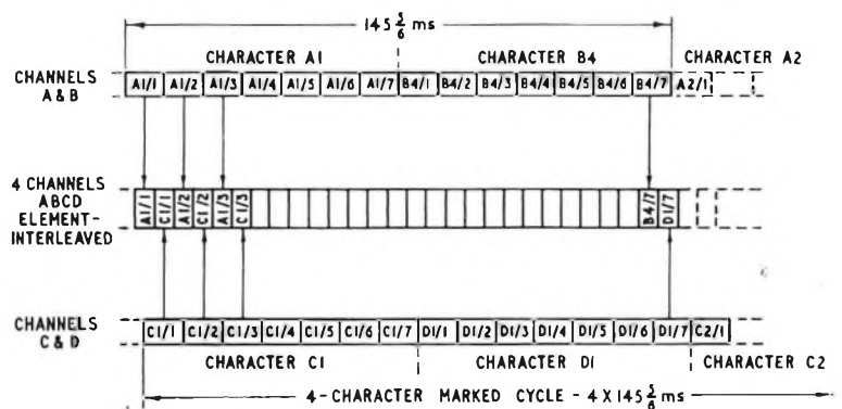
(e) Combination of Channels A, B, C and D to Form a 4-Channel Aggregate Signal. Channels A and B are Interleaved Element by Element with Channels C and D so that the First Element A1/1 of Characters A1 is followed by the First Element C1/1 of Character C1, and so on.
