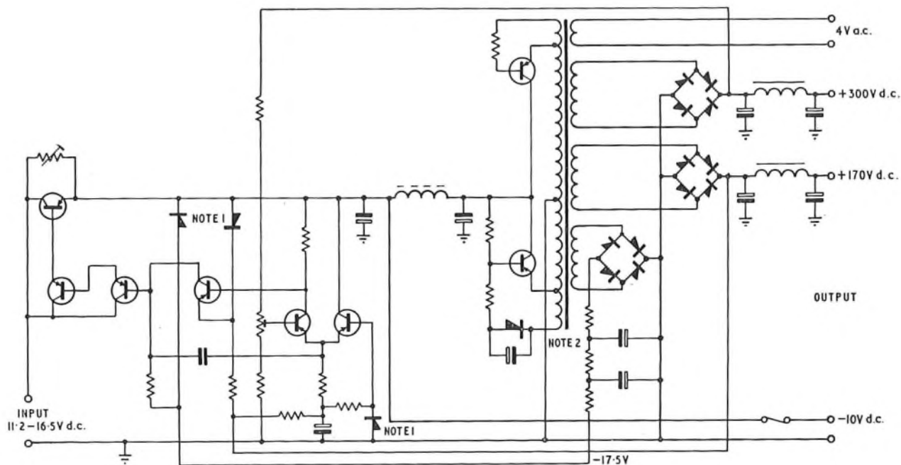
Notes: 1. Zener diodes. 2. Saturated low-hysteresis transformer.
