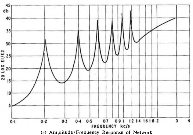
FIG. 4—FIVE-MILLISECOND INTEGRATING NETWORK
