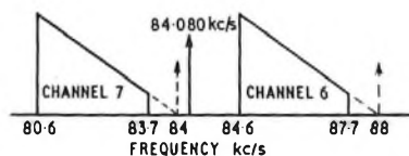
FIG. 1—POSITION OF THE PILOT-SIGNAL FREQUENCY WITHIN THE GROUP SPECTRUM
