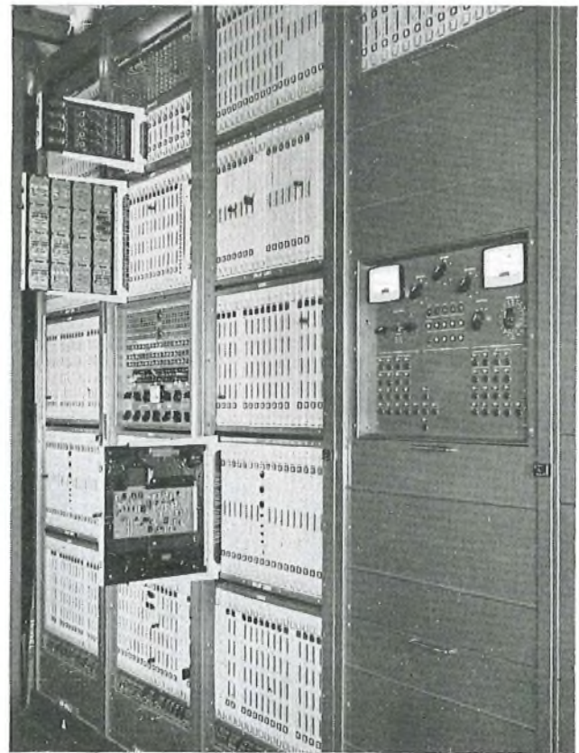
FIG. 13—REGISTER RACKS
