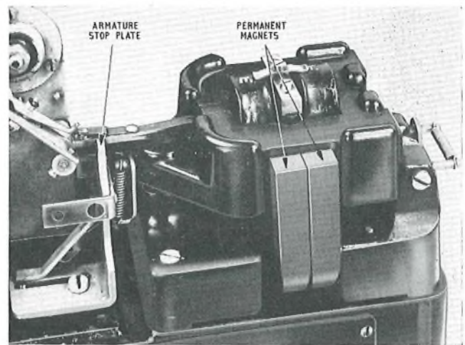
(a) Old-type Electromagnet and Stop-Plate
