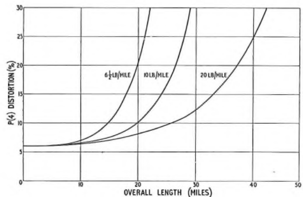
The graph shows the relationship of the P(4) value of start-stop telegraph distortion and the overall length of two interconnected telex subscribers' lines, the two lines being of equal length
