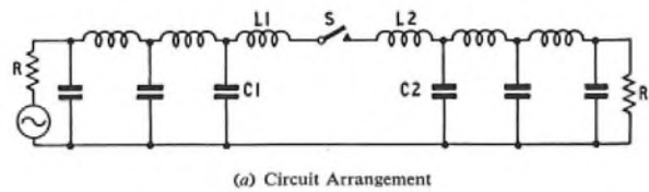
(a) Circuit Arrangement
