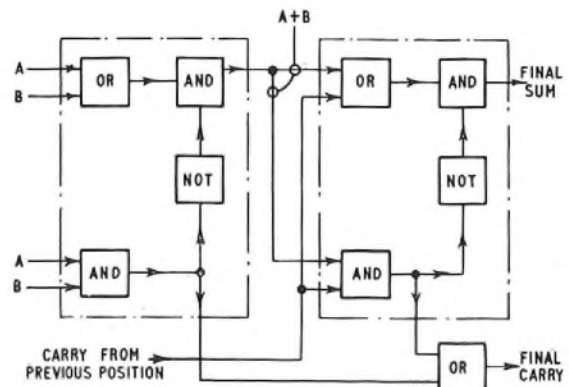
FIG. 4—TWO HALF-ADDEES
