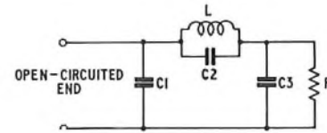
FIG. 9—CONFIGURATION OF A 4-ELEMENT FILTER
