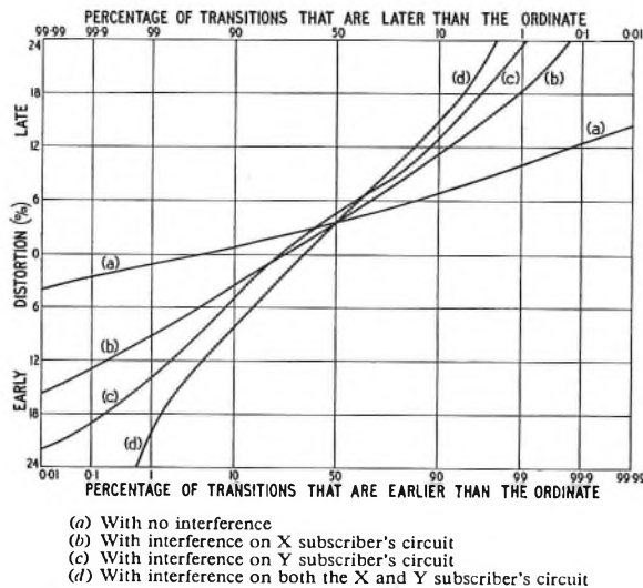
Each of the two lines consisted of an artificial cable equivalent to 25 miles of 20 lb/mile conductor
