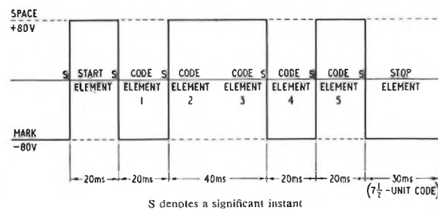
FIG. 1—ELEMENTS OF TELEGRAPH-CHARACTER SIGNAL
