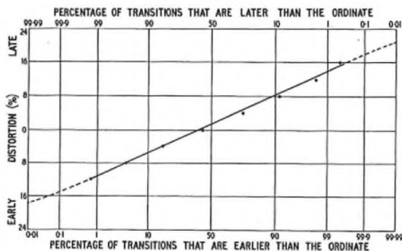
Each of the two lines was 20 miles long and consisted of 20 lb/mile conductors FIG. 2—DISTORTION MEASURED OVER TWO INTERCONNECTED TELEX SUBSCRIBERS' LINES
