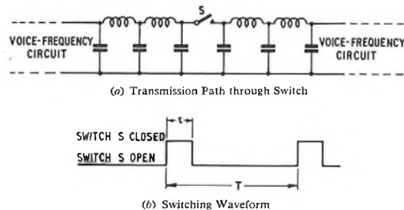
FIG. 1—PRINCIPLE OF THE BOTHWAY GATE
