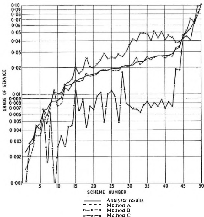
FIG. 9—GRADE OF SERVICE FOR VARIOUS SCHEMES OF ALTERNATIVE ROUTING
