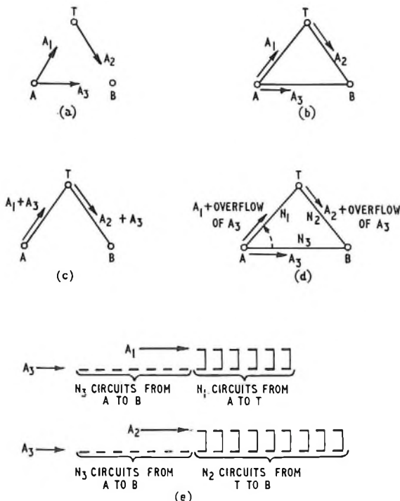
FIG. 8—ALTERNATIVE ROUTING
