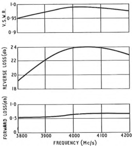
FIG. 8.—PERFORMANCE
