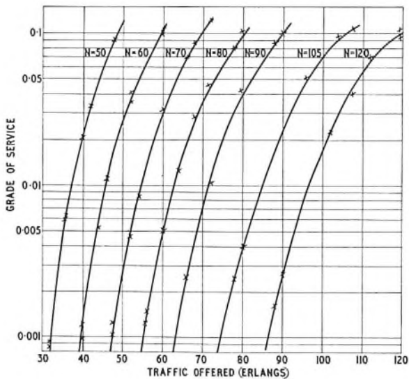
N = Number of trunks × Denotes analyser results FIG. 5—VARIATION OF GRADE OF SERVICE WITH TRAFFIC OFFERED FOR 40-AVAILABILITY GRADINGS
