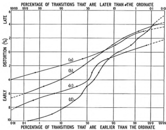
FIG. 9—DISTORTION INTRODUCED BY TELEGRAPH TRANSMITTERS
