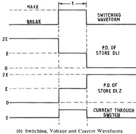
FIG. 4—BOTHWAY GATE EMPLOYING DELAY LINES—INTERCHANGE OF CHARGES
