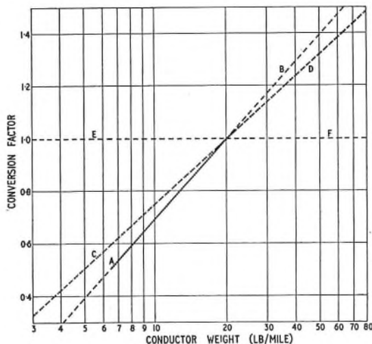
AB = conversion factor when P(4) = 25% CD = conversion factor when P(4) = 10% EF = conversion factor when P(4) = 6%
