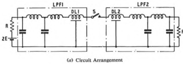
(a) Circuit Arrangement
