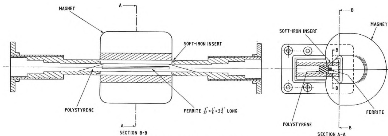
FIG. 5—MECHANICAL ARRANGEMENT
