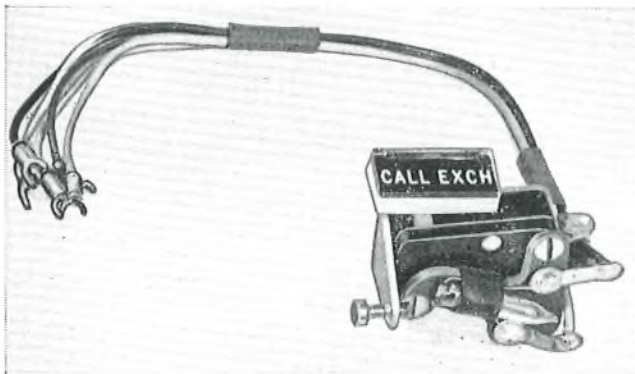
FIG. 15—SHARED-SERVICE ADAPTOR
