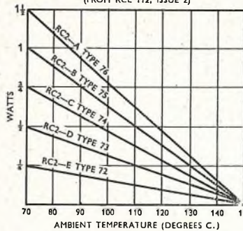
WATTAGE RATING/AMBIENT TEMPERATURE GRAPH (FROM RCL 112, ISSUE 2)
