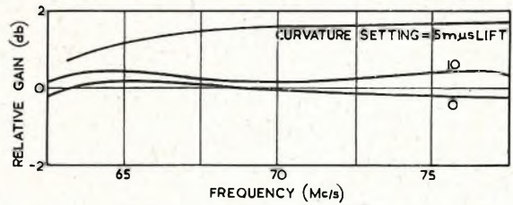
FIG. 5.—AMPLITUDE TRANSMISSION CHARACTERISTICS.
