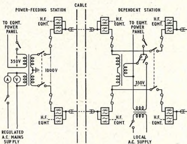
FIG. 5.—POWER-FEEDING CIRCUIT.
