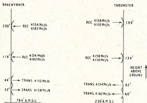
FIG. 10.—AERIAL HEIGHTS.
