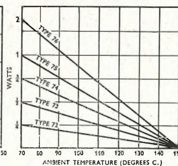
COMMERCIAL DERATING CURVE
