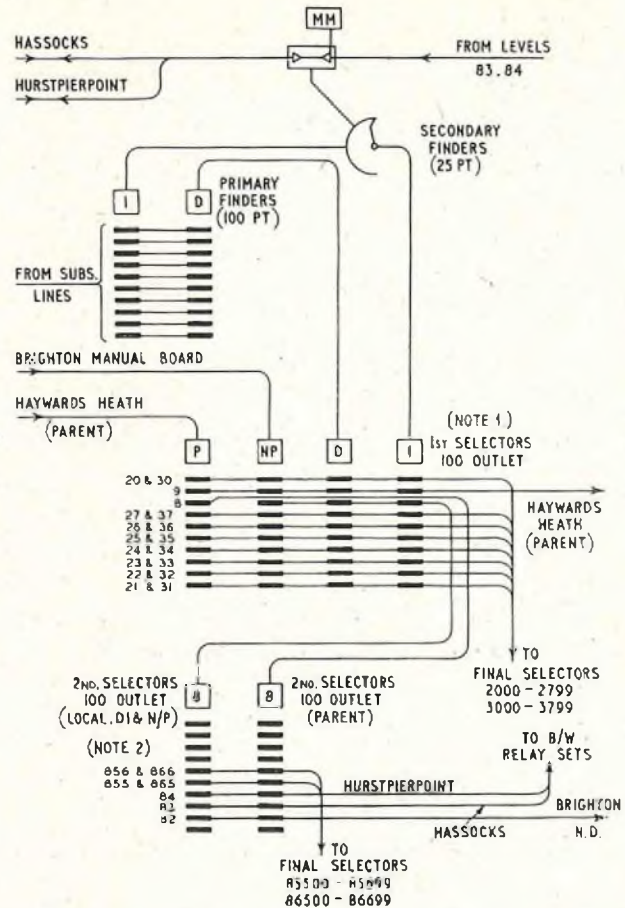
TRUNKING DIAGRAM. BURGESS HILL U.A.X. No. 7.
