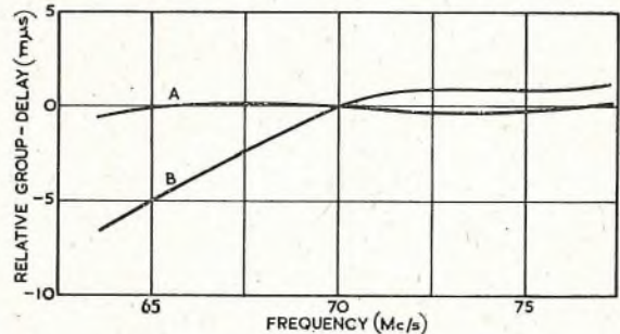
Curve A: Zero slope, zero curvature. Curve B: Slope + 1.0 \mu\text{s}/\text{Mc}/\text{s} . Curvature 3 \mu\text{s} lift.
