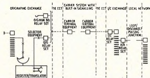
FIG. 4.—ROUTING ARRANGEMENTS.
