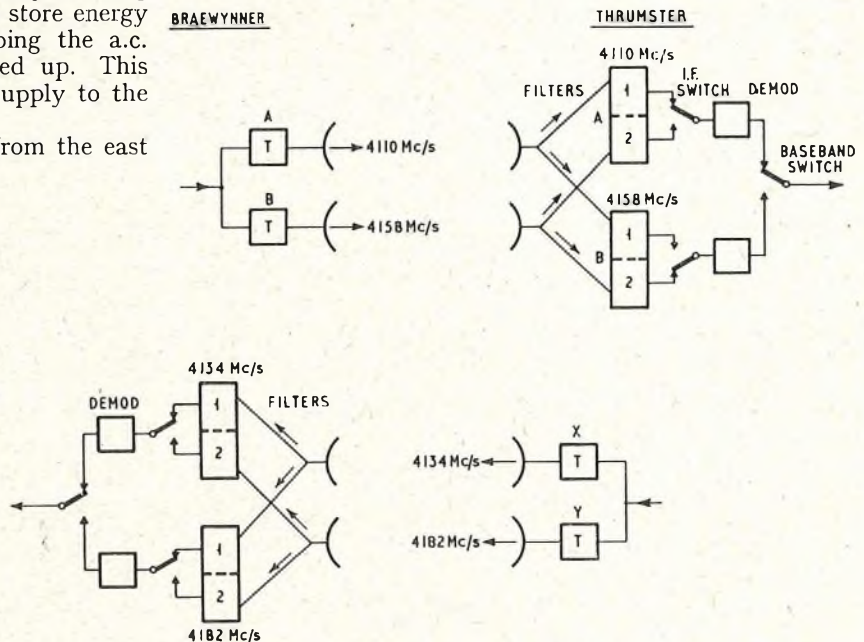
FIG. 6.—SIMPLIFIED BLOCK SCHEMATIC DIAGRAM OF RADIO EQUIPMENT.
