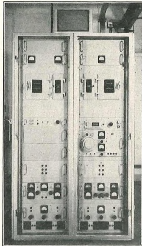
FIG. 14.—FRONT VIEW OF TRANSMITTER WITH DOORS REMOVED.
