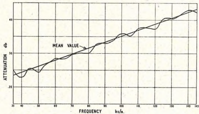
ATTENUATION/FREQUENCY CHARACTERISTIC.
