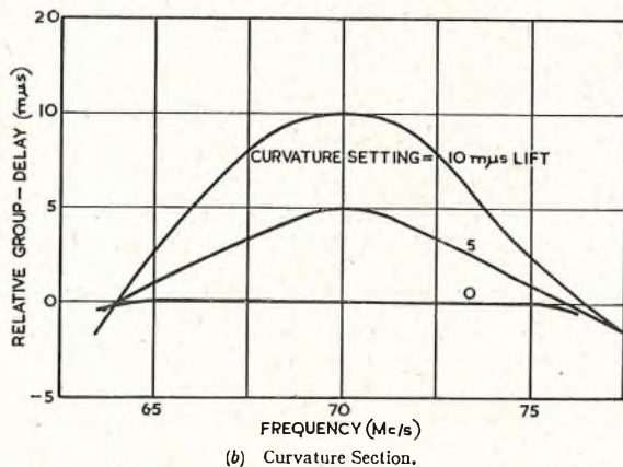
FIG. 4.—GROUP-DELAY TRANSMISSION CHARACTERISTICS.
