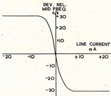
FIG. 5.—MODULATOR CHARACTERISTIC.
