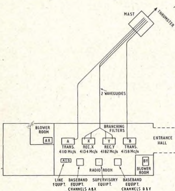
FIG. 12.—LAYOUT OF MAST, WAVEGUIDE RUNS AND BUILDING AT BRAEVYNNER.
