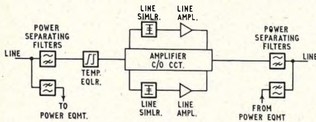
One h.f. channel only is shown; the other is identical.
