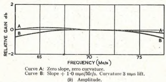
FIG. 6.—TYPICAL OVERALL TRANSMISSION CHARACTERISTICS.
