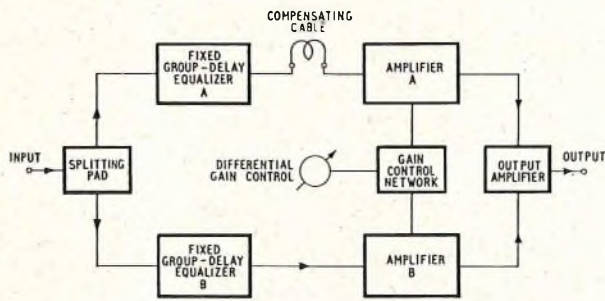
FIG. 3.—BLOCK SCHEMATIC DIAGRAM OF BASIC CIRCUIT.
