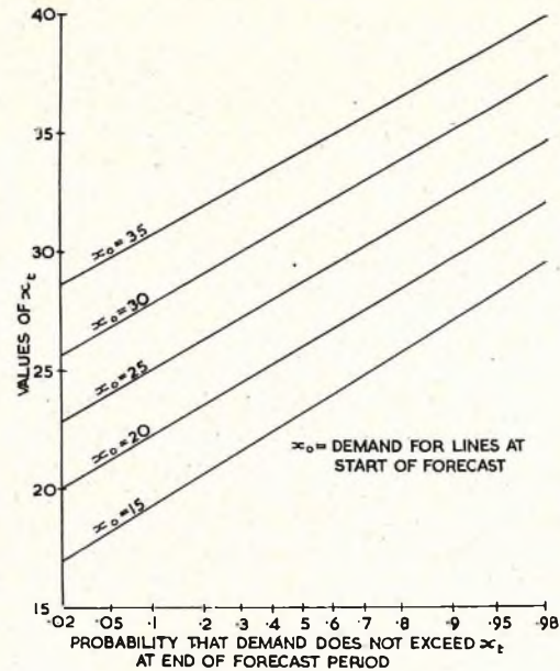
FIG. 4.—FORECASTING CHART FOR DISTRIBUTION AREA.
