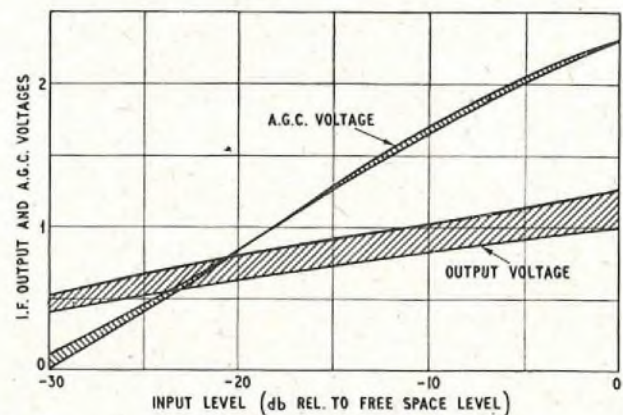
FIG. 22.—RECEIVER TRACKING.
