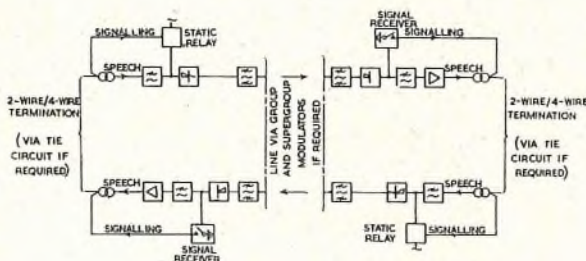
FIG. 1.—BASIC PRINCIPLES OF OUT-BAND SIGNALLING.
