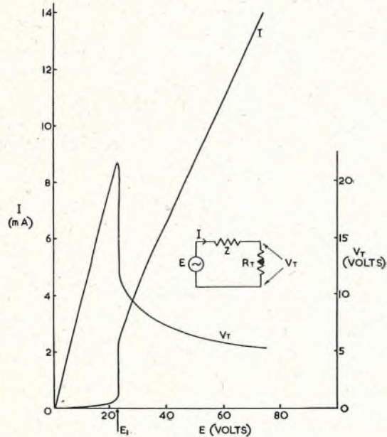
FIG. 6.—VOLTAGE AND CURRENT CONDITIONS IN A THERMISTOR CIRCUIT AT 20°C.
