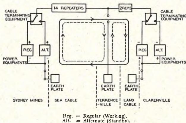
FIG. 2.—CURRENT PATHS ON CLARENVILLE-SYDNEY MINES LINK.
