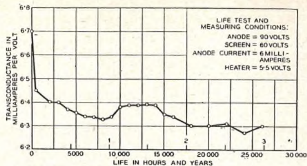
FIG. 13.—BEHAVIOUR OF A GROUP OF 92 6P12 VALVES OVER A PERIOD OF THREE YEARS.
