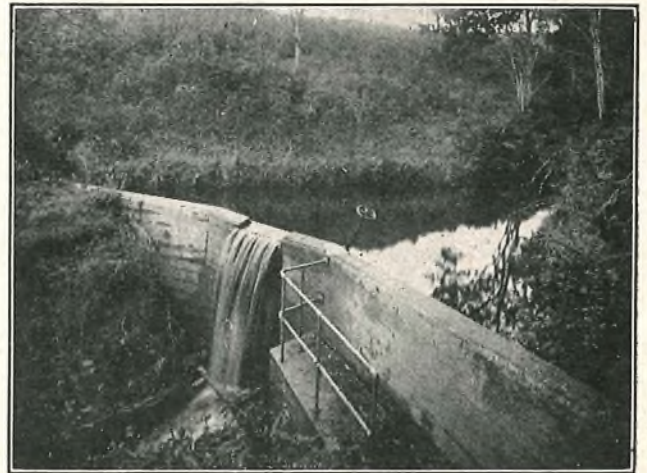
FIG. 17.—POND USED FOR ENGINE-COOLING WATER.
