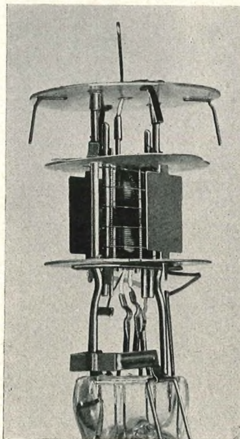
FIG. 14.—INTERIOR OF A 6P12 TYPE VALVE.
