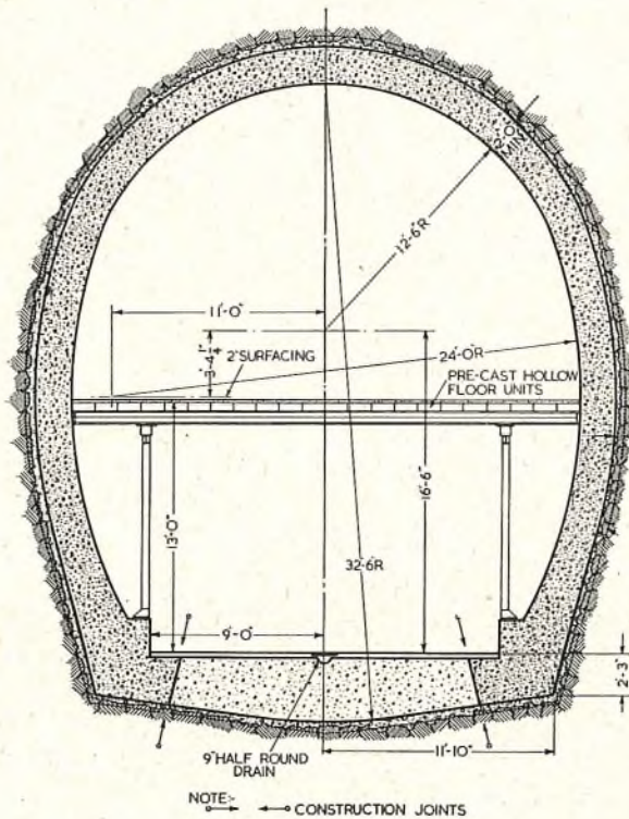
FIG. 5.—CROSS-SECTION OF TUNNEL.
