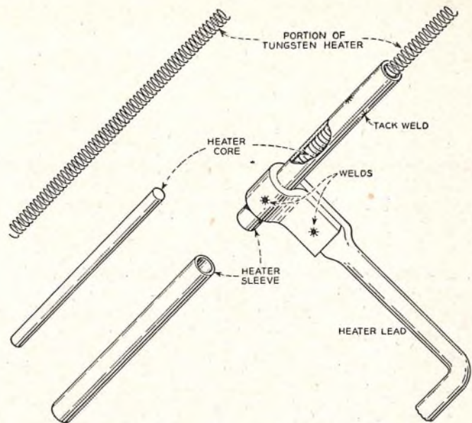
FIG. 4.—HEATER CONNEXION OF THE 175HQ VALVE.
