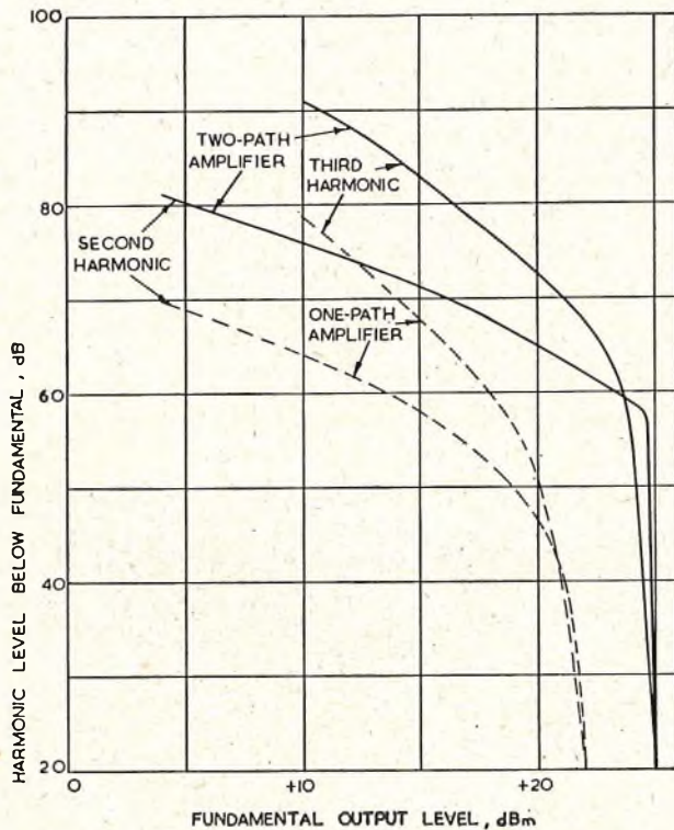
FIG. 14.—AMPLIFIER DISTORTION.
