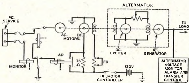
FIG. 4.—TWO-MOTOR ALTERNATOR SET.
