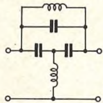
FIG. 12.—SCHEMATIC DIAGRAM OF DELAY EQUALIZER SECTION.
