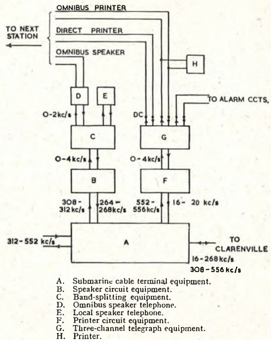
FIG. 11.—ARRANGEMENT OF SPEAKER AND PRINTER EQUIPMENT AT SYDNEY MINES.
