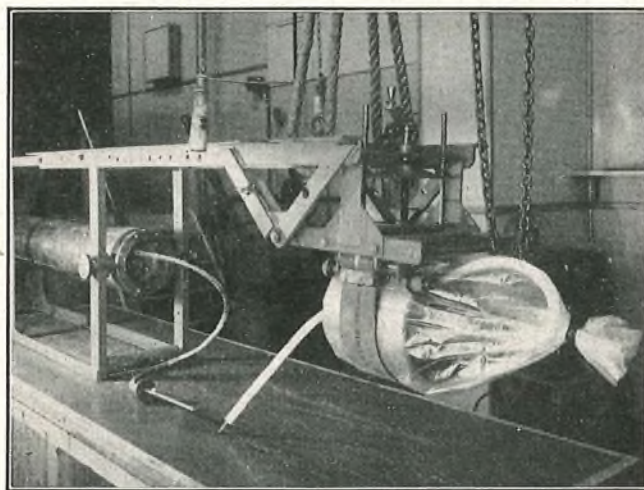
FIG. 6.—ELECTRICAL UNIT AND BULKHEAD, WITH CABLE ENDS READY FOR JOINTING.
