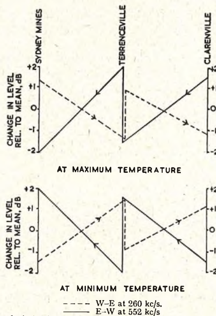
FIG. 10.—DEVIATION FROM MEAN OF TRANSMISSION LEVELS WITH OPTIMUM ADJUSTMENTS OF EQUALIZERS AT SYDNEY MINES, TERRENCEVILLE AND CLARENVILLE.
