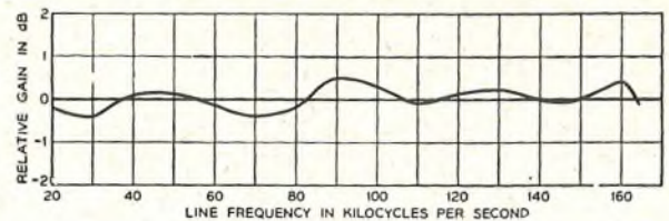
FIG. 12.—GAIN/LINE-FREQUENCY: NO. 1 CABLE.
