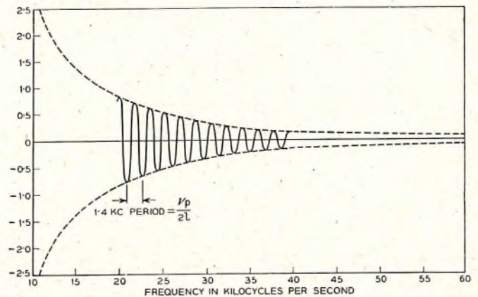
FIG. 20.—INTERACTION RIPPLE FOR THE SYSTEM.
