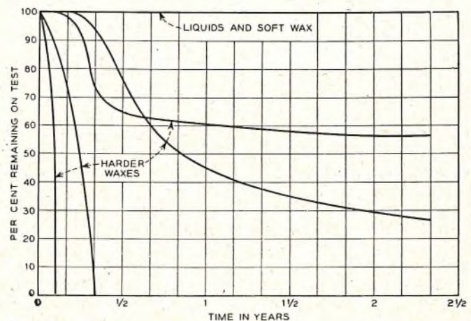
FIG. 12.—ACCELERATED LIFE TESTS ON PAPER CAPACITORS WITH VARIOUS IMPREGNANTS AT ROOM TEMPERATURE (60°-80°F).
