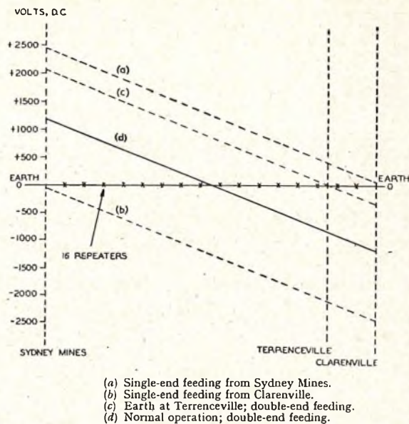
FIG. 3.—POTENTIAL DISTRIBUTION ON CLARENVILLE-SYDNEY MINES LINK.
