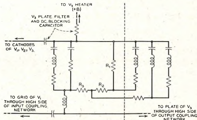
FIG. 8.—BETA NETWORK.
