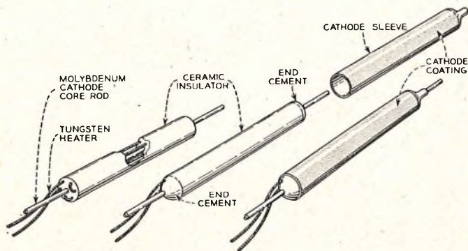
FIG. 3.—HEATER, HEATER INSULATOR AND CATHODE ASSEMBLY OF THE 175HQ VALVE.
