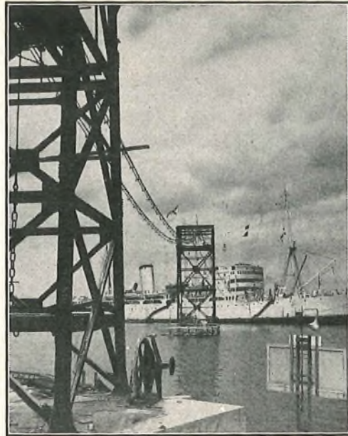
FIG. 3.—CABLE TOWERS, USED FOR LOADING CABLE INTO THE SHIP
