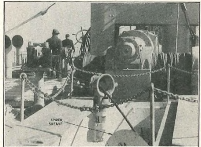
FIG. 8.—FORMER SPIDER SHEAVE AT CABLE TANK NO. 1.
