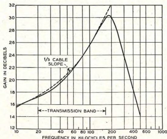
FIG. 6.—GAIN OF INPUT COUPLING NETWORK.
