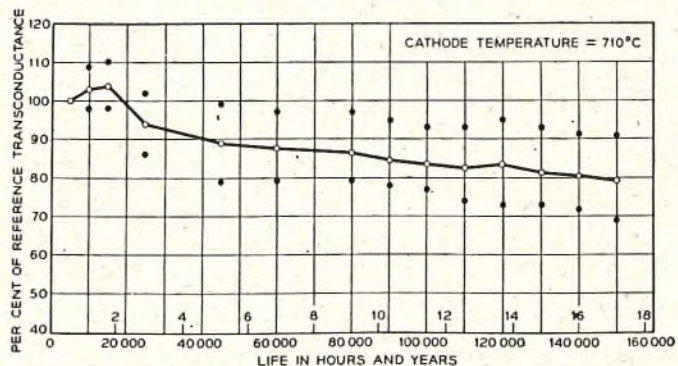
FIG. 7.—RESULTS OF LIFE TESTS ON SIXTEEN 175HQ VALVES OPERATING AT A CATHODE TEMPERATURE OF 710^\circ\text{C} .
