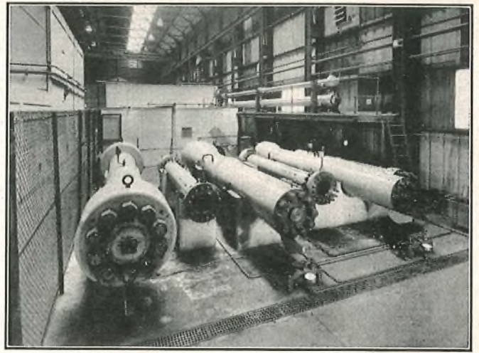
FIG. 9.—PRESSURE-TESTING EQUIPMENT.
