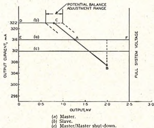
FIG. 1.—OUTPUT-CURRENT/OUTPUT-VOLTAGE CHARACTERISTICS.
