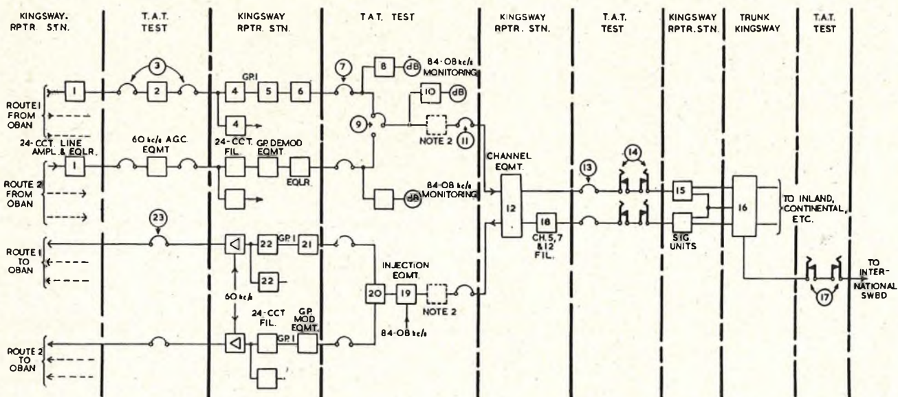
FIG. 18.—ARRANGEMENT OF CARRIER CIRCUIT IN LONDON FOR THE T.A.T. CABLE SYSTEM.
