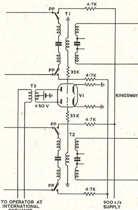
FIG. 8.—MONITORING AND 3-MINUTE TONE CIRCUIT ELEMENT.
