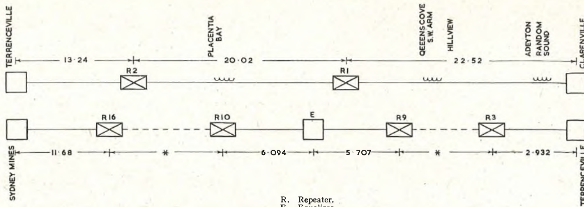
R. Repeater. E. Equalizer. All distances are in nautical miles. * Repeater spacing R3-R9 and R10-R16, 20.4 n.m. FIG. 2.—STRAIGHT-LINE DIAGRAM OF ROUTE.
