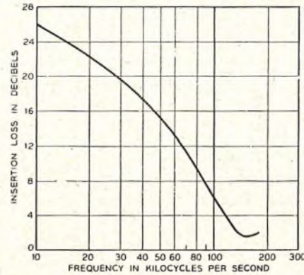
FIG. 6.—TRANSMITTING EQUALIZER: LOSS/FREQUENCY CHARACTERISTIC.
