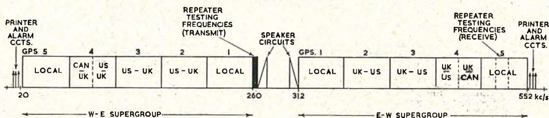
FIG. 5.—FREQUENCY ALLOCATION.
