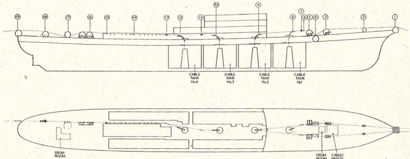
FIG. 1.—LAYOUT OF CABLE MACHINERY IN H.M.T.S. "MONARCH."
