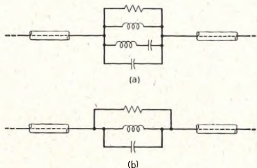
(a) Schematic of Type IV equalizer. (b) Schematic of Type V equalizer.
