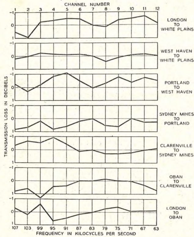
FIG. 5.—FREQUENCY CHARACTERISTIC OF TYPICAL LONDON-NEW YORK GROUP.
