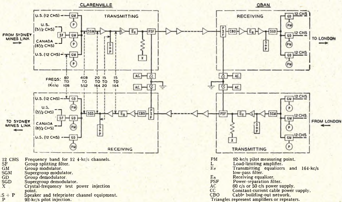
FIG. 2.—NORTH ATLANTIC LINK: BLOCK SCHEMATIC DIAGRAM.
