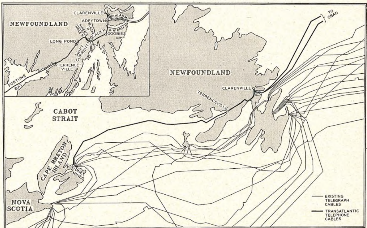
FIG. 3.—CABLE LANDINGS ON NEWFOUNDLAND, AND THE FINAL ROUTE OF THE OVERLAND SECTION OF THE CLARENVILLE-SYDNEY MINES CABLE.
