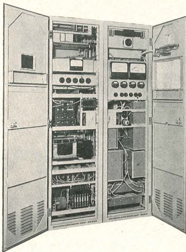
FIG. 7.—POWER EQUIPMENT.
