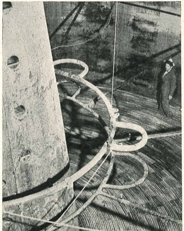
FIG. 7.—INTERIOR OF CABLE TANK, SHOWING CENTRAL CONE, CRINOLINE, AND A "FLAKE" OF CABLE.
