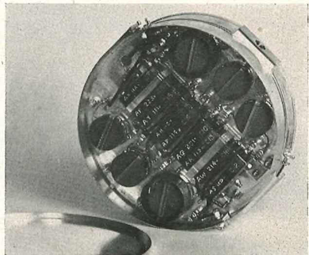
High-pass filter with low-pass filter can on rear.
