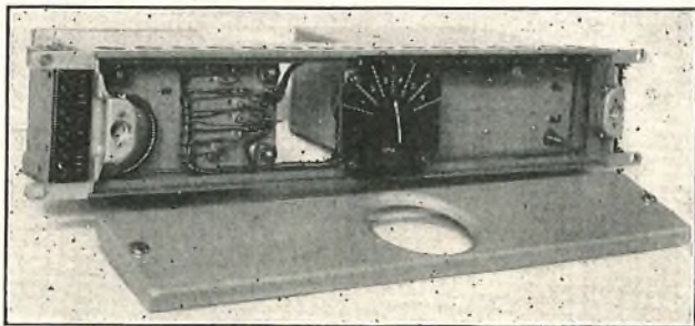
FIG. 1.—24-CIRCUIT TEMPERATURE AND RESIDUAL EQUALIZERS.
