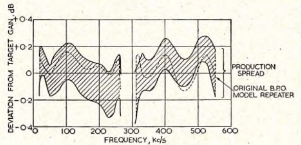
FIG. 17.—REPEATER-GAIN RESPONSE.
