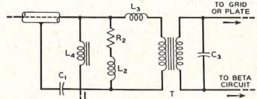
FIG. 4.—COUPLING NETWORK.
