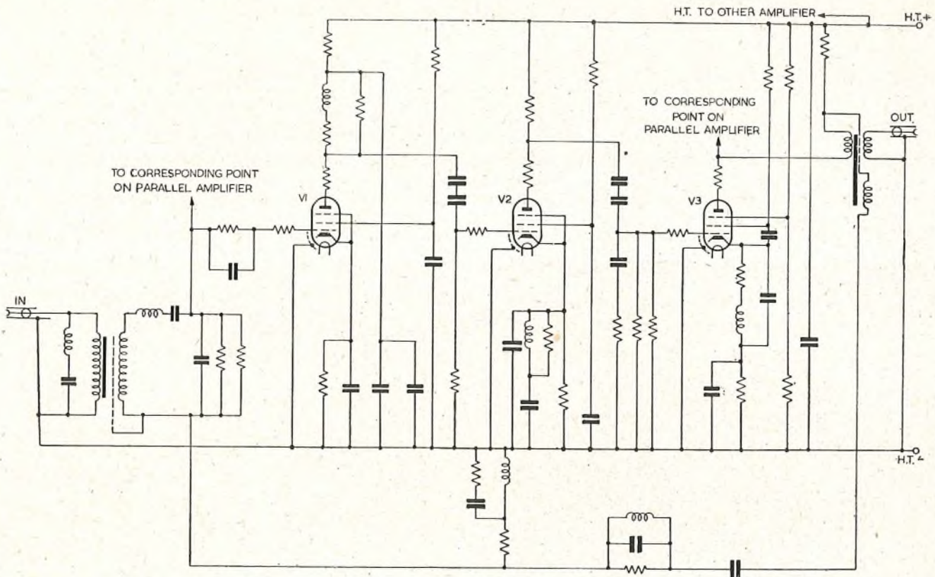
FIG. 3.—AMPLIFIER CIRCUIT.
