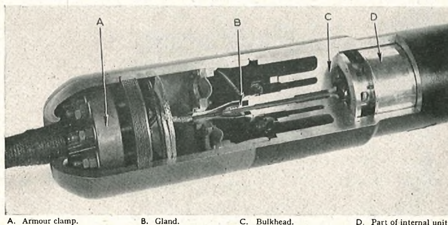
FIG. 8.—DETAILS OF HOUSING CONSTRUCTION.
