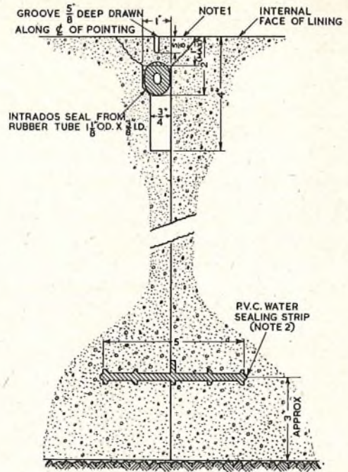
FIG. 6.—DETAILS OF CONSTRUCTION JOINT.
