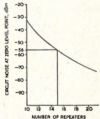
FIG. 8.—VARIATION OF CIRCUIT NOISE WITH NUMBER OF REPEATERS.
