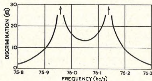
FIG. 10.—TYPICAL CHARACTERISTIC OF PEAK-SUPPRESSION FILTER.
