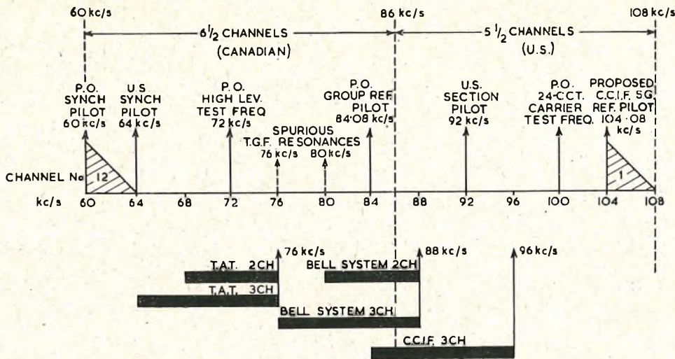
FIG. 6.—FREQUENCY ALLOCATION FOR MUSIC-IN-BAND CIRCUITS.
