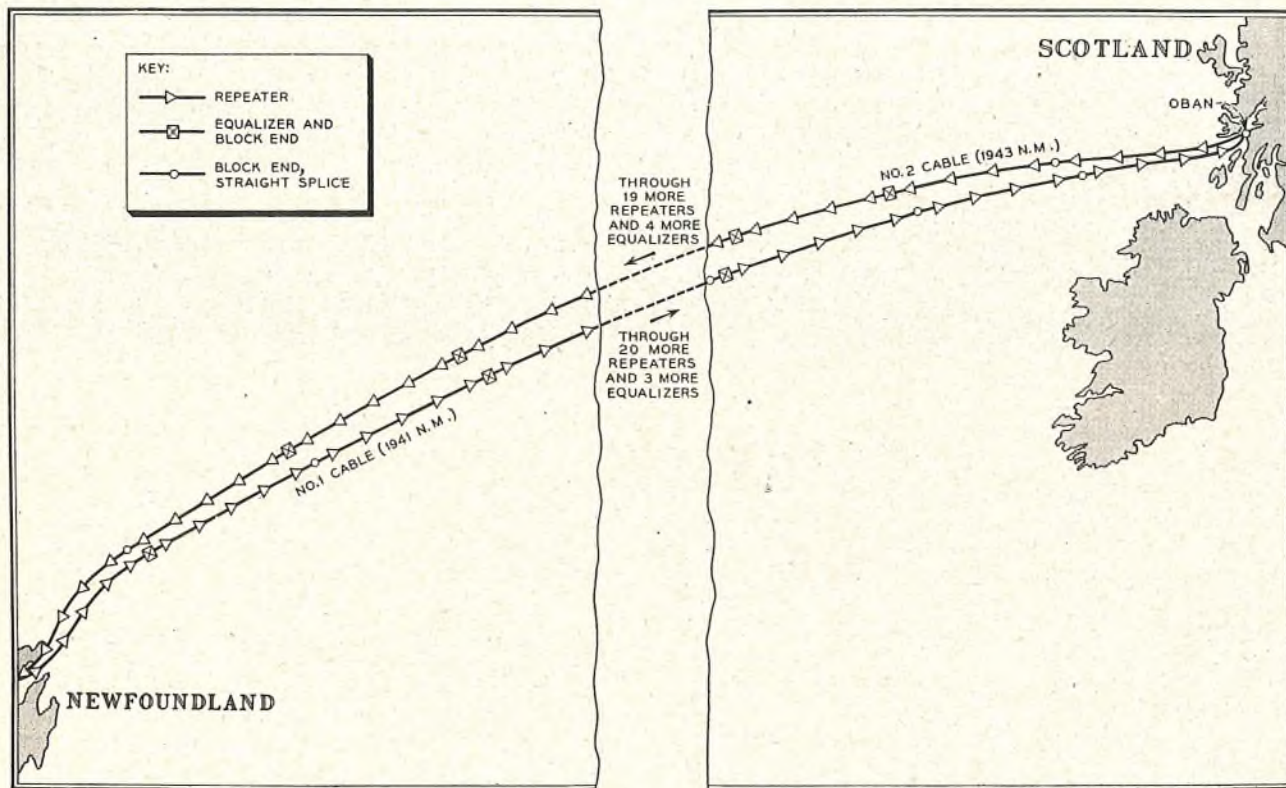
FIG. 4.—TRANSATLANTIC TELEPHONE CABLE ROUTES.
