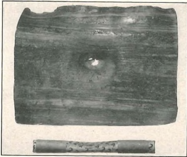
DAMAGED SHEATH REMOVED FROM COAXIAL CABLE, AND COAXIAL TUBE FLATTENED BY LIGHTNING DAMAGE.
