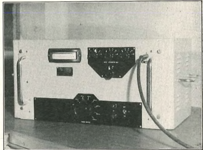
FIG. 8.—EXPERIMENTAL NOISE RECEIVER.
