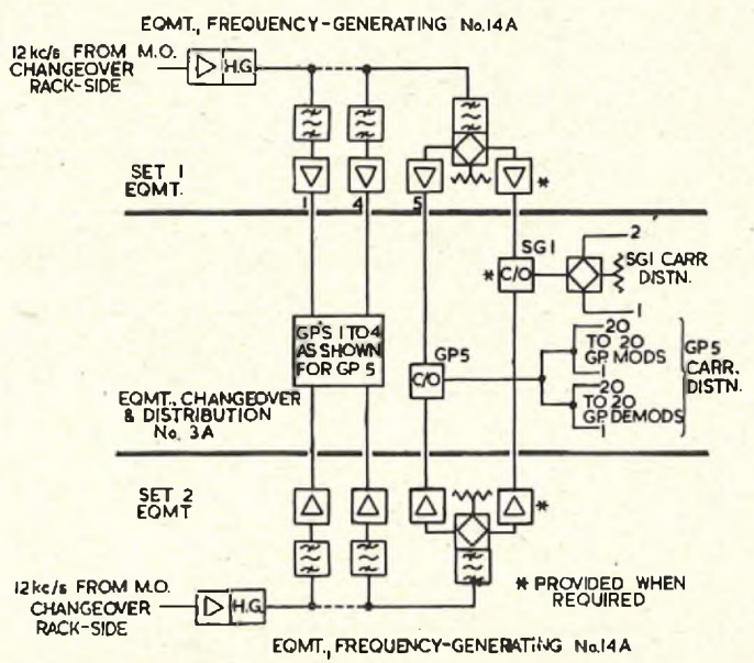
FIG. 4.—GROUP CARRIER GENERATING EQUIPMENT.
