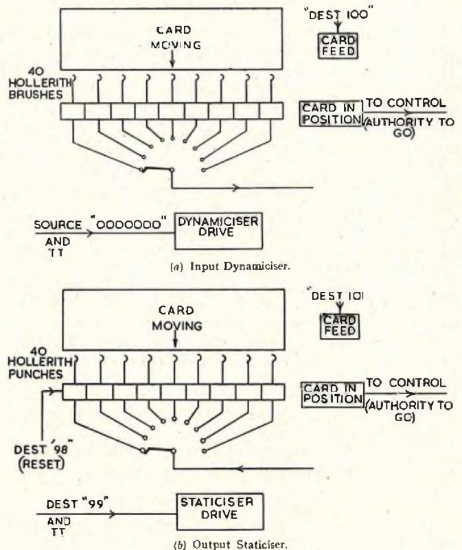
FIG. 8.—INPUT AND OUTPUT CONTROLS.
