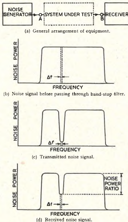
FIG. 1.—PRINCIPLE OF NOISE TESTING METHOD.
