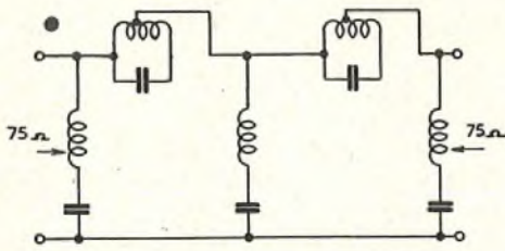
FIG. 6.—TYPICAL BAND-STOP FILTER.
