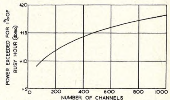
FIG. 2.—TRAFFIC LOADING.
