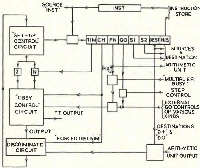
FIG. 5.—BLOCK SCHEMATIC DIAGRAM OF CONTROL CIRCUIT.
