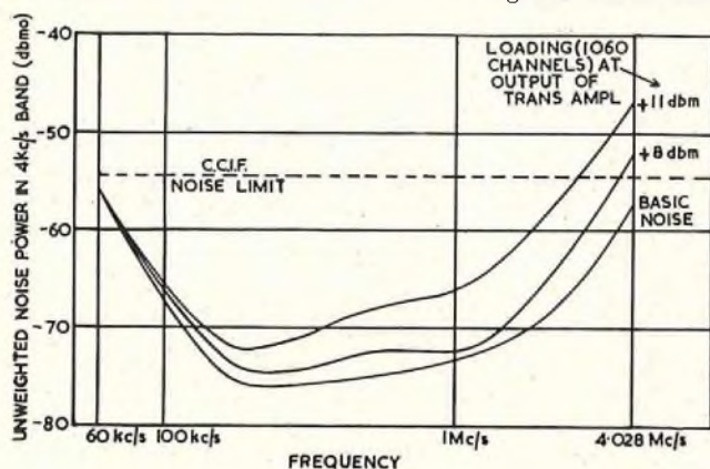
FIG. 10.—PERFORMANCE OF A 335-MILE COAXIAL-CABLE LINK.
