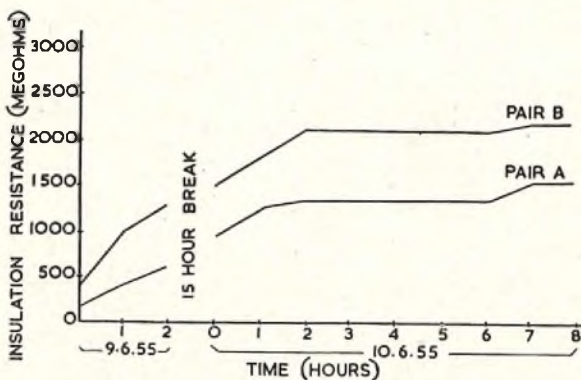
CHANGE IN INSULATION RESISTANCE OF TWO CABLE PAIRS DURING DESICCATION.
