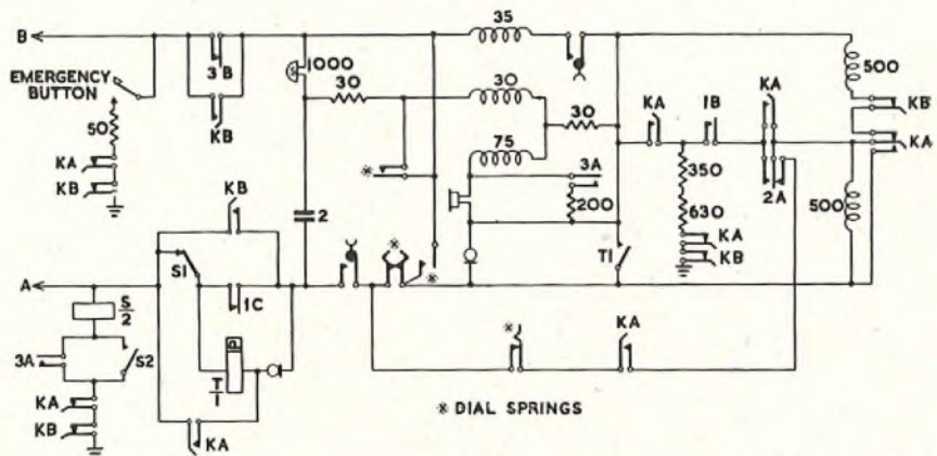
FIG. 5.—TELEPHONE CIRCUIT, INCLUDING KEYS MOUNTED ON THE KEY SWITCHING PANEL.
