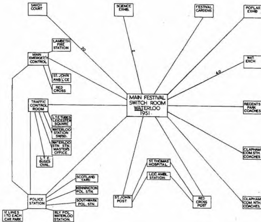
FIG. 1.—COMMUNICATION DIAGRAM.
