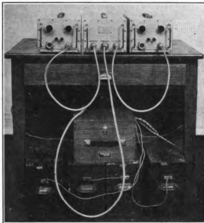
FIG. 2.—EQUIPMENT FOR A COMPLETE RADIO TERMINAL STATION.
