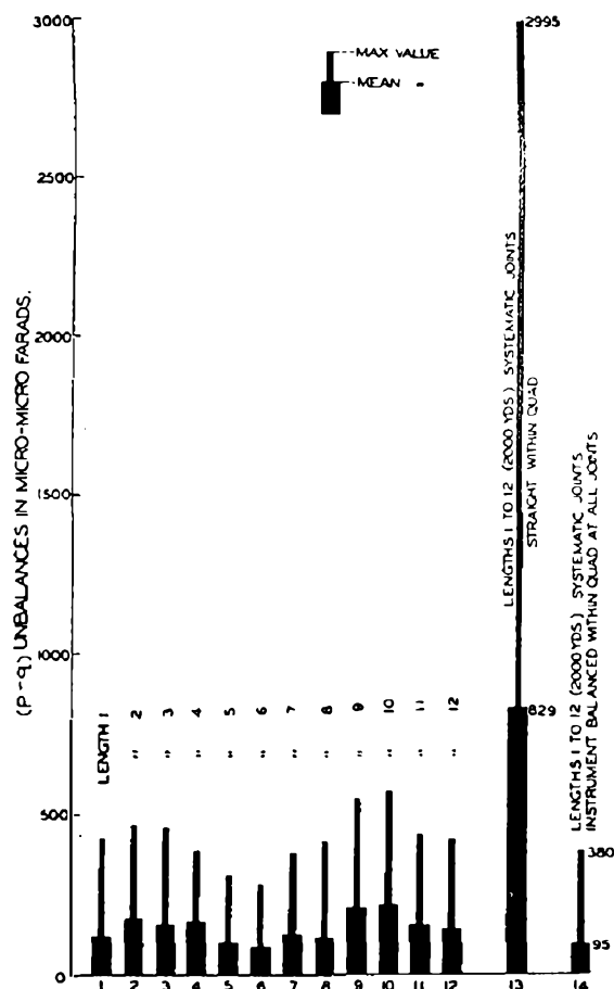
FIG. 1.—SIDE-TO-SIDE (p-q) UNBALANCES WITH AND WITHOUT USE OF INSTRUMENT. 100 PR. 20 LB. P.C.Q.L. CABLE.
