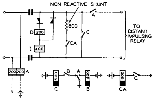
FIG. 2.—CIRCUIT ELEMENTS OF "TWO-STAGE DROP-BACK" FEATURE.
