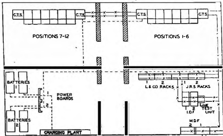
FIG. 2.—TYPICAL LAYOUT FOR 12-POSITION EXCHANGE.
