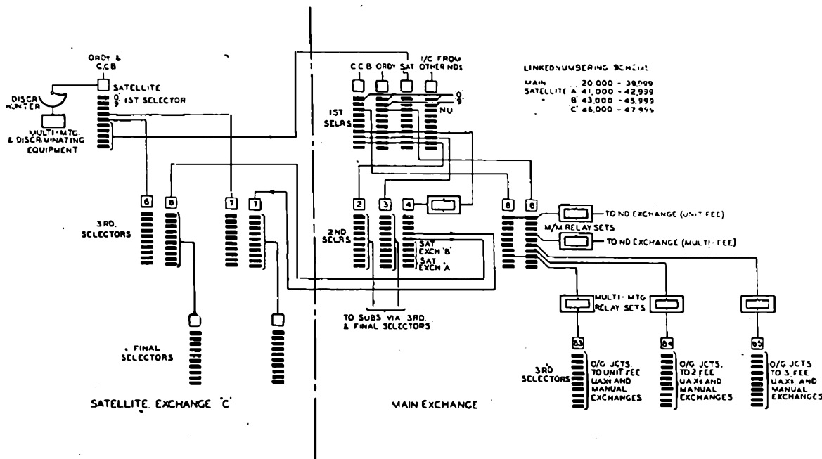
FIG. 1.—TYPICAL TRUNKING ARRANGEMENTS.
