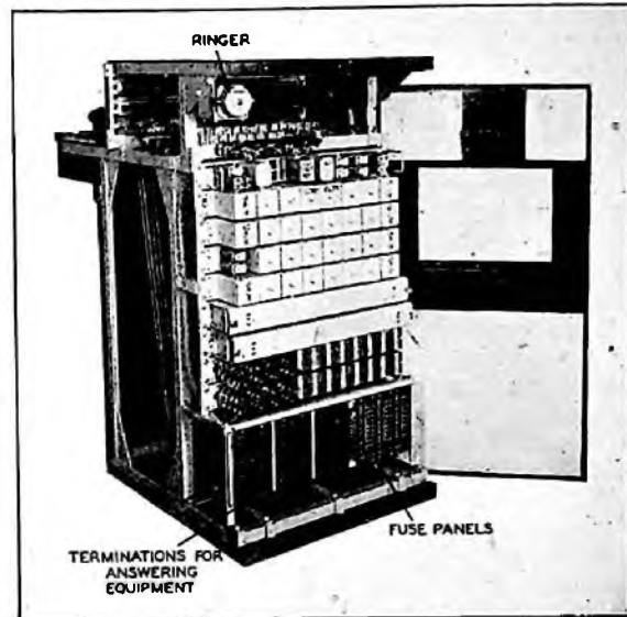
FIG. 3.—REAR OF SWITCH SECTION.
