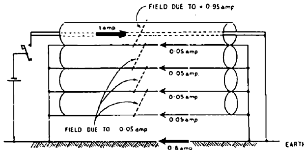
FIG. 1.—DIAGRAM ILLUSTRATING CURRENT FLOW.
