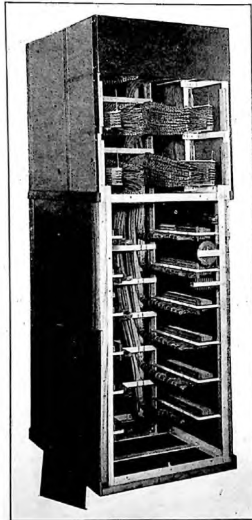
FIG. 5.—CABLE TERMINATING SECTION.
