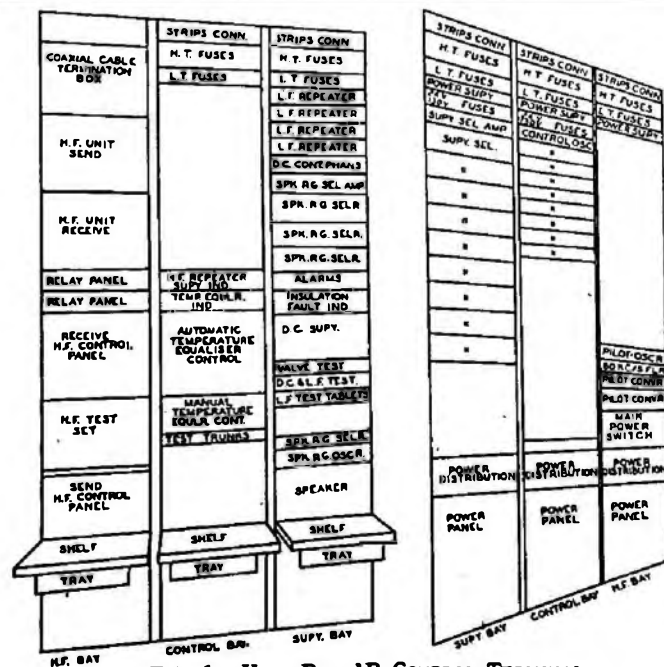
FIG. 1.—UNIT BAY IB CONTROL TERMINAL.
