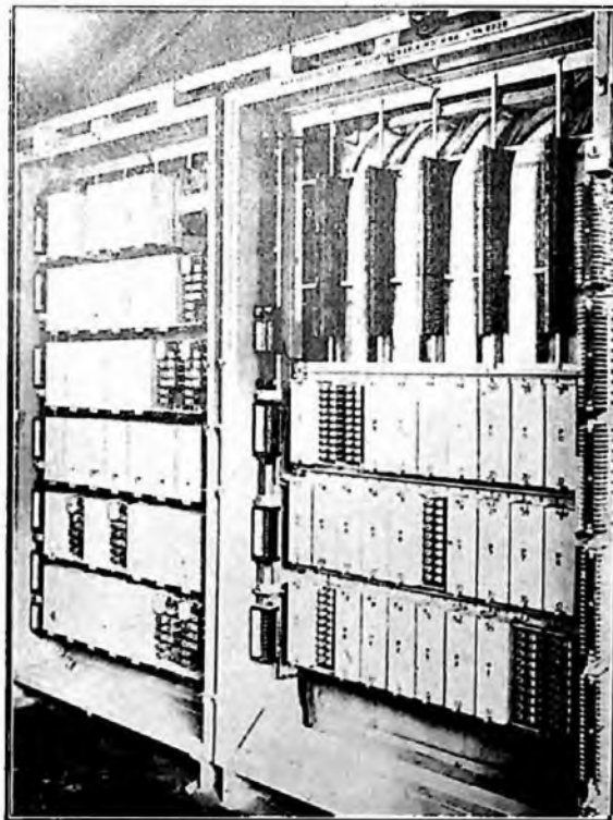
JUNCTION RELAY SET RACK. L AND K RELAY RACK. FIG. 6.—APPARATUS RACKS (COVERS REMOVED).
