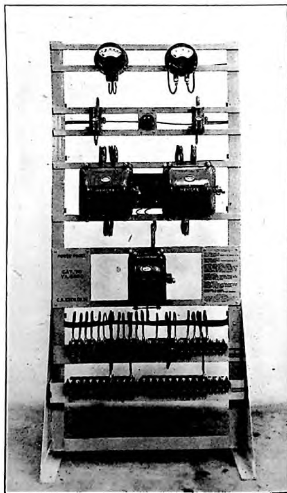
FIG. 8.—POWER BOARD.
