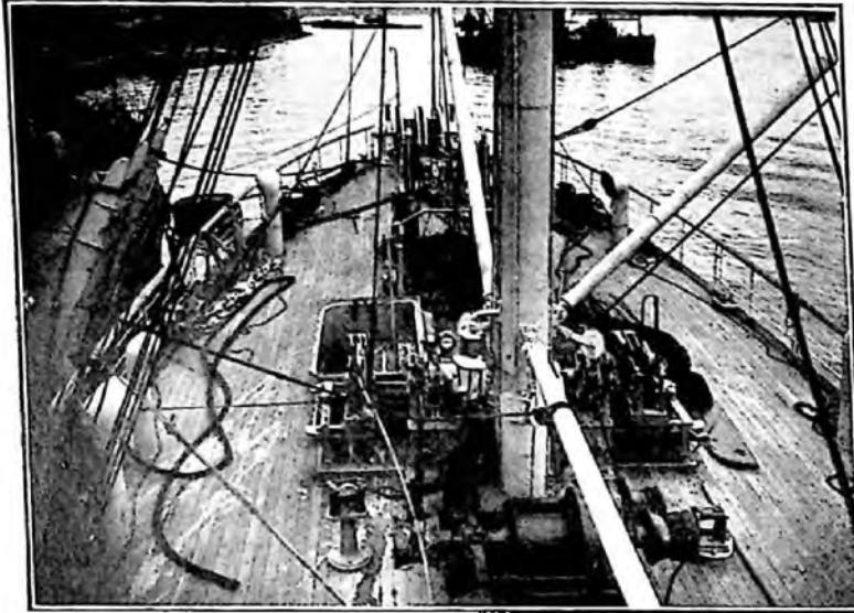
FIG. 5.—H.M.T.S. "IRIS." GENERAL VIEW OF FORE DECK—LOADING CABLE AT DEPOT.
