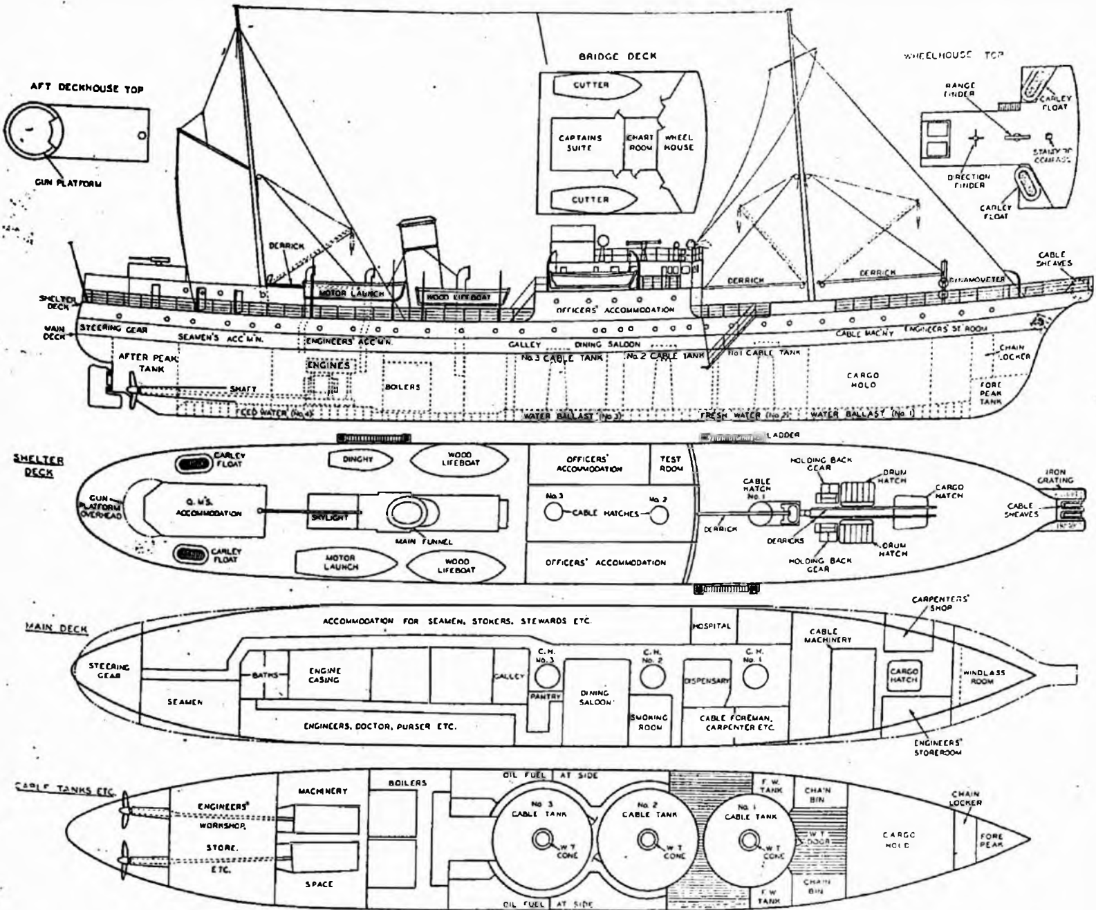
FIG. 2.—H.M.T.S. "Iris." GENERAL ARRANGEMENT (SCALE 1/32 IN.=1'FT.).
