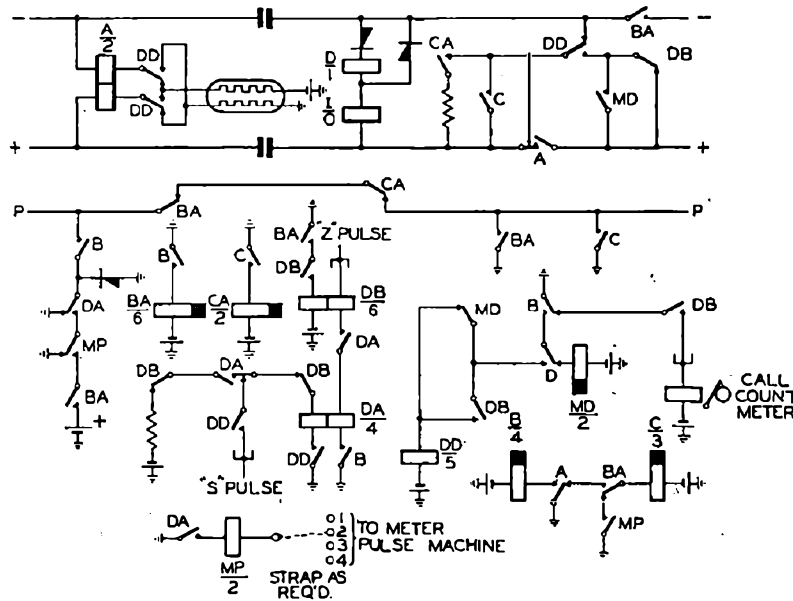
FIG. 2.—AUTO-AUTO RELAY SET WITH MULTI-METERING.
