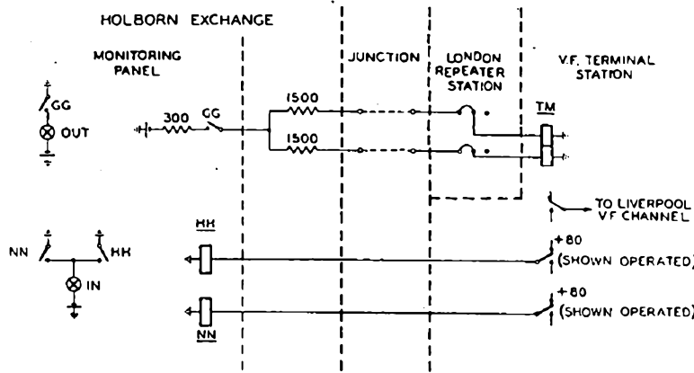
FIG. 4.—MONITORING CIRCUIT
