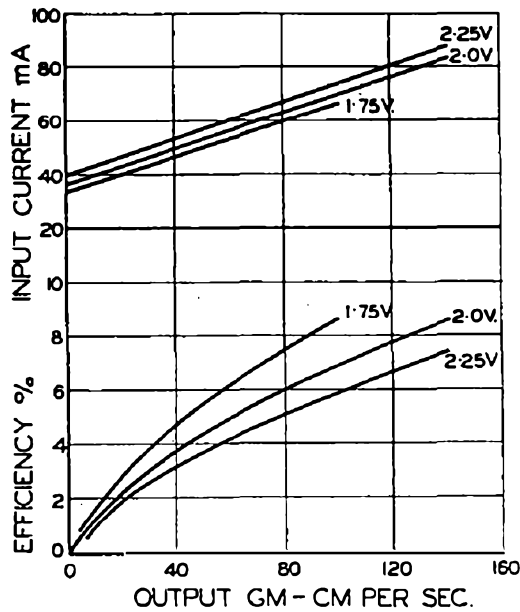
FIG. 7.—PERFORMANCE CURVES OF EXPERIMENTAL MOTOR.
