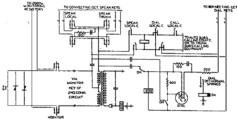
FIG. 6.—OPERATOR'S CIRCUIT.
