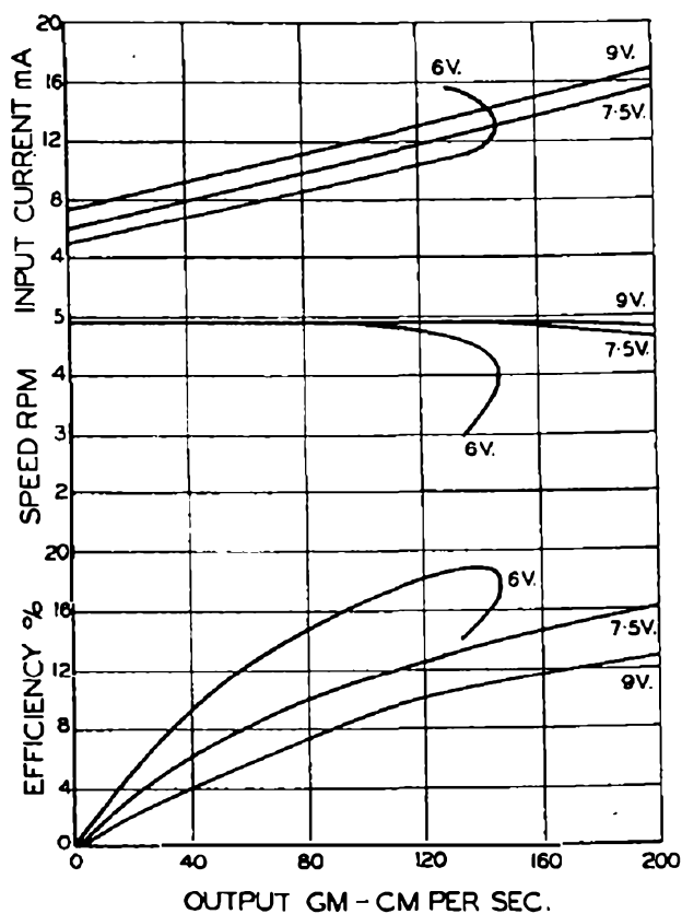
FIG. 4.—PERFORMANCE CURVES OF WALLACE AND TIERNAN MOTOR.
