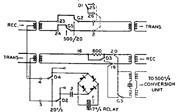
FIG. 2.—OPERATION OF RINGER IN 4-WIRE LINE.
