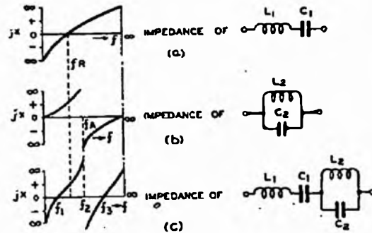
FIG. 5.—IMPEDANCE CURVES OF REACTIVE CIRCUITS.
