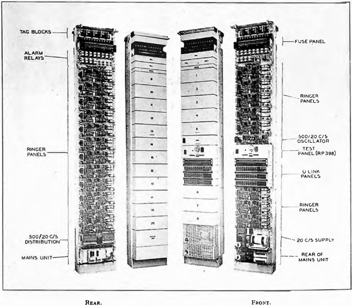
FIG. 6.—REAR AND FRONT VIEWS OF COMPLETE BAY.
