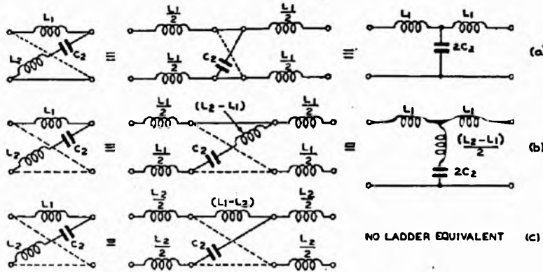
FIG. 4.—EQUIVALENT LATTICE AND LADDER NETWORKS.
