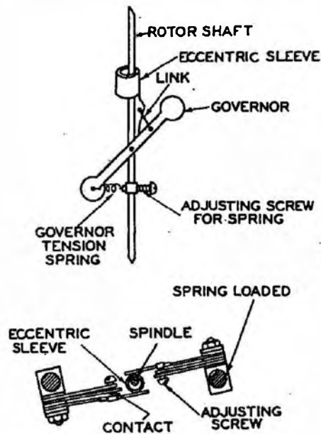
FIG. 2.—GOVERNOR DETAILS. WALLACE AND TIERNAN MOTOR.
