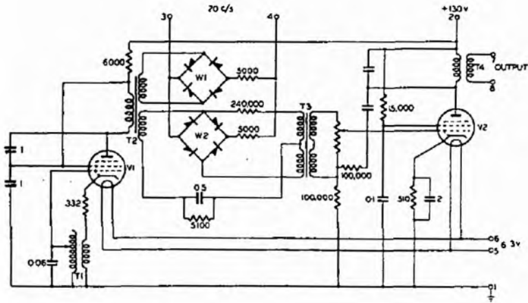
FIG. 4.—500 c/s Oscillator with Static "Chopper."
