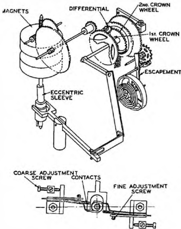
FIG. 6.—CONSTRUCTIONAL DETAILS OF EXPERIMENTAL MOTOR.
