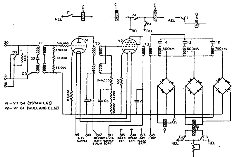
FIG. 3.—500/20 c/s CONVERSION CIRCUIT.
