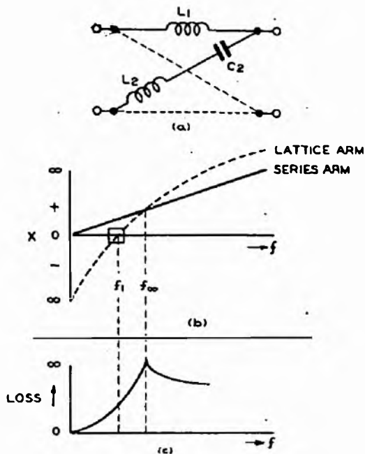
FIG. 2.—REACTANCE AND LOSS CURVES FOR A SIMPLE LOW-PASS LATTICE FILTER NETWORK.
