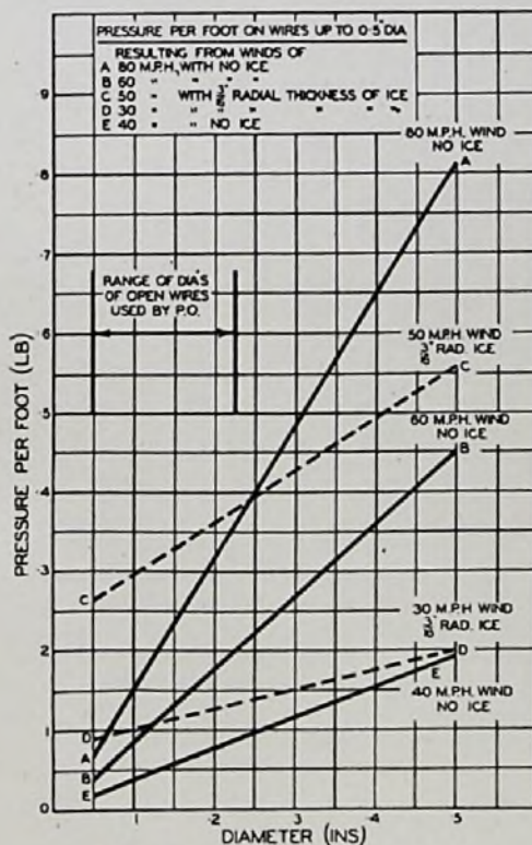
FIG. 1.—WIND PRESSURE CURVES.
