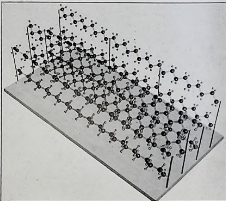
FIG. 1.—MODEL SHOWING ARRANGEMENT OF CARBON AND HYDROGEN ATOMS AND ALIGNMENT OF MOLECULAR CHAINS IN POLYTHENE.
