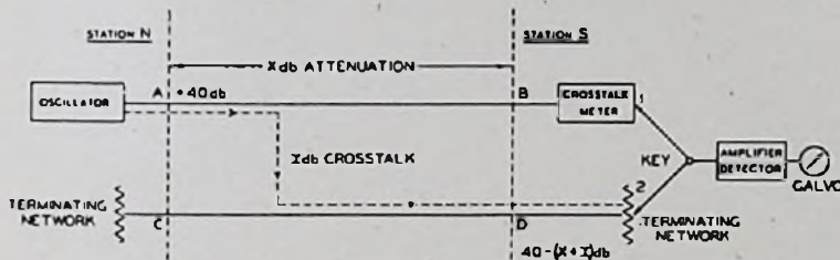
FIG. 1.—SCHEMATIC DIAGRAM SHOWING METHOD OF MEASURING CROSSTALK AND THE LEVELS RELATIVE TO 1 mW.
