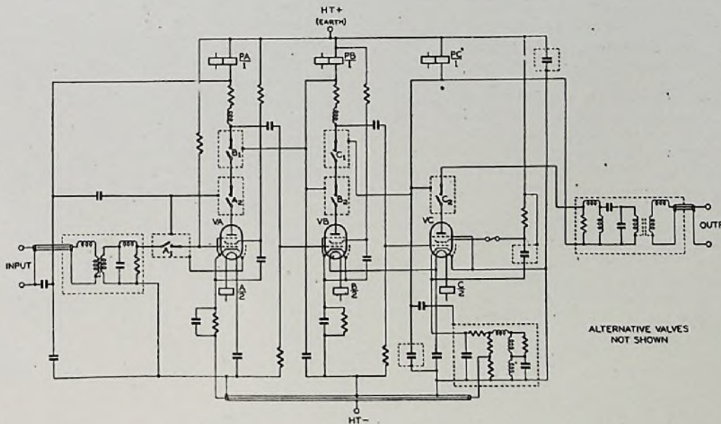
FIG. 8.—AMPLIFIER CIRCUIT.
