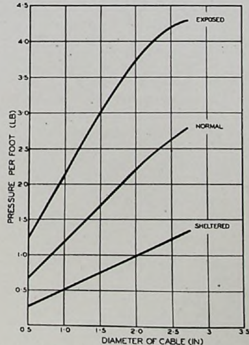
FIG. 2.—WIND PRESSURE CURVES FOR AERIAL CABLE ERECTED IN VARIOUS SITUATIONS.
