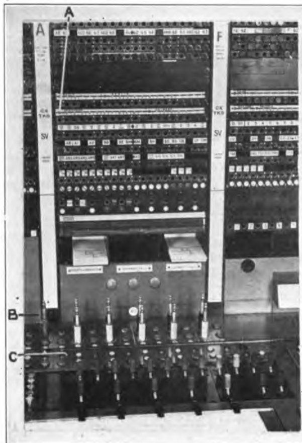
FIG. 1.—SWITCHBOARD FITTED WITH DELAY INDICATOR.
