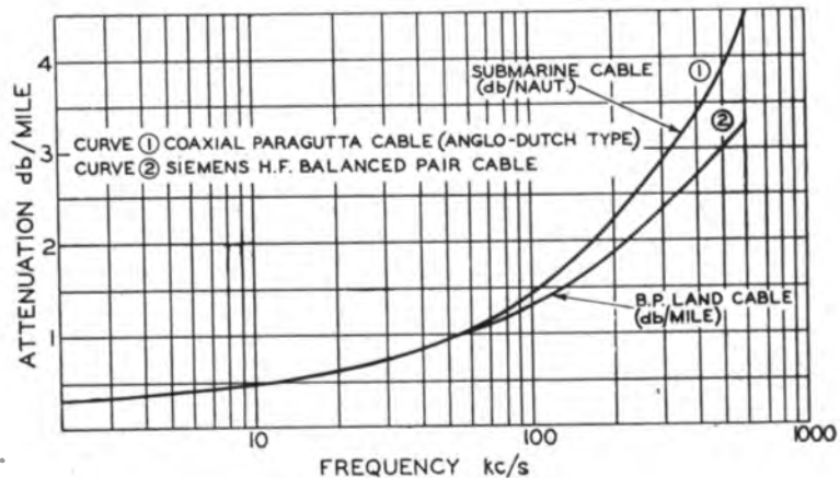
FIG. 1.—CABLE ATTENUATIONS.
