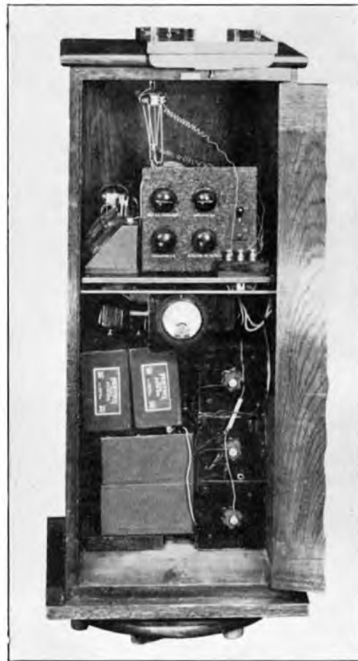
FIG. 10.—RECEIVER CABINET.
