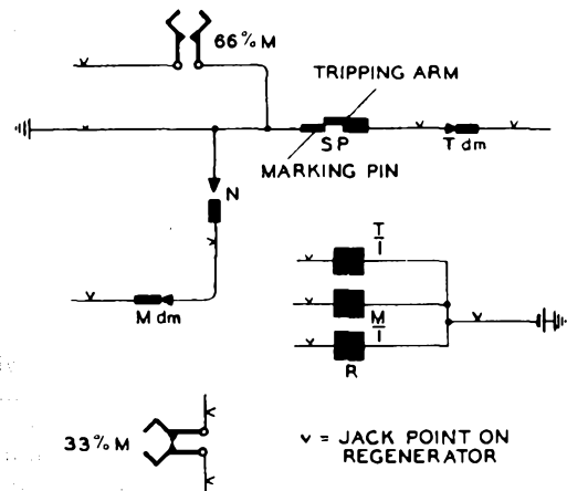
FIG. 12.—REGENERATOR CIRCUIT ELEMENTS AND ACCESS POINTS.
