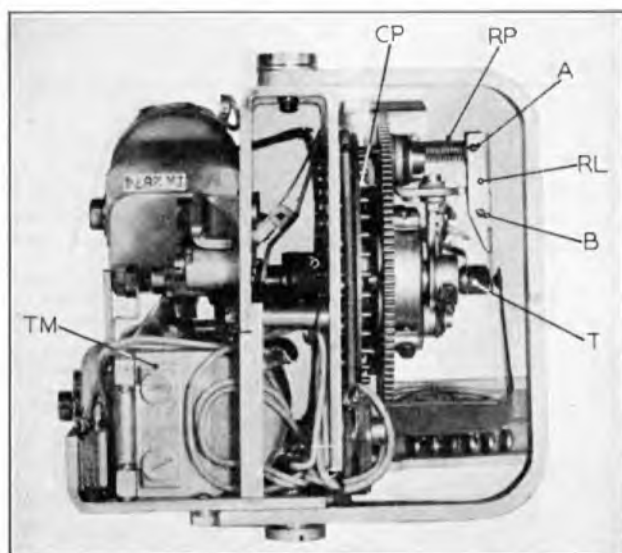
FIG. 1.—FRONT VIEW.
