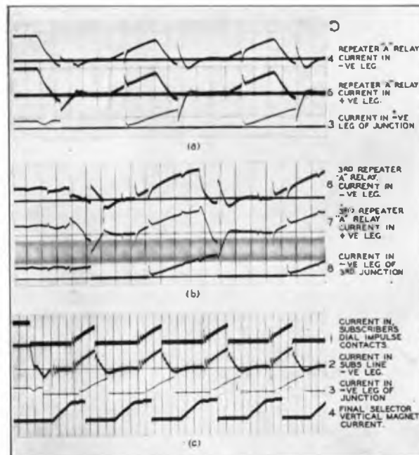
FIG. 17.—WAVEFORMS OF A RELAY CURRENTS (FOR POSITION OF OSCILLOGRAPH POINTS, SEE FIG. 1).
