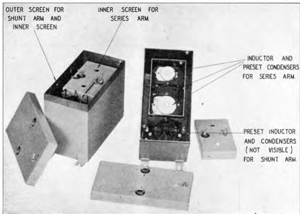
FIG. 21.—DOUBLE SCREENED FILTER SECTIONS.
