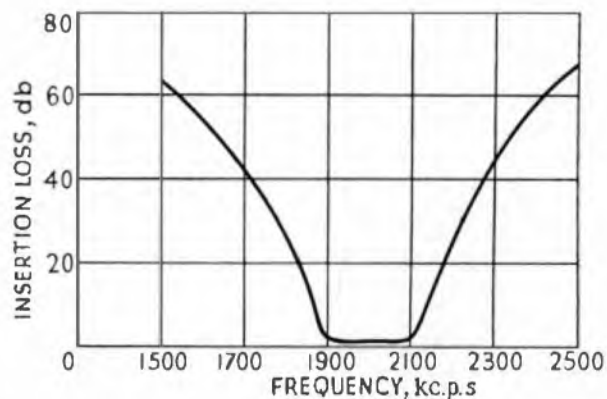
FIG. 22.—INSERTION LOSS CHARACTERISTIC OF SUPER GROUP FILTER.
