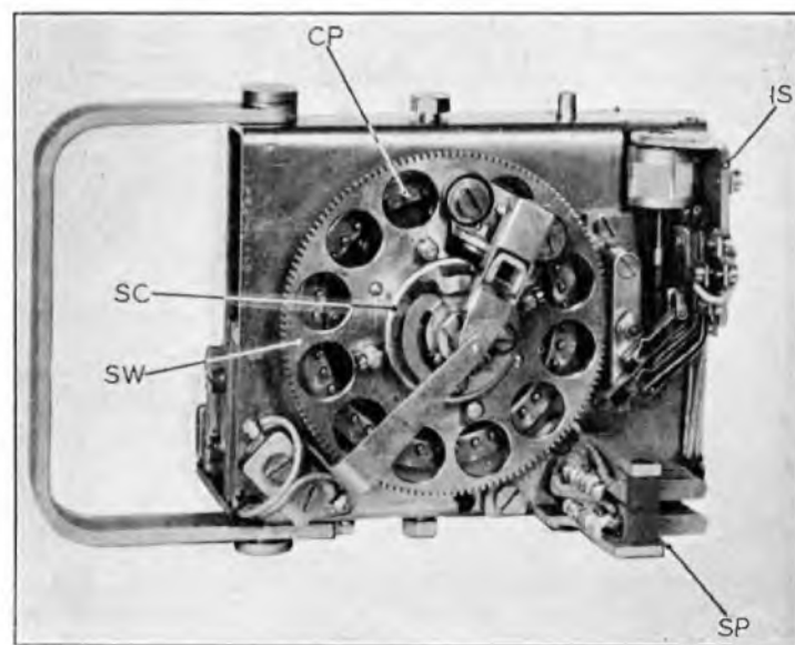
FIG. 3.—TRANSMITTING ELEMENT.
