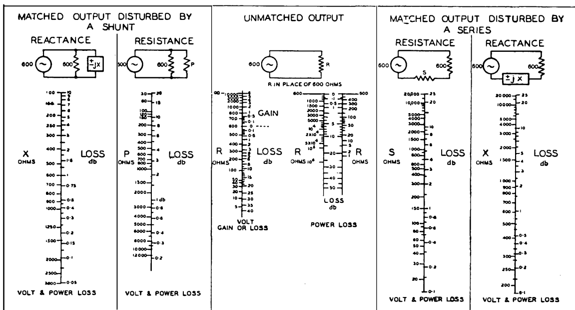
FIG. 1.—ABACS GIVING MISMATCH LOSS.
