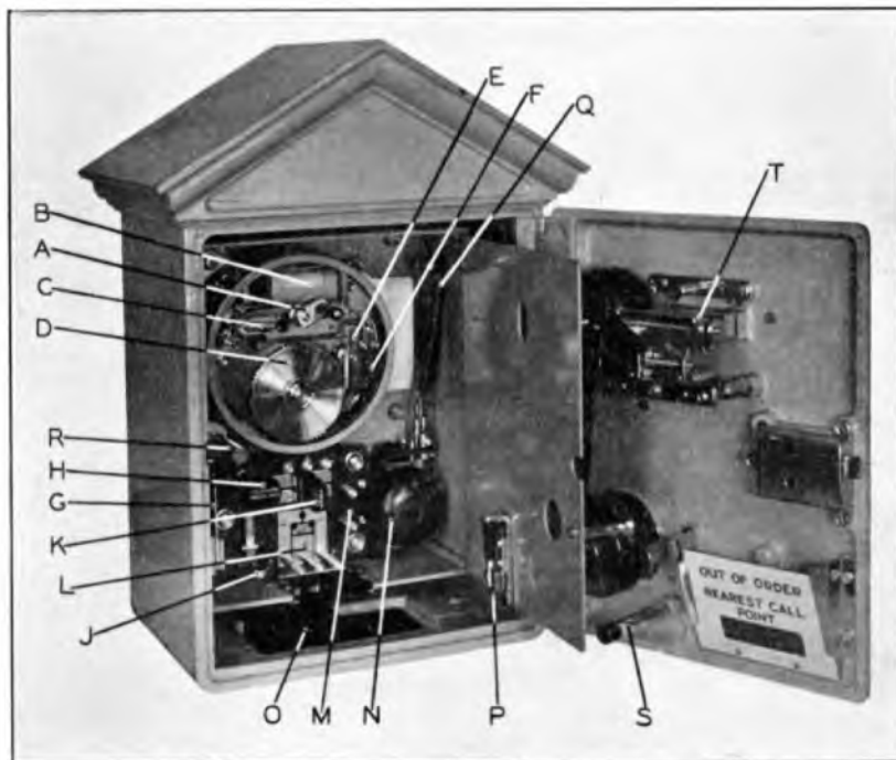
FIG. 3.—INTERIOR OF THE SUCCESSION ALARM BOX.
