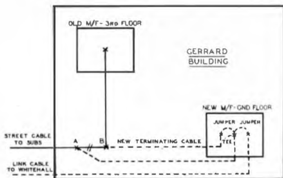
FIG. 2.—CABLING ARRANGEMENTS.
