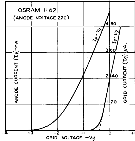
GRAPH 1. VALVE CHARACTERISTIC.
