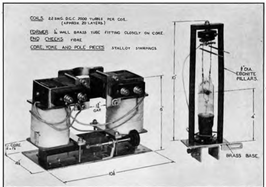
FIG. 5.—ELECTROMAGNET AND MAGNETRON SHOWING MOUNTING.
