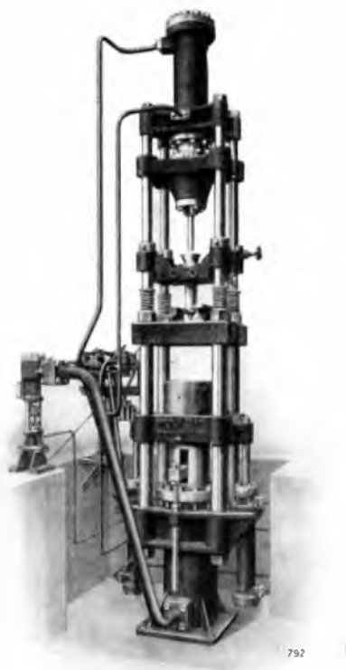
FIG. 3.—COMBINED INJECTION AND MOULDING PRESS.
