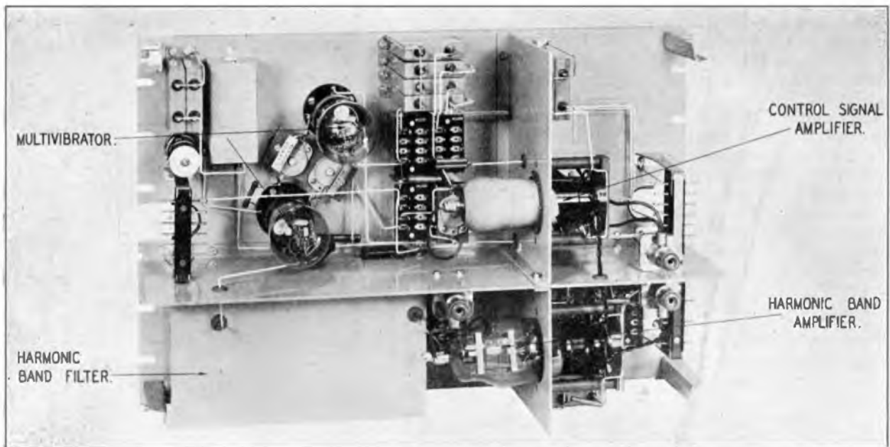
FIG. 28.—MULTI-VIBRATOR UNIT.
