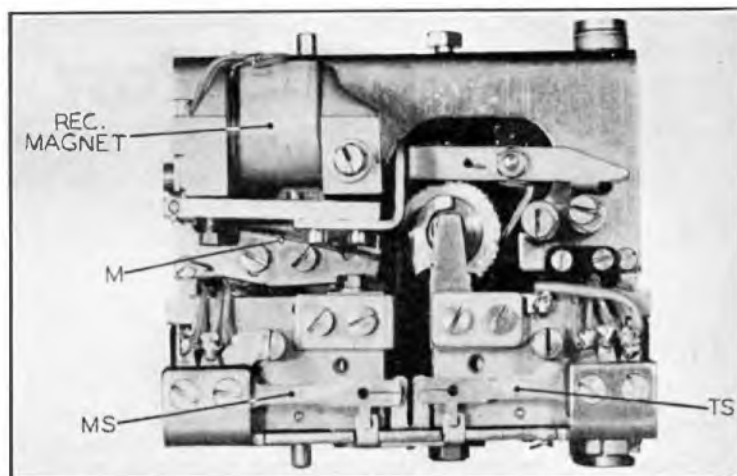
FIG. 2.—RECEIVING AND MARKING ELEMENT.
