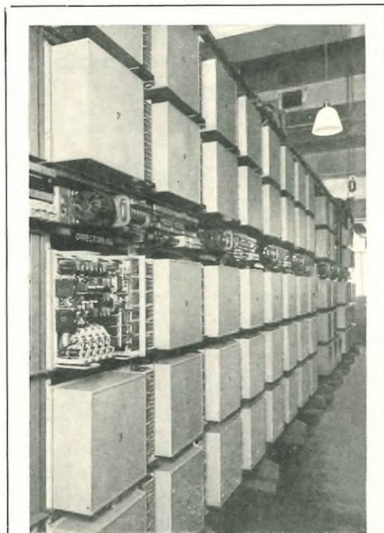
Director Racks at "Flaxman," the first fully equipped 10,000 line Automatic Exchange in London manufactured and installed by the G.E.C.
