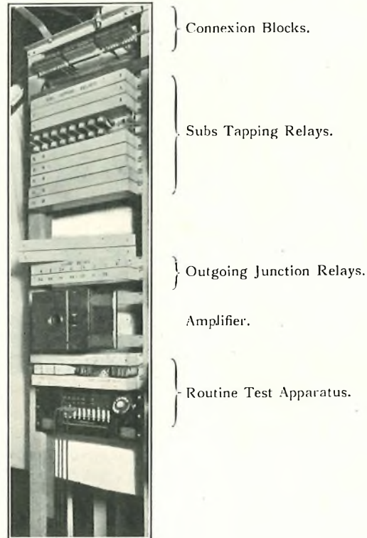
FIG. 3.—EQUIPMENT AT OBSERVED AUTOMATIC EXCHANGE.
