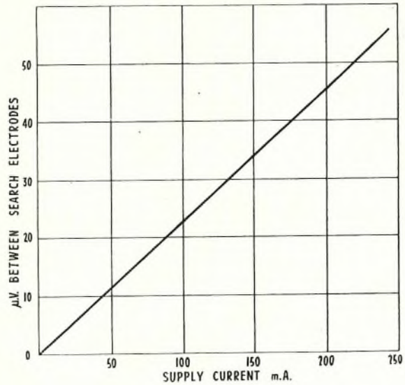
FIG. 6.—ELECTRODE P.D. VERSUS SUPPLY CURRENT.
