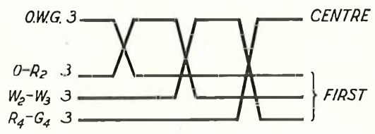
FIG. 2.—INTERLAYER SEPARATION JOINT FOR 24-PAIR CABLE.
