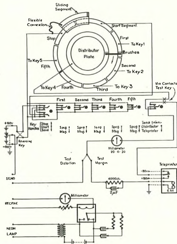
FIG. 2.—TELETYPE DISTORTION AND MARGIN TESTER; PRINCIPLE CONNEXIONS.
