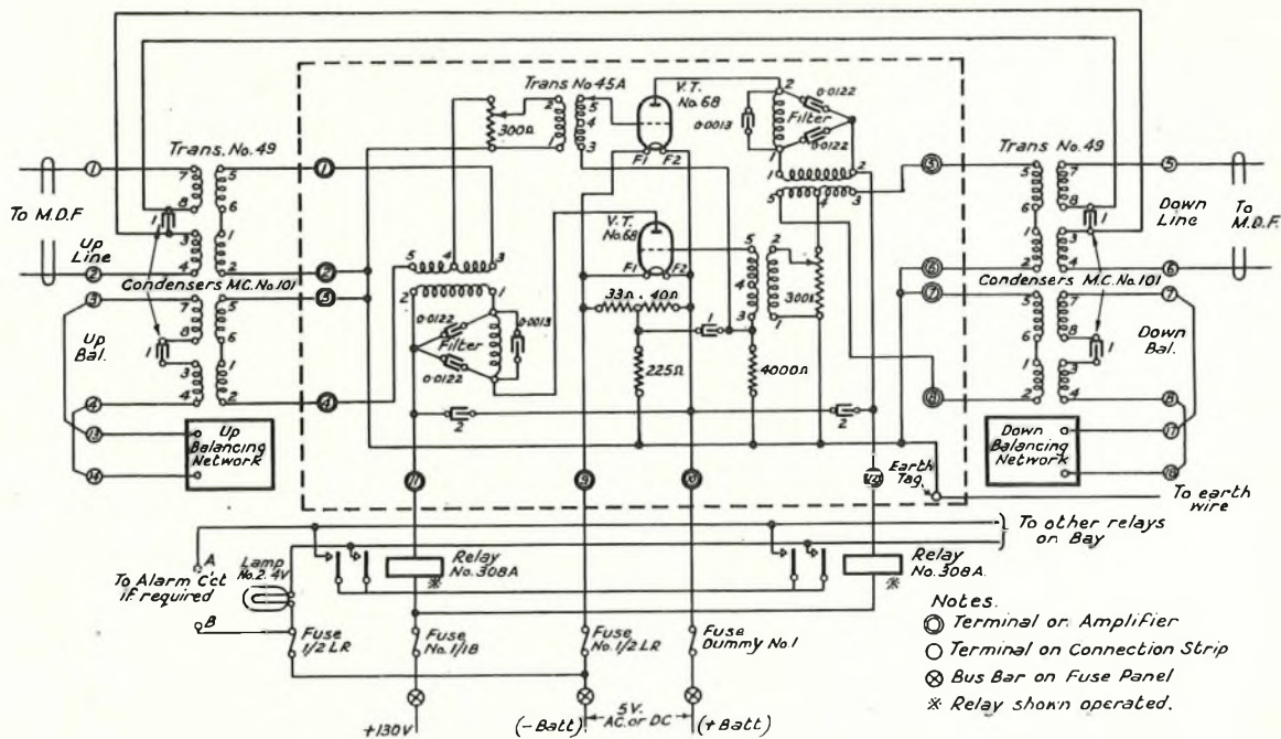
FIG. 7.—TWO-WIRE REPEATER.
