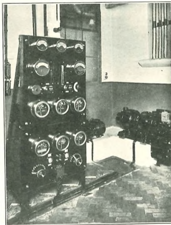
FIG. 8.—POWER BAY.
