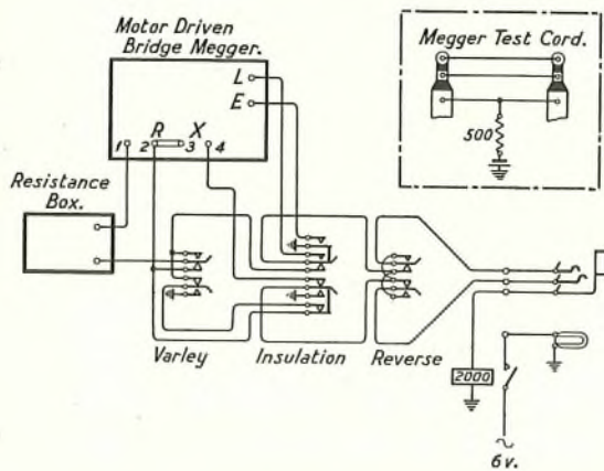
FIG. 5.—CIRCUIT OF BRIDGE MEGGER.
