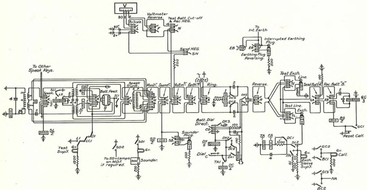
FIG. 4.—TEST CORD CIRCUIT.
