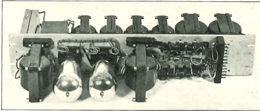
Two-wire Repeater.
