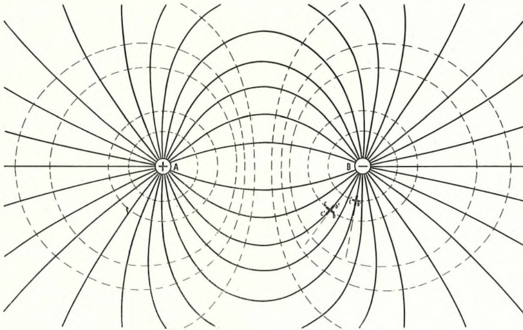
FIG. 1.—FORM OF CURRENT PATHS FROM EARTH FAULT.
