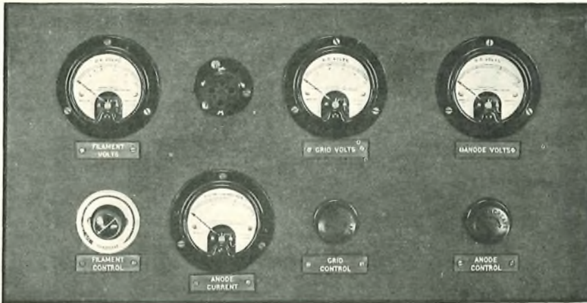
FIG. 5.—VALVE TEST PANEL.
