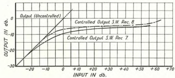
FIG. 3.—EFFECT OF AUTOMATIC CONTROL ON RECEIVER OUTPUT.
