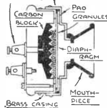
Fig. 3—Hunning's use of carbon granules
