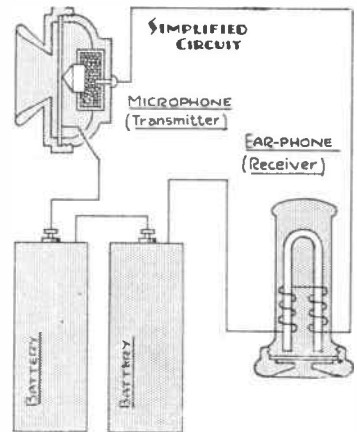
Fig. 5—The basic principles of the telephone circuit are unchanged
