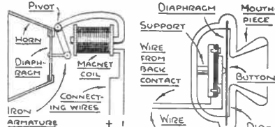
Fig. 1—Bell's early type transmitter
