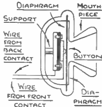
Fig. 2—Edison's carbon transmitter
