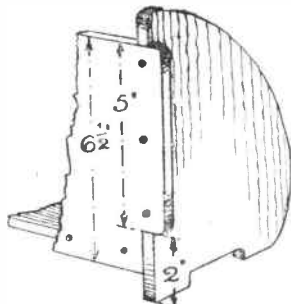
Fig. 4—The back rail fixing
