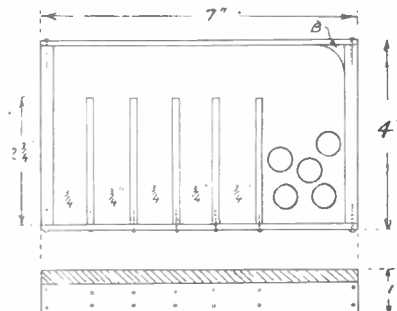
Fig. 2—Dimensions of the parts needed
