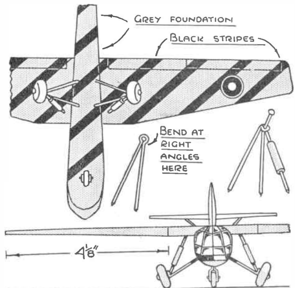
Fig. 3—Under view and front elevation
