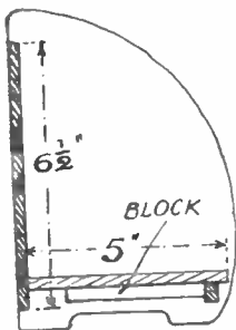
Fig. 1—End details
