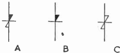
Fig. 2.—A suggested new symbol for barrier layer photo-cell more fully indicating its function. It is derived from B in the dark stage and C when illuminated.
