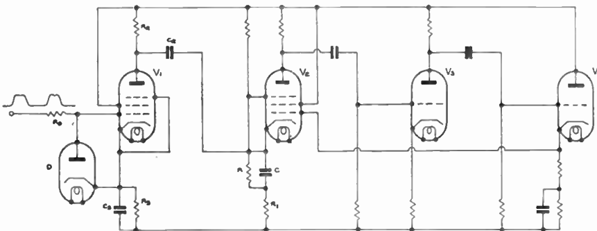
Fig. 22—Improved modulator circuit.
