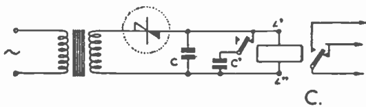
Fig. 4C.—Method of increasing sensitivity to small changes of illumination.
