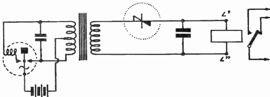
Fig. 11.—Battery fed A.C. switching current.
