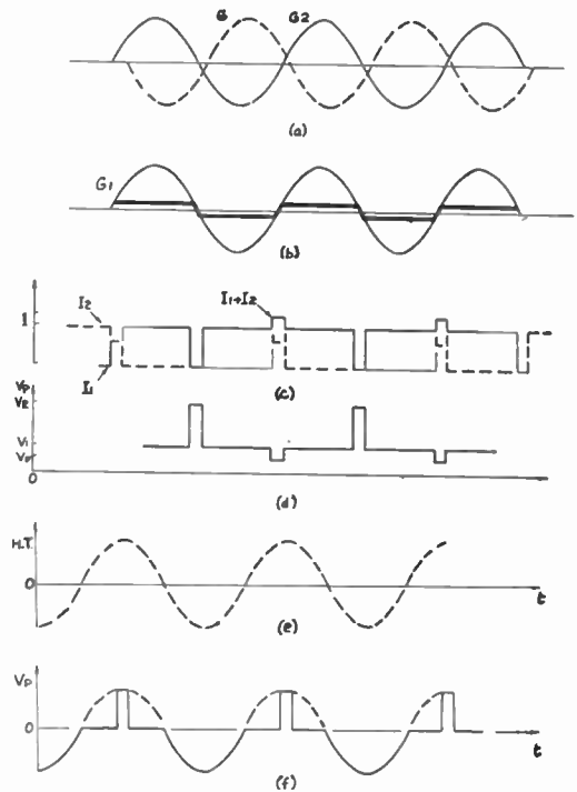
Fig. 13.—Working diagrams of the power pulse generator of Fig. 12.
