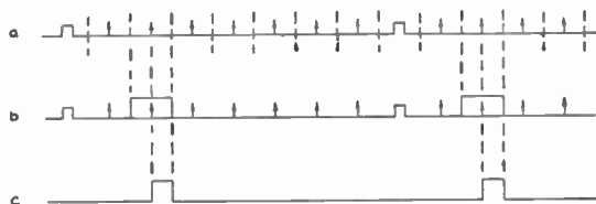
Fig. 20.—Demodulation process.
