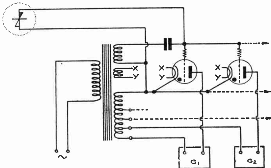
Fig. 9.—Grading circuit to strike each gas relay at different low levels of illumination, both gas relays are inoperative with much illumination.
