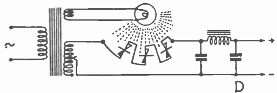
Fig. 4D.—Low voltage stabilised power unit using new effect.
