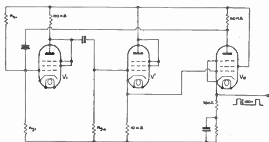
Fig. 16.—Practical power pulse multivibrator circuit.
