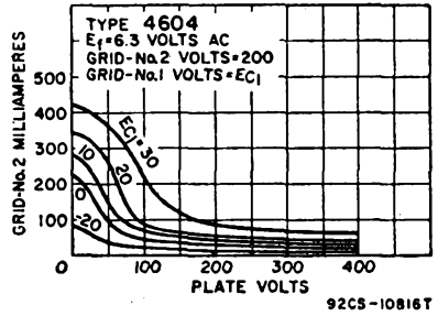
TYPICAL CHARACTERISTICS
