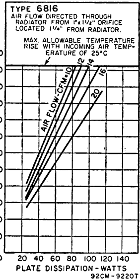
TYPICAL COOLING REQUIREMENTS
