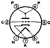
VIEWED FROM SHORT END
