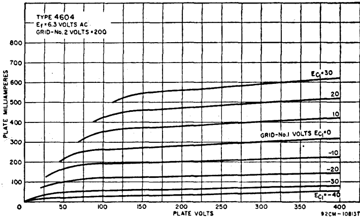
TYPICAL CHARACTERISTICS
