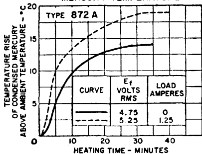
RATE OF RISE OF CONDENSED-MERCURY TEMPERATURE
