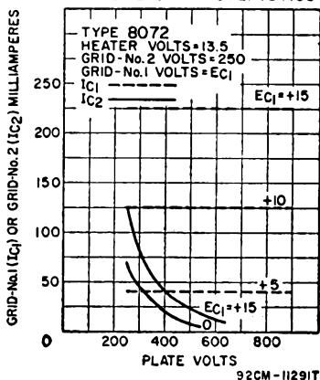
TYPICAL CHARACTERISTICS
