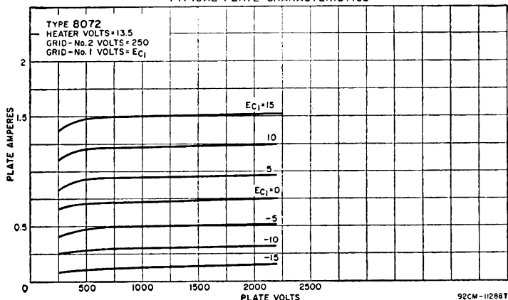
TYPICAL CHARACTERISTICS
