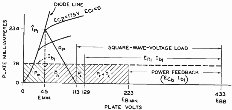
Fig. 16—Plate-load diagram of deflection power tube ( V_1 ).
