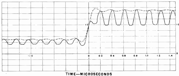
GREEN RESPONSE TO BAND LIMITED STEP FUNCTION SUMS OF SCANS f_0 = 2.4 Mc., f_B = 4.1 Mc., f_A = 2.0 Mc.
