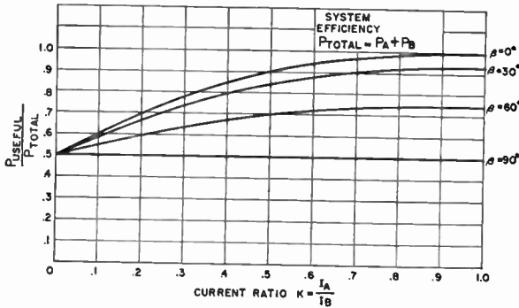
Fig. 3—Power in the useful load in terms of the total power as a function of the ratio of the currents produced by the two generators.
