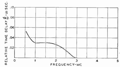
Fig. 5—Delay distortion introduced by VSB transmission.
