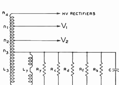
Fig. 13—Shunt-loss diagrams of deflection circuit.
