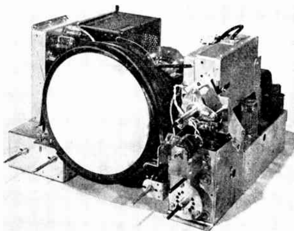
Fig. 12—Standard VHF chassis with UHF tuner added.
