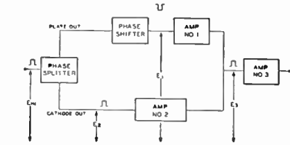
Fig. 3—Block diagram of phase compensating network.
