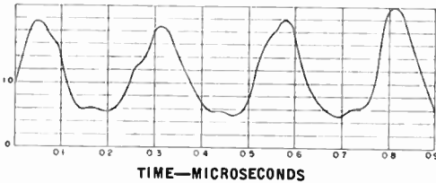
(e) Combined light intensity of two successive scans of the same line, obtained by adding light intensities of the green, red and blue tubes.
