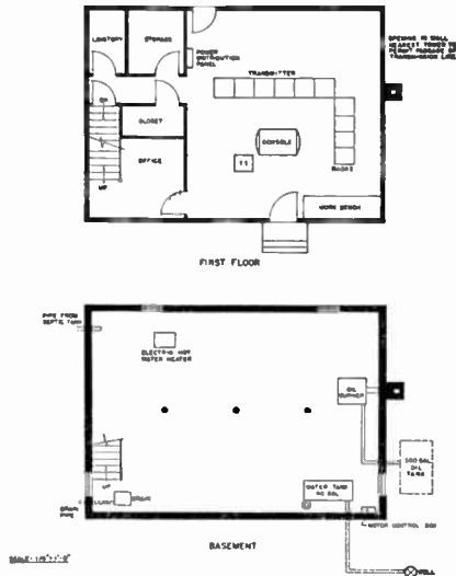
Fig. 4—Floor plans of transmitter building.
