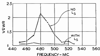
Fig. 12—Standing wave ratio of sample run of UHF transmission line.
