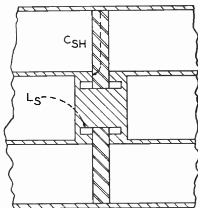
Fig. 11—Section of compensated undercut insulator for \frac{3}{8} -inch diameter coaxial line.
