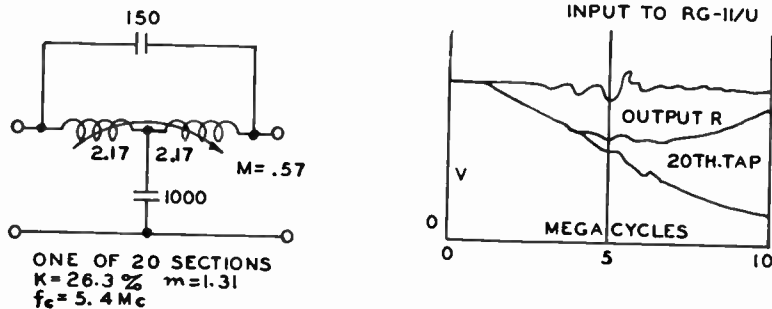
Fig. 6—Same as in Figure 5 except the half-section coils pushed together.
