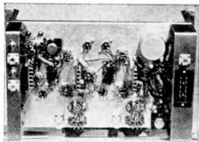
Fig. 13—Phase and amplitude equalizer (rear view).
