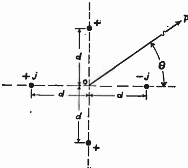
Fig. 1 — Simplified four-radiator array.
