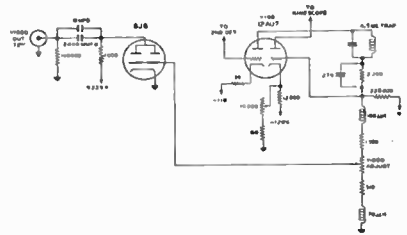
Fig. 7a—Revised video output circuit of Channel 4 receivers.
