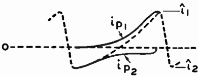
Fig. 5c—Waveform distortion increasing the average value of i_{p2} .
