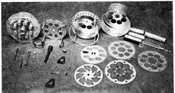
Fig. 7—Disassembled cavity.
