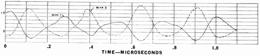
Fig. 10(b)—Signal on the green kinescope grid of a color television receiver.
