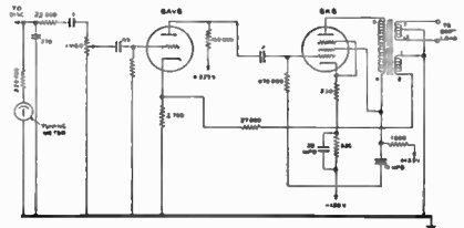
Fig. 7b—Revised audio amplifier circuit of Channel 4 receivers.
