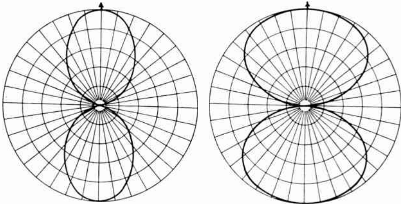
A. Broadside array.
