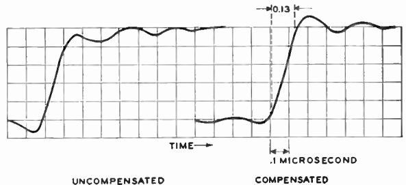
Fig. 11—Overall response of station WNBW + station monitor.
