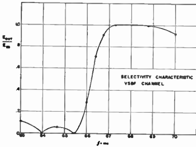
Fig. 20—Frequency-response characteristic of the vestigial sideband filter.
