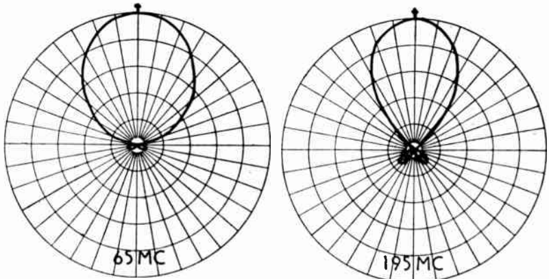
A. Combination array, d = 90^\circ . B. Combination array, d = 270^\circ .
