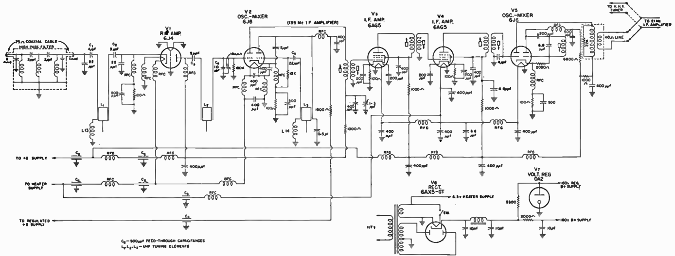
Fig. 2—Circuit diagram of UHF tuner and power supply.
