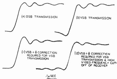
Fig. 7—Television receiver square-wave response.
