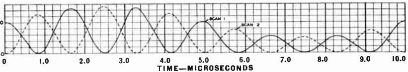
Fig 25(b)—Effective light intensities for two scans on the same line of the blue tube. Sampling frequency is 0.6 megacycle.
