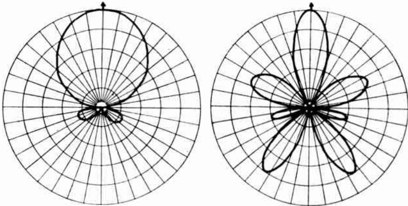
C. Combination array, d = 90^\circ .
