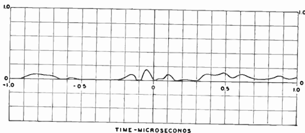
Fig. 18—Combined light intensity of two successive line scans of the same line on the red kinescope.
