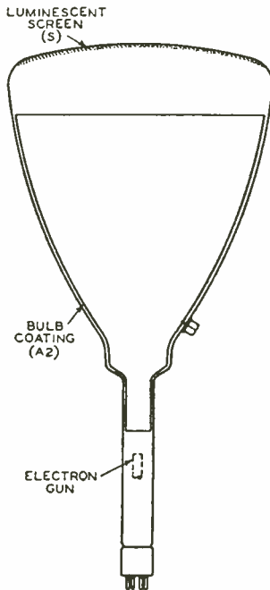
Fig. 11—Schematic section of a Kinescope.
