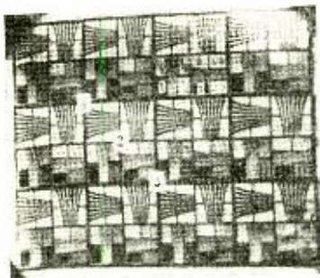
FIG. 13—Resolution pattern reproduced by electrostatic-image iconoscope.
