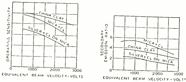
Fig. 9—Properties of various mosaics.
