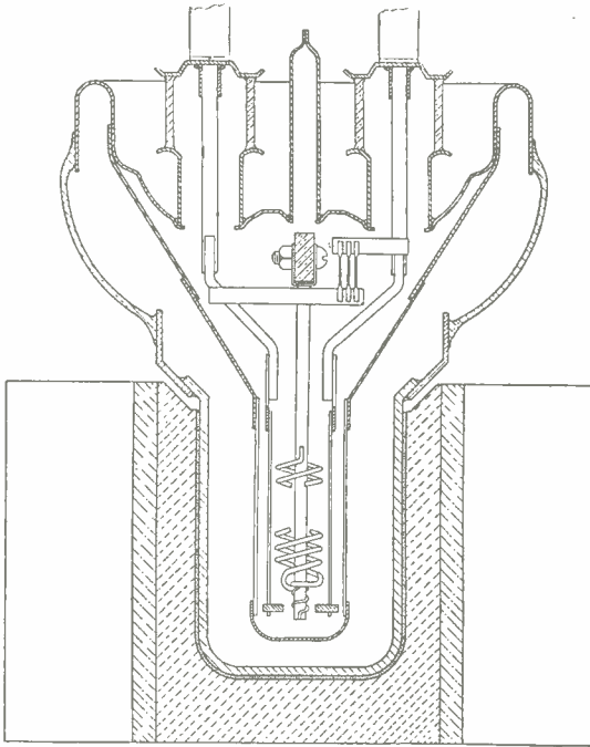
Fig. 2—Cross section of tube.
