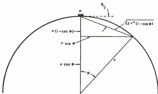
Fig. 6—Geometric considerations relative to the analysis of the effect of screen curvature.
