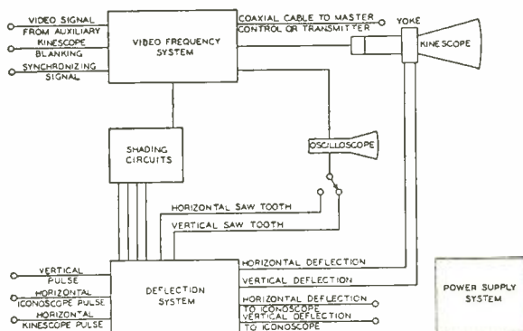
Fig. 11—Block diagram of camera-control unit.
