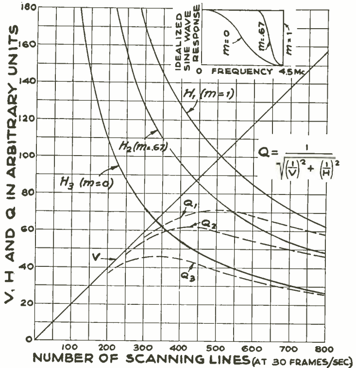
Fig. 9—The V and H -curves are vertical and horizontal resolution, respectively, provided by receivers having the idealized over-all frequency characteristics shown in the insert. The Q -curves are intended to indicate the corresponding picture quality as a function of the number of scanning lines.
