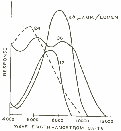
Fig. 3—Spectral response of semitransparent photocathodes.
