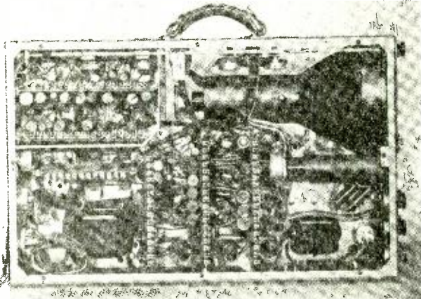
Fig. 13—Camera-control unit—circuit-component side, cover removed.
