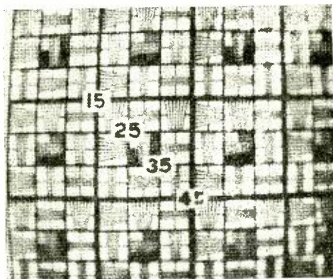
Fig. 8—Resolution pattern by magnetic-image tube.
