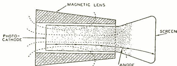
Fig. 7.—Magnetic-image tube.
