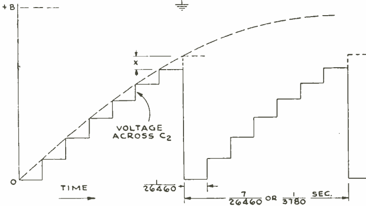
Fig. 2—(a) Frequency Divider. (b) Shows how C_2 is charged in steps through V_3 and C_1 and discharged at intervals by V_4 .
