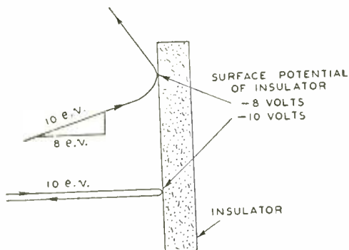
Fig. 3—Electron paths near target.
