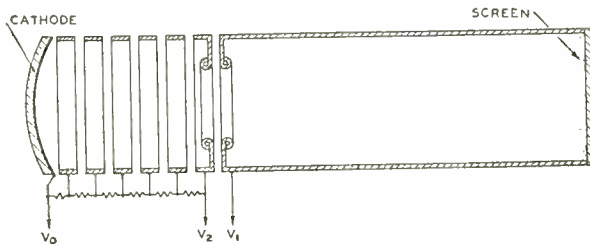
Fig. 6—Electrostatic-image tube.
