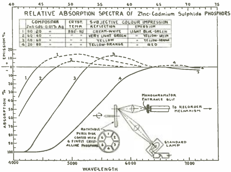
Fig. 2—Absorption spectra of zinc cadmium sulphide phosphors.
