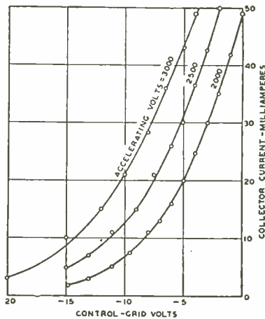
Fig. 8—Static characteristics of a developmental tube
