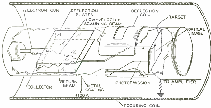
Fig. 9—Schematic diagram of an Orthicon.
