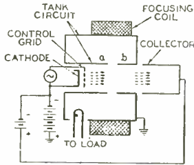
Fig. 1—Schematic diagram of a grid-controlled inductive-output amplifier.
