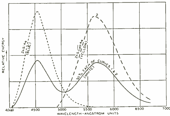
Fig. 20—White-emitting binary phosphor mixture.
