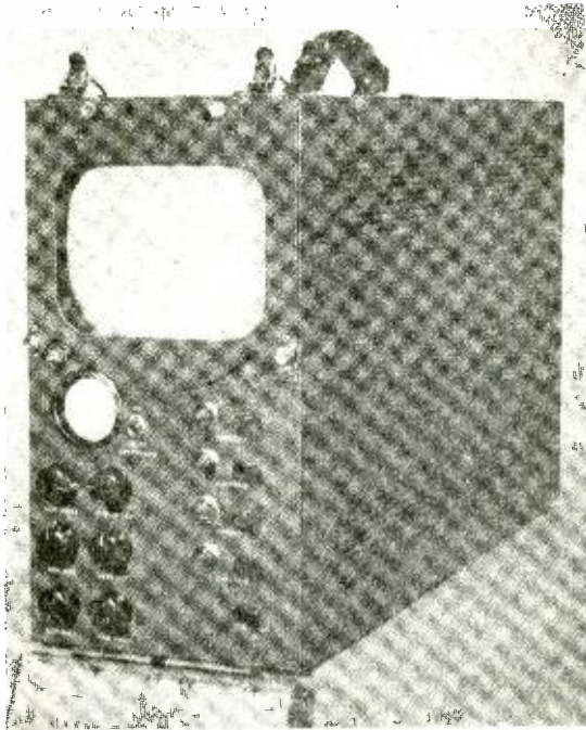
Fig. 16—Master-control unit—front view.
