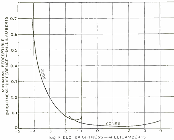
Fig. 24—Minimum perceptible brightness difference as a function of field brightness.
