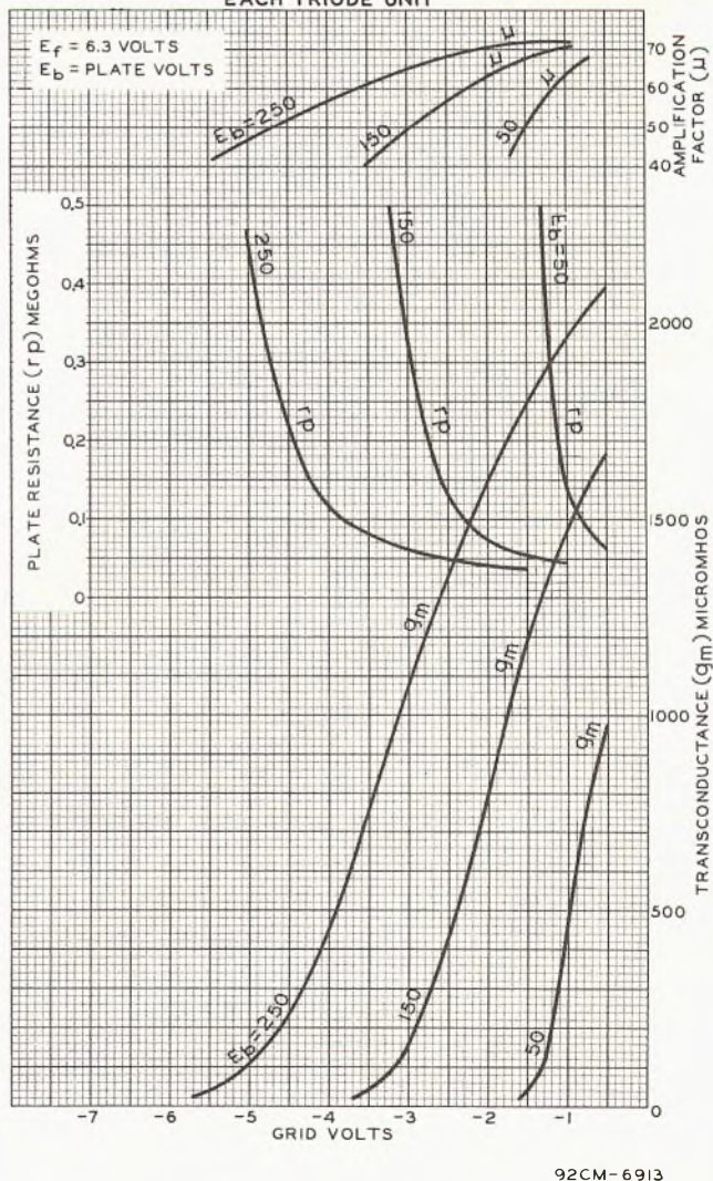
AVERAGE CHARACTERISTICS EACH TRIODE UNIT
