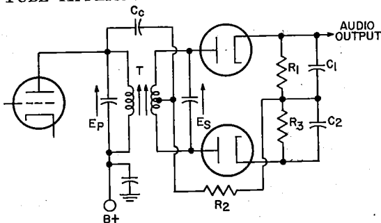
Fig. 30—Balanced phase-shift discriminator circuit.
