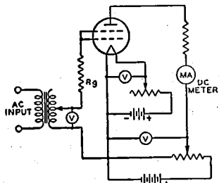
Fig. 134—Fundamental circuit of a power-output tester for class B operation of tubes.
