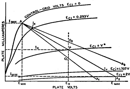
Fig. 43—Graphic calculations for class A amplifier using a pentode or beam power tube.
