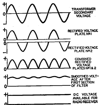
Fig. 17—Voltage waveforms of full-wave rectifier circuit.
