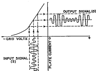
Fig. 34—Current characteristics of class A amplifier.
