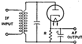
Fig. 22—Basic diode-detector circuit.
