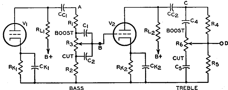
Fig. 58—Two-stage tone-control circuit incorporating separate bass and treble controls.
