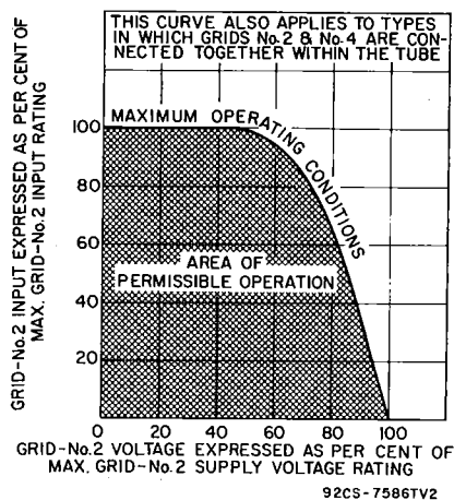
Fig. 128—Grid-No. 2 input rating curve.
