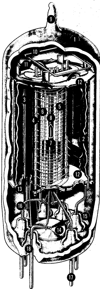
Structure of a Miniature Tube
