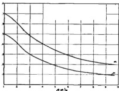
Fig. 1—Minimum value of \alpha for which complex roots exist and the corresponding \mu .
