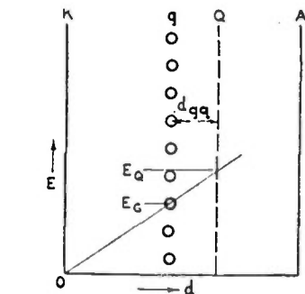
Fig. 7—Determination of equivalent potential E_Q of the Q plane.
