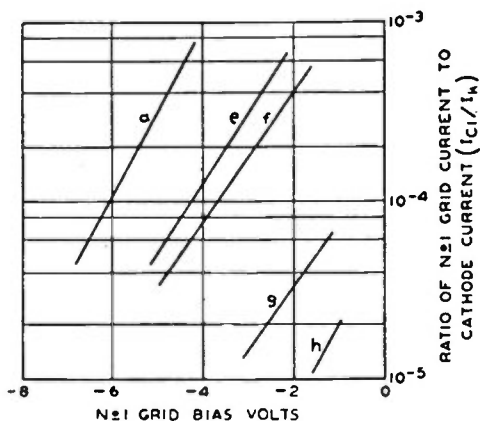
Fig. 21—Signal-grid (grid No. 1) current of the outer-grid injection mixers shown in Fig. 20. Curve a corresponds to the original design ( a ) of Fig. 18 and is shown for comparison. Data taken with a 20-megacycle oscillator voltage of 12 volts peak amplitude applied to the oscillator-grid. E_{c3} = -10 volts, E_{c2} and \epsilon = 100 volts, E_b = 250 volts.
