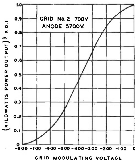
Fig. 11— Modulation characteristics.
