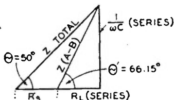
EQUIV. SERIES CIRCUIT AT \omega = 377
