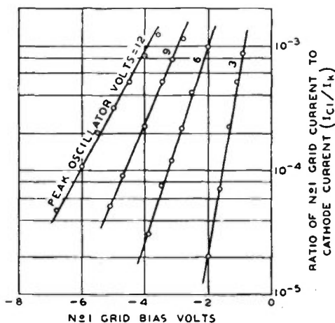
Fig. 15—Signal-grid (grid No. 1) current in a typical mixer with a 20-megacycle oscillator voltage applied to grid No. 3. E_{c3} = -10 volts. E_{r2 \text{ and } 1} = 100 volts, E_b = 250 volts.
