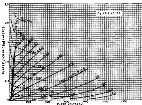
Fig. 12—Characteristic curves.
