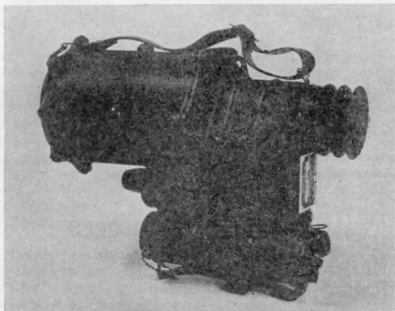
Fig. 1—Infrared telescope.
