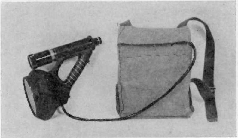
Fig. 9—Laboratory prototype Sniperscope.
