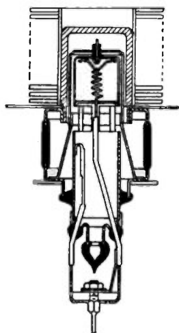
Fig. 1—Cross section of the H-2614 pulse triode.
