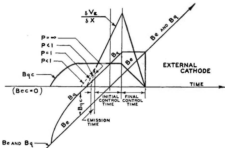
Fig. 4—Time variation of the magnetic field, magnetic flux and electric field.
