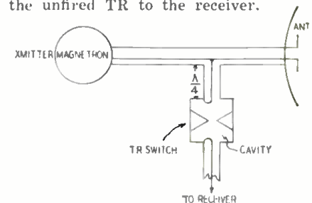
Fig. 5—TR switch in antenna circuit.
