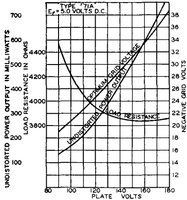
AVERAGE CHARACTERISTICS
