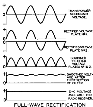
FULL-WAVE RECTIFICATION
