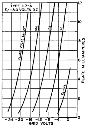
AVERAGE CHARACTERISTICS
