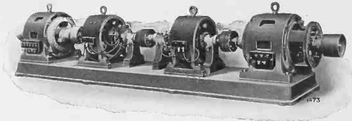
Motor Generator set for Variable Frequency, Phase and Voltage
