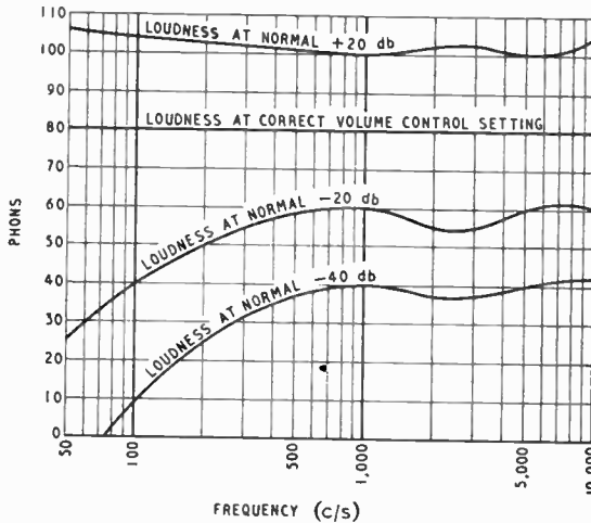
Fig. 2. Scale distortion when 80-phon sound is reproduced at various volume-control settings, derived from Fig. 1.
