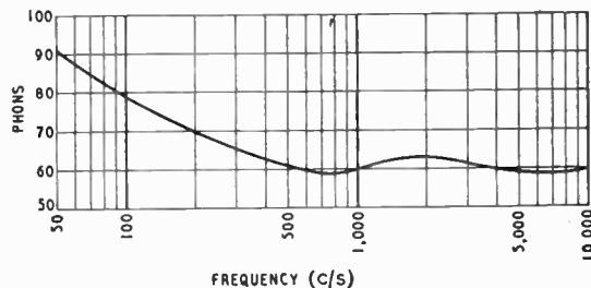
Fig. 4. If the compensated 60-phon characteristic of Fig. 3 were used, instead of a level one, to reproduce sound life-size at 60 phons, the result would be excessive bass as shown here.
