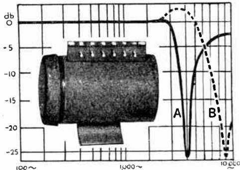
A Tuned for maximum rejection at 4,000 cycles B Tuned for maximum rejection at 9,000 cycles
