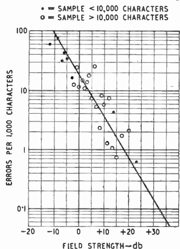
Fig. 4. Field strength/error curve for on-off keying. Three-receiver diversity reception, 1 kc/s I.F. bandwidth. 0 db = 1\mu\text{V/m} .
