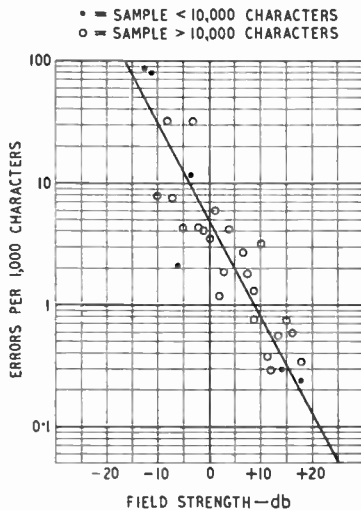
Fig. 3. Field strength/error curve for frequency-shift keying. Two-receiver diversity reception, I.F. bandwidth 1 kc/s. Frequency shift 850 c/s. 0 db = 1\mu\text{V/m} .
