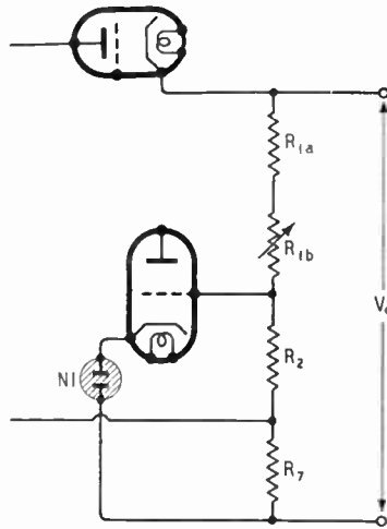
Fig. 11. Output current feedback, normally used together with input voltage feedback, to neutralize the resistance of V_i .
