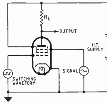
Fig. 1. A simple pentode "gate" circuit.
