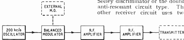
Fig. 2. Mixer-oscillator frequency-shift exciter.
