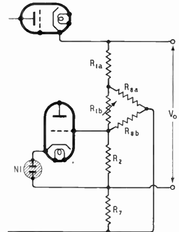
Fig. 12. Modification of Fig. 11 to make it independent of R_{1b} .
