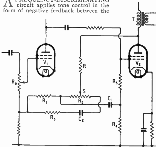
Tone control feedback circuit.
