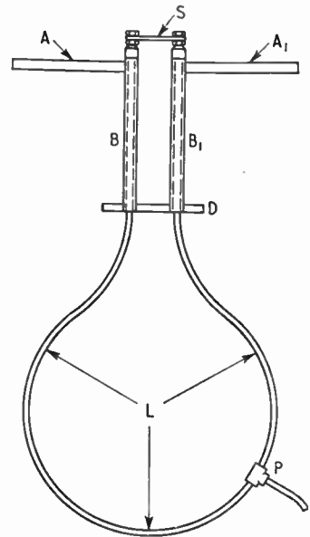
Dipole coupling system.
