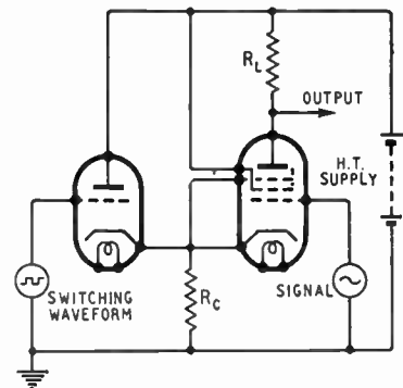
Fig. 2. Cathode-coupled two valve "gate."
