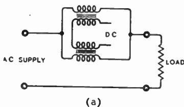
Fig. 2. Methods of eliminating AC from the DC windings of a polarised choke. (a) Separate chokes are connected in parallel with the DC windings in opposition. (b) A single winding is used for DC and the AC fluxes are in opposite phases.
