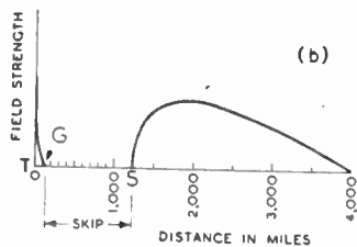
Fig. 1. Diagram (a) shows the extent of the skip zone, while (b) indicates the manner in which field strength varies with distance.
