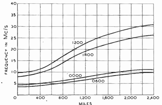
Fig. 5. Skip distances for various frequencies at different times of day.
