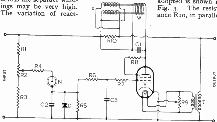
Fig. 3. Complete circuit diagram of AC stabiliser unit. R_1 , 7,000 ohms; R_2 , 1,000 ohms; R_3 , 12,000 ohms; R_4 , 20,000 ohms; R_5 , 0.03 megohm; R_6 , 0.15 megohm; R_7 , 0.25 megohm; R_8 , 200 ohms; R_9 , 50-0-50 ohms; R_{10} , 350 ohms. With the exception of R_3 , which should be rated at 2 watts, all resistances may be of the 1-watt type. C_1 , 8.0 \mu F electrolytic; C_2 , 0.3 \mu F paper; C_3 , 0.5 \mu F paper; V , Osram KT41 tetrode, connected as triode; N , Philips 5-watt neon lamp with cap resistance removed; D , half-wave metal rectifier, rating 20 V, 5 mA.
