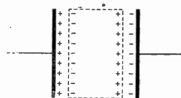
Fig. 3. Effect of polarisation in dielectric of condenser.
