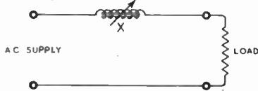
Fig. 1. Basic circuit of "variable series impedance" type of stabiliser.
