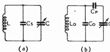
Fig. 2. Significant elements of the superheterodyne input (a) and oscillator (b) circuits.
