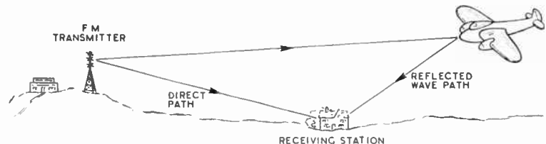
Fig. 1. Reflections from a moving aircraft are received at a slightly altered frequency. The resultant heterodyne with the direct path wave will usually be below the limit of audibility.
