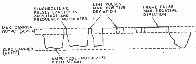
Fig. 2. It is suggested that FM could be used for the transmission of television synchronising pulses, while AM is used for the video component of the signal.
