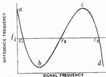
Fig. 1. Typical tracking curve for a superheterodyne receiver. The difference frequency only coincides exactly with the nominal intermediate frequency at three points.
