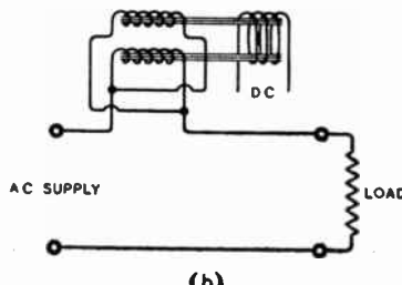
Fig. 2. Methods of eliminating AC from the DC windings of a polarised choke. (a) Separate chokes are connected in parallel with the DC windings in opposition. (b) A single winding is used for DC and the AC fluxes are in opposite phases.
