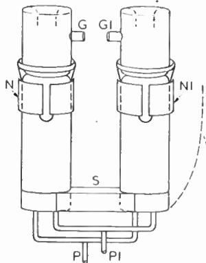
Push-pull USW generator.
