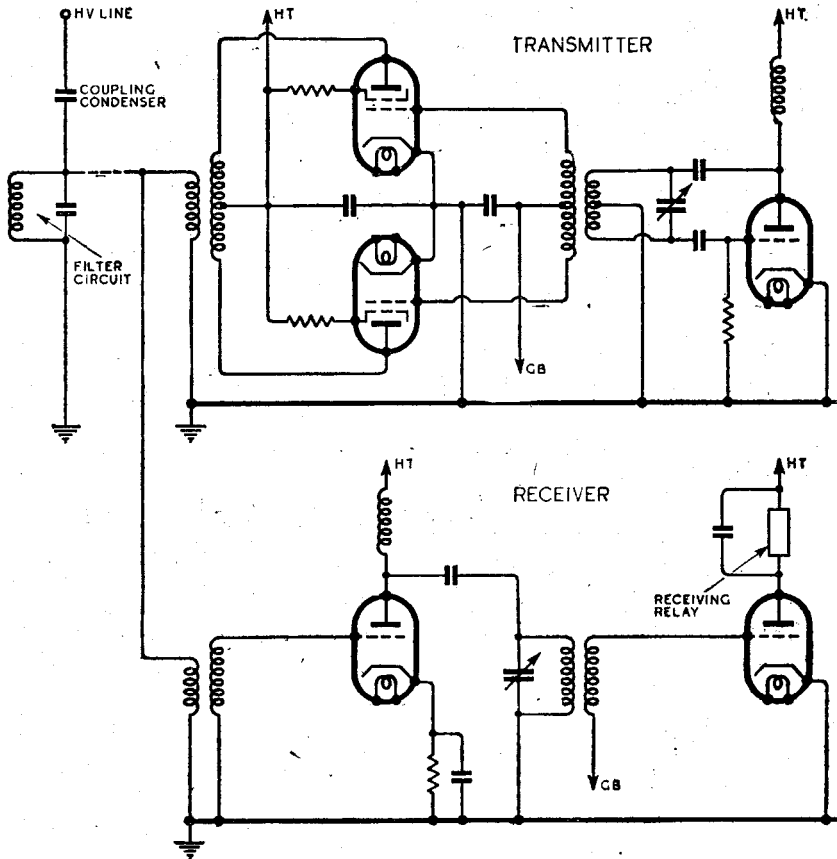
Fig. 4. Schematic diagram of a simple form of "wired wireless" transmitter and receiver.
