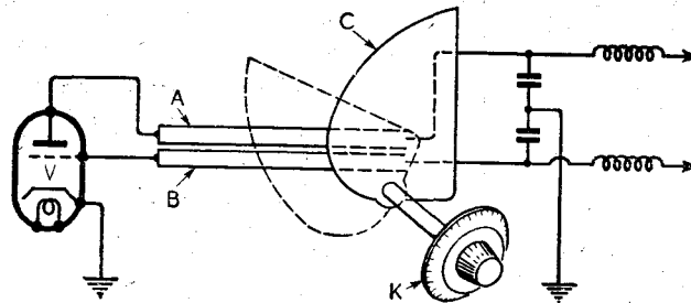
Rotary Lecher-wire tuning.
