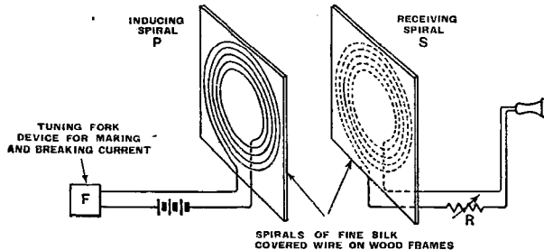
Fig. 3.—Circuit and layout of the apparatus used for the early induction experiments described in the text.
