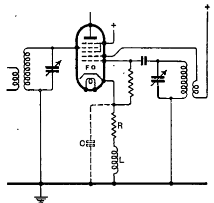
Negative feedback applied to a frequency changer.
