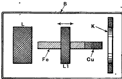
Method of tone compensation in band-pass circuits.
