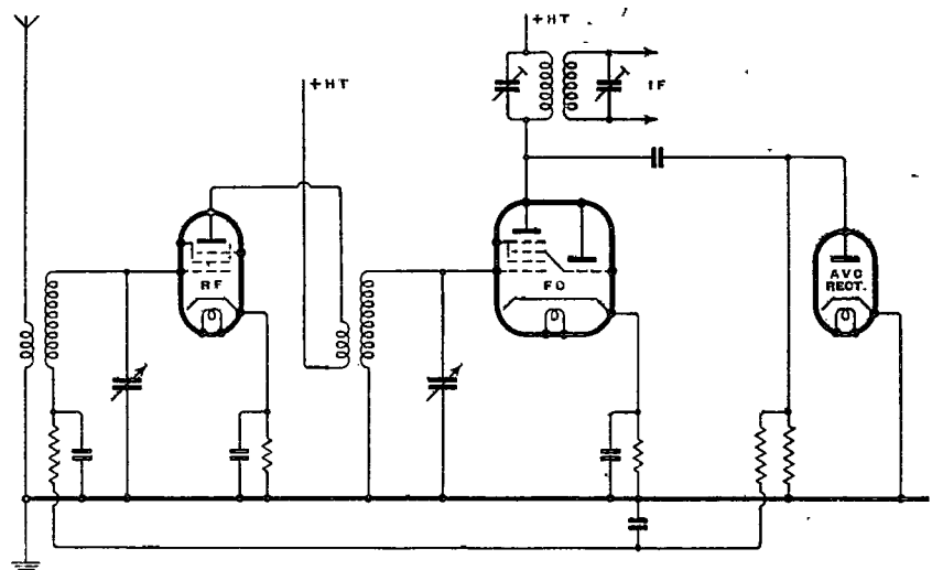
Fig. 2.—An obvious method of obtaining the RF stage AVC bias is shown here, but it is one which is unlikely to prove satisfactory.
