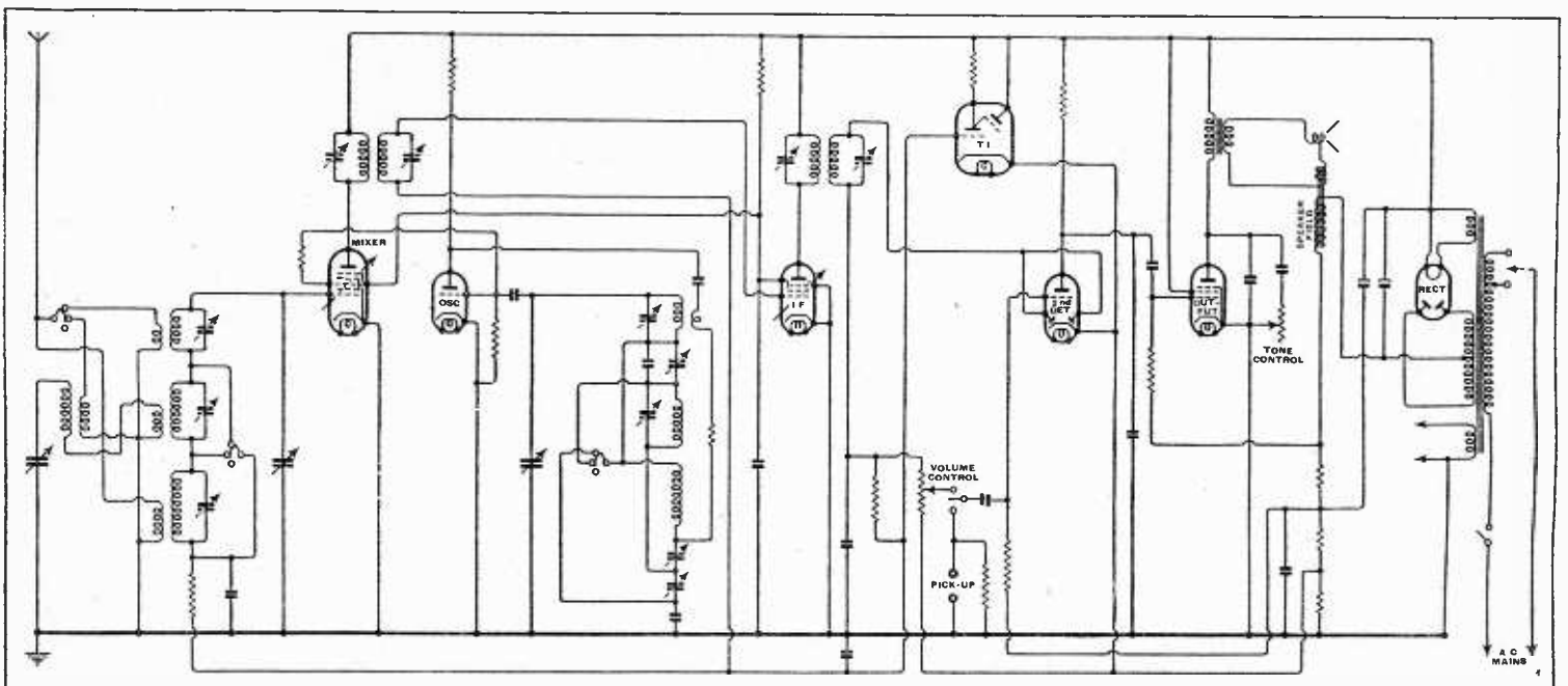
A band-pass filter is used on medium waves and single tuned circuits on the short- and long-wave ranges. Separate valves are used for the oscillator and mixing functions of the frequency-changer.
