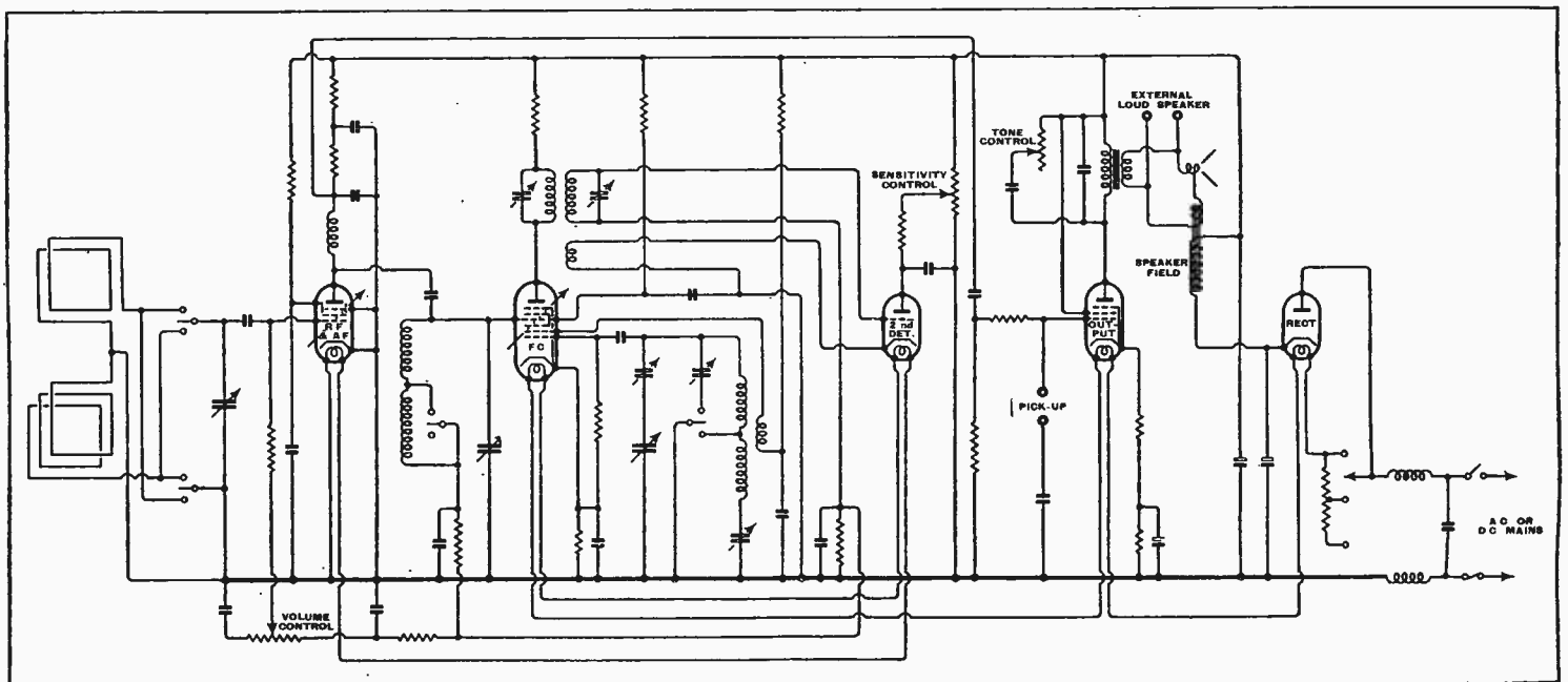
A reflexed input stage and a triode second detector arranged to give diode rectification with reaction, are unusual features of the superheterodyne circuit.
