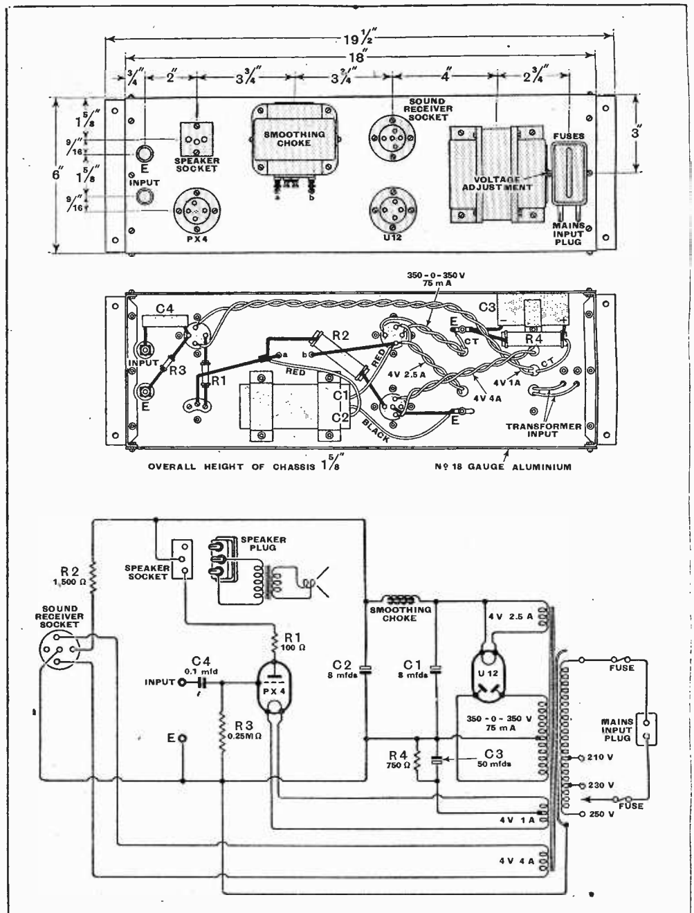
Fig. 4.—Full details are given here of a simple power unit for the sound receiver.
