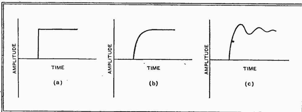
Fig. 25.—A sudden change of voltage such as that shown at (a) will be distorted in the manner depicted at (b) by an amplifier with a limited high-frequency response. With an amplifier of the type of Fig. 26, however, the output voltage may be like that of (c) if the values of components are not properly related.
