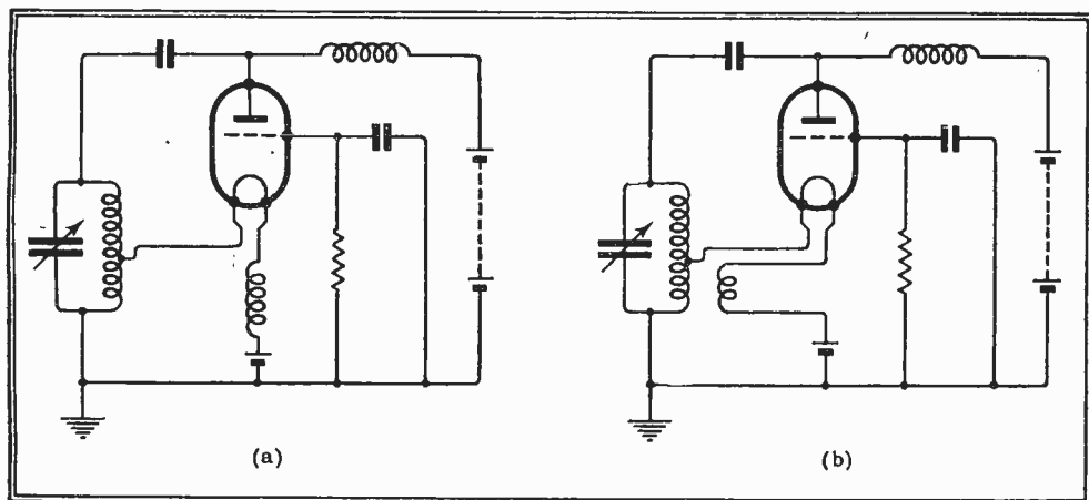
Fig. 7.—Arrangements permitting the grid end of the tuned circuit to be earthed. The filament-circuit coil in diagram (b) must be closely wound with the tuned winding.
