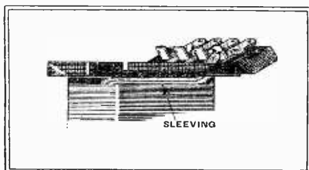
Breakdowns in output transformers are reduced to a minimum by the use of sleeving made from a transparent plastic substance for leading out the inner end of the primary winding.
