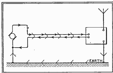
Fig. 1.—The passage of interfering impulses along supply leads.
