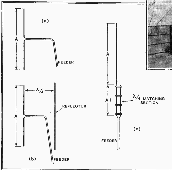
Fig. 2.—The same three aerials as shown in Fig. 1, but here depicted in theoretical form.
