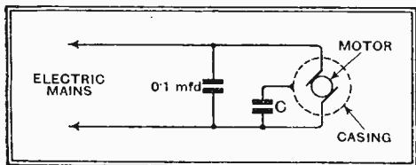
Fig. 4.—Explaining the need for caution in fitting a suppressor to a non-earthed electrical appliance.
