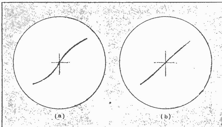
Cathode-ray figures obtained from amplifier. (a) Without degeneration, (b) with degeneration.
