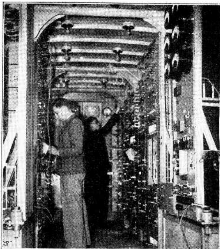
TELEVISION NERVE CENTRE. The interior of the control van which was used for the television broadcast of the Coronation Procession. At the far end of the van can be seen the two monitoring tubes on which the control engineer sees the picture as transmitted. Each tube is connected to a separate camera.
