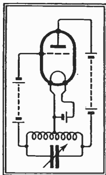
Fig. 2.—The batteries might be connected in this manner, but are "in the air."
