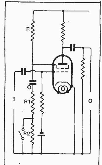
Amplifier for television signals to maintain correct phase relation in input and output circuits.
