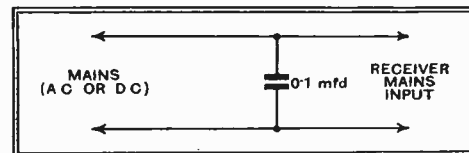
Fig. 3.—Simple suppressor circuit for the elimination of symmetrical component of mains-borne interference.
