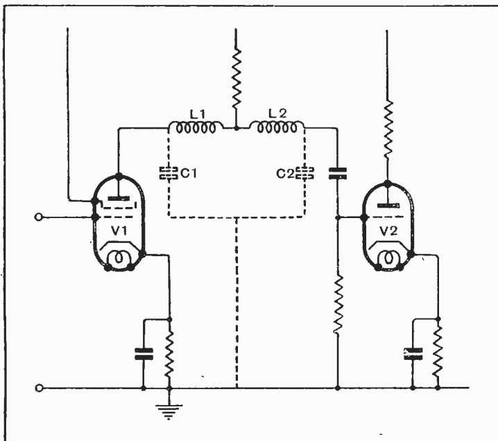
Circuit for amplifier with wide-band frequency response
