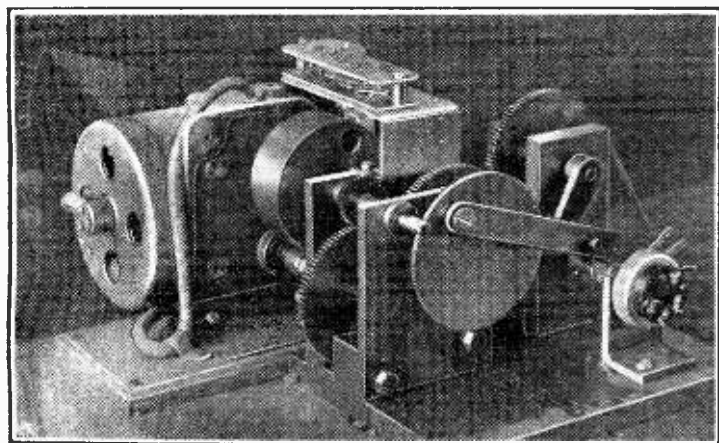
Life tests of volume controls and on-off switches are carried out with this reciprocating mechanism. The machine runs day and night and a counter at the top records the number of movements made.
