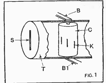
Assembly of the two cylinders in a television scanning system.
