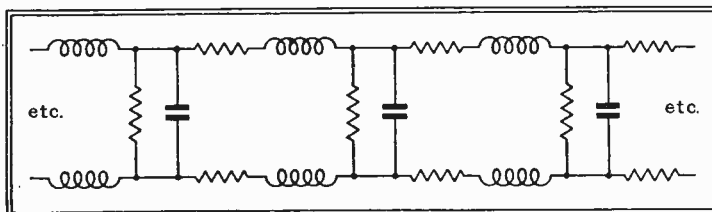
Fig. 2.—So far as their behaviour to radio-frequency currents is concerned, a pair of mains leads may be represented as in this diagram.
