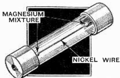
Sensitive to small sustained rises of current, the "Mag-Nickel" fuse is, nevertheless, unaffected by the surges which occur when the receiver is first switched on.
