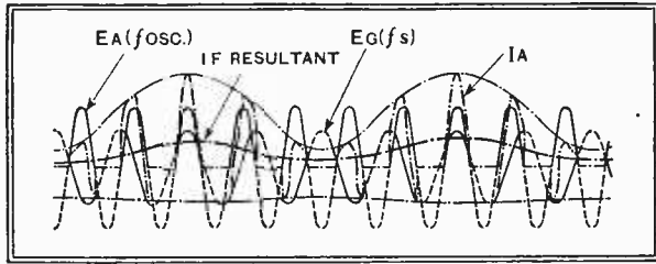
Fig. 5.—Showing additive mixing in "Ultra-dyne" circuit.
