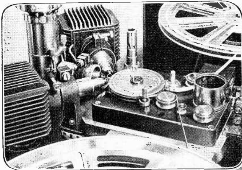
The Selenophone reproducing apparatus. Note the cooling fins on the two illuminating units between which can be seen the photo-cell tube.
