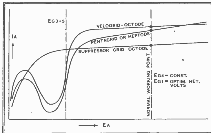
Fig. 10.—General characteristics of mixers in group a; note the higher anode impedance of the octodes.
