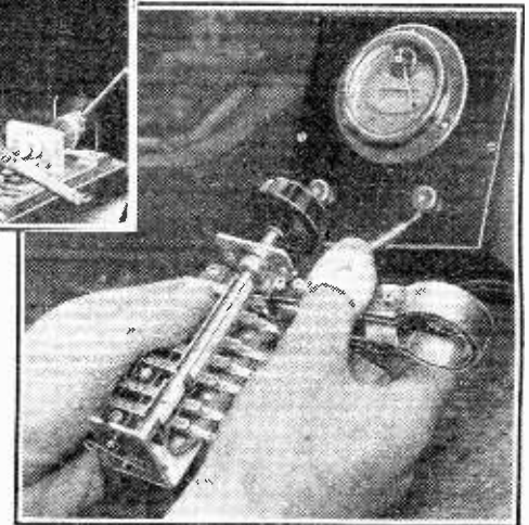
(Above) A bank of waverange switches being "run in" by a special machine. (Right) Checking contact pressure with calibrated spring tongs. Contact, which must be maintained against the opening force of the test tongs, is indicated by the meter in the background.
