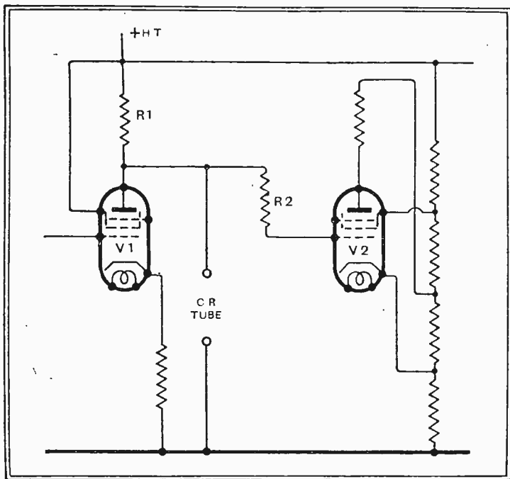
Fig. 21.—This circuit operates in a similar manner to that of Fig. 18, but is impracticable because small voltage variations in the HT supply upset the operation.
