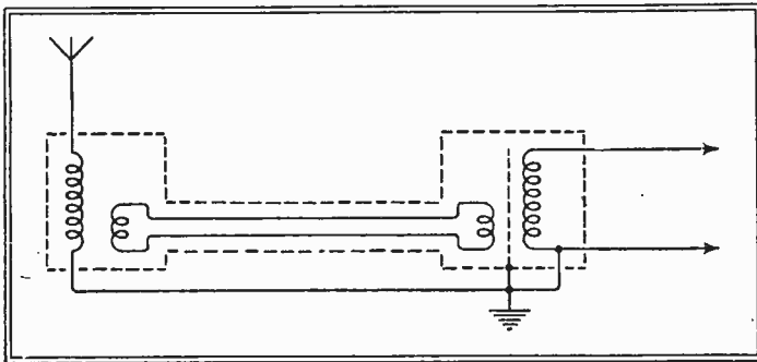
Fig. 1.—Basic anti-interference aerial circuit.
