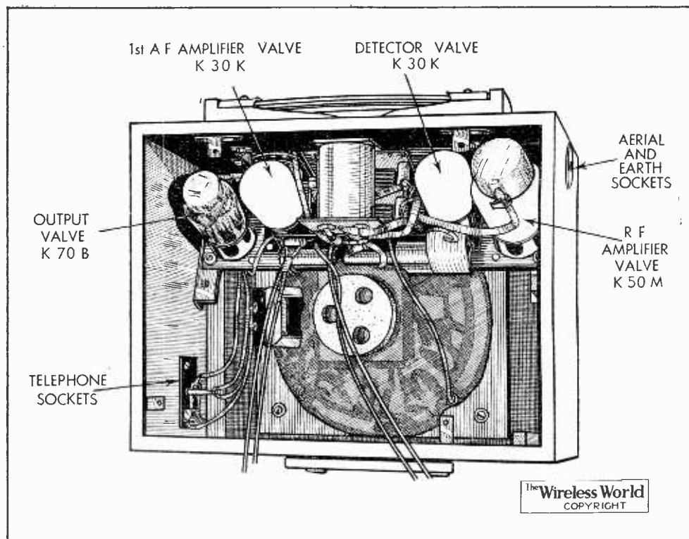
A compact receiver chassis leaves ample space for batteries of standard capacity. The frame aerial windings are incorporated in the sides of the cabinet.
