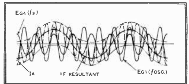
Fig. 11.—Showing IF resultant produced by multiplicative mixing without recourse to rectification.
