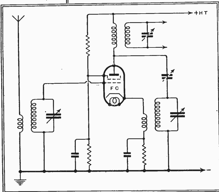
Fig. 6.—(Above). The first single-valve mixer circuit, as widely used on the Continent. Fig. 7.—(Right). Cathode injection mixer, made practicable by the introduction of the indirectly-heated SG valve.
