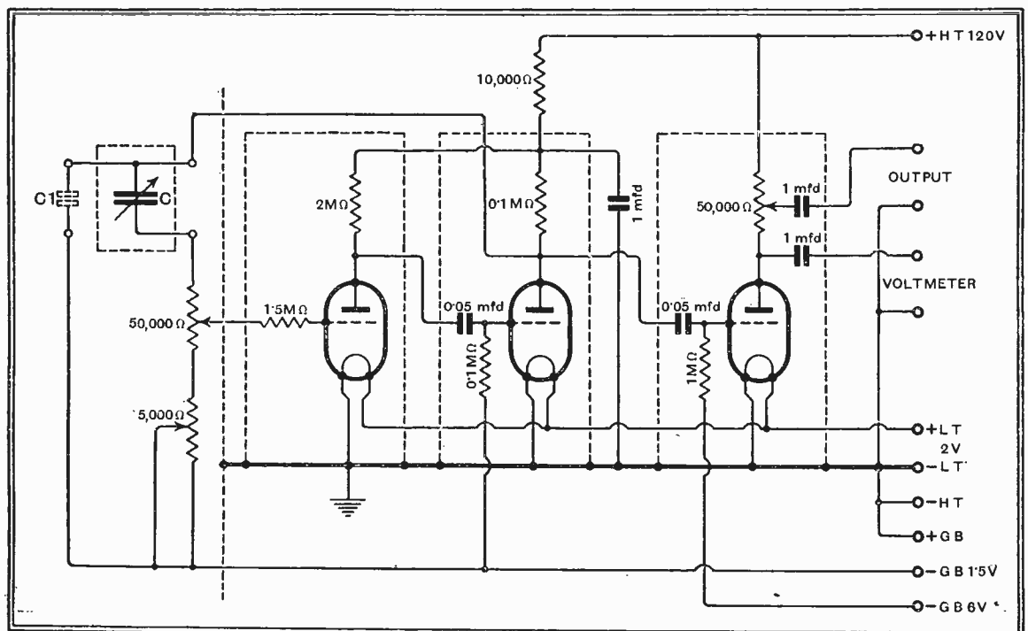
Fig. 3.—Circuit of a practical oscillator; the extra valve provides isolation between the output terminals and the oscillator proper.
