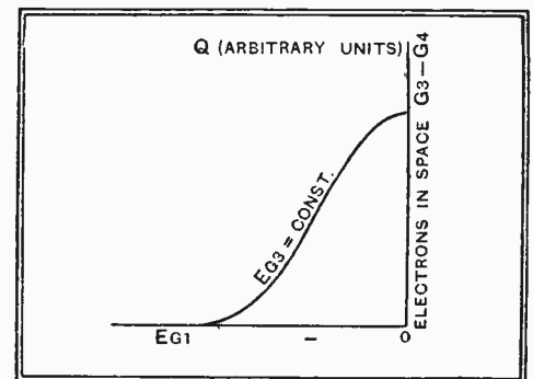
Fig. 15.—Distribution of electrons in the virtual cathode space charge as a function of the voltage on the first grid.
