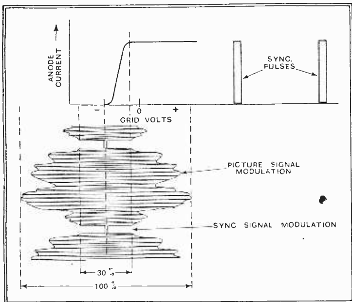
Fig. 18.—The operation of an amplitude filter operating on the modulated carrier is shown here, and it is readily seen how only the sync pulses can affect the output.
