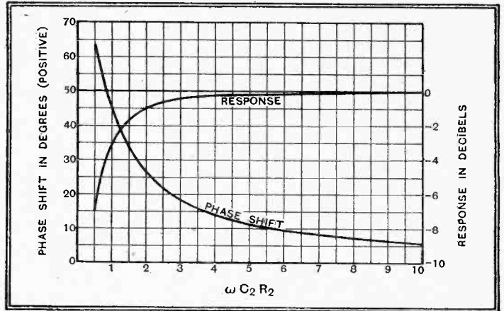
Fig. 29.—The response and phase shift at low frequencies caused by the coupling condenser C_2 and grid leak R_2 are shown here.
