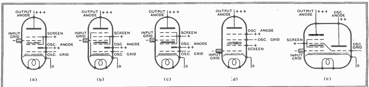
Fig. 9.—Showing relative potentials and functions of pentagrids (heptodes), suppressor grid octodes, velogrid octodes and hexodes. Shaded areas indicate space charges; the normal cathode space charge occupies the area nearest the cathode, while the area between the first positive screening grid and the second negative control grid comprises the virtual cathode space charge.
