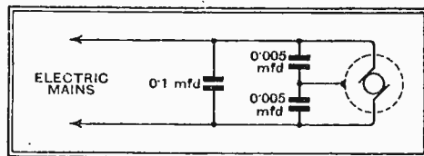
Fig. 5.—Another method of suppressing interference from a device of which the metallic casing (dotted lines) is unearthed.
