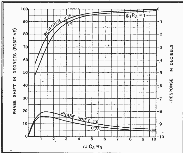
Fig. 30.—These curves show the effect of the bias resistance R_3 and its by-pass condenser C_3 .
