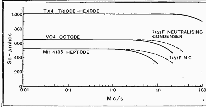
Fig. 12.—Variation of conversion conductance with frequency, showing beneficial effect of neutralising condenser between points X and Y (see Fig. 13).
