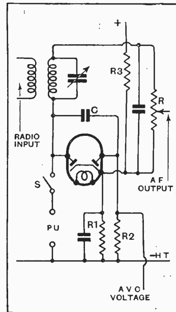
Circuit arrangement when a volume control common to radio and gramophone is used.
