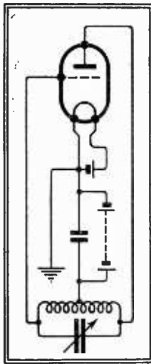
(Below) Fig. 3.— Full HT voltage on the grid—clearly an inadmissible state of affairs.
