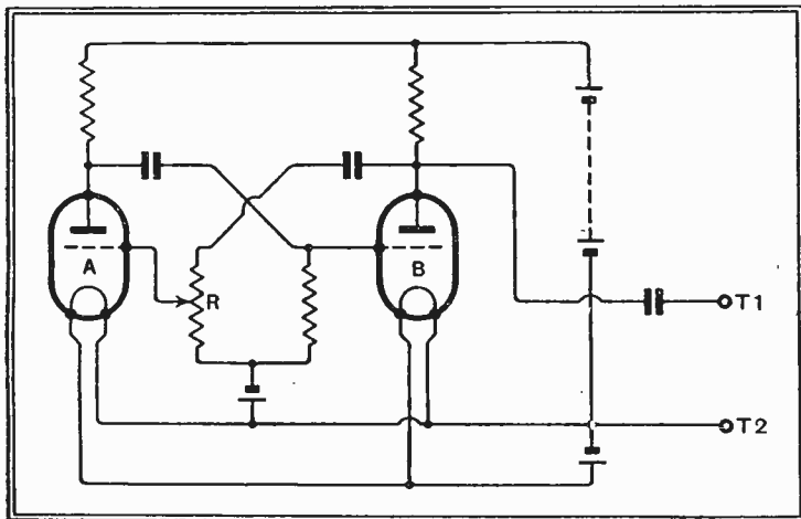
Fig. 1.—The simple "multi-vibrator" generator.
