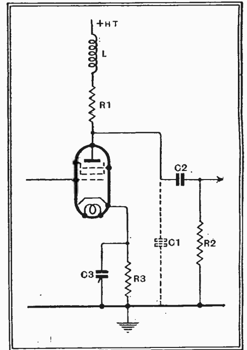
Fig. 26.—A typical VF stage is shown here. The condenser C1 represents the stray capacity.
