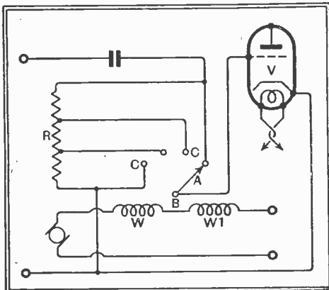
Volume according to the speed: novel application of AVC to a car radio receiver.
