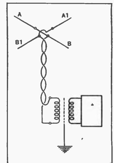
Aerial designed for efficient reception over a wide band of short-waves.
