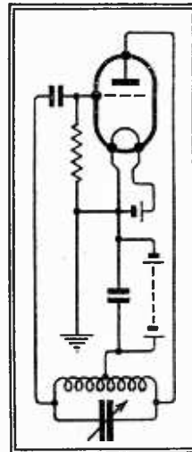
Fig. 4.—The series-fed Hartley circuit; this and succeeding diagrams show practical working arrangements.
