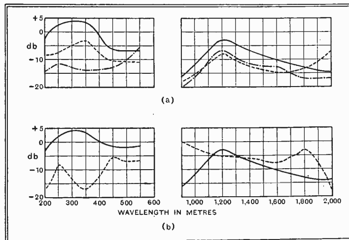
Fig. 3.—Diagram (a) shows losses introduced by the same screened aerial equipment into different broadcast receivers, while diagram (b) shows losses introduced by different screened aerials into the same receiver.
