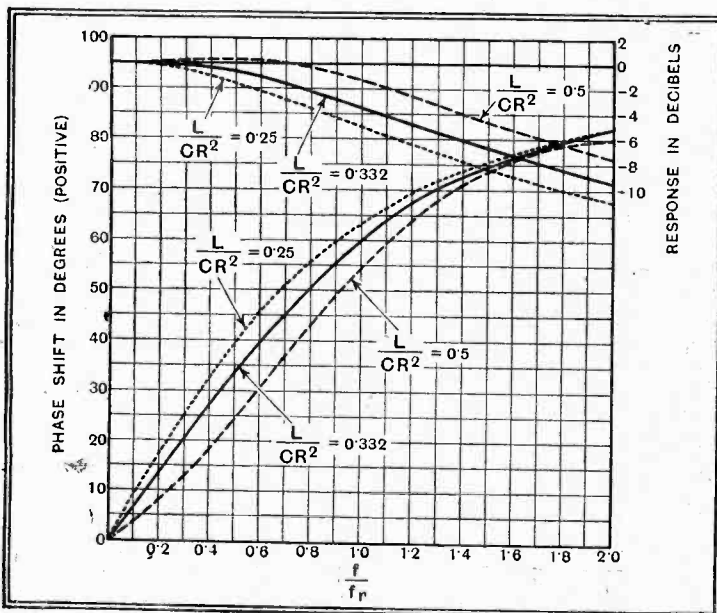
Fig. 27. — These curves show the frequency response and phase shift for the amplifier of Fig. 26 for three values of L/CR^2 . The frequency scale is expressed in frequency ratios so that the curves are of universal application.
