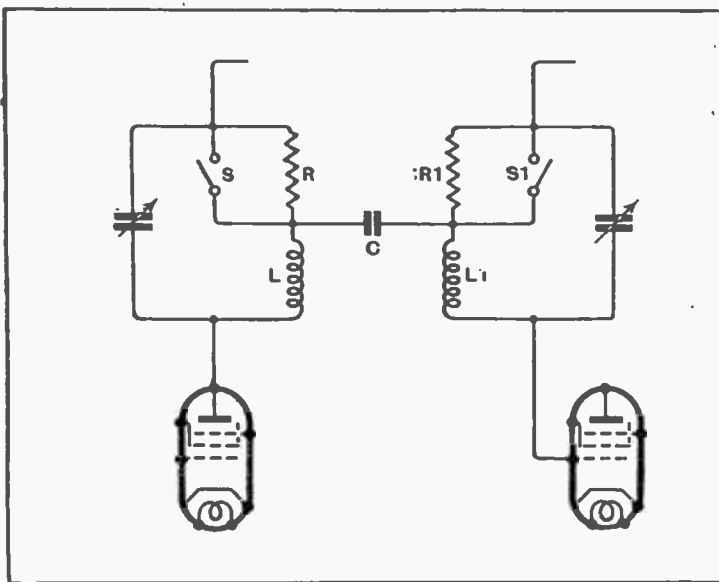
Variable selectivity circuit for superhet IF amplifiers.
