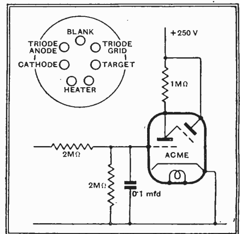
Base connections and circuit for using the ACME indicator.
