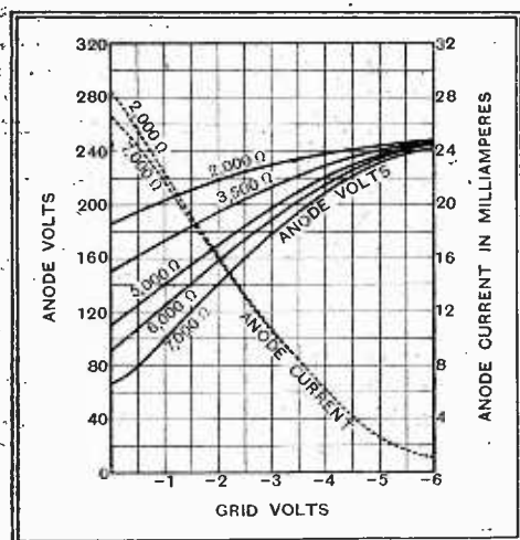
Fig. 31.—Dynamic grid volts—anode-volts curves of the TSP4 are given here.
