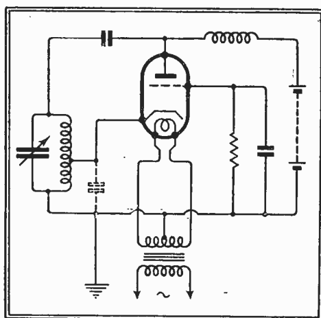
Fig. 9.—The filament choke may be avoided by using an indirectly heated valve.
