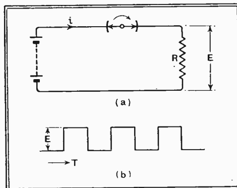
Fig. 1.—Artificially generated interference: operation of the rotary switch in diagram (a) produces a square-topped wave form represented by curve (b).
