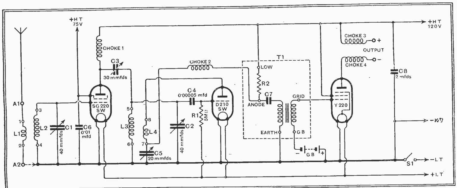
Fig. 1.—Theoretical circuit diagram of the ultra-short wave receiver.
