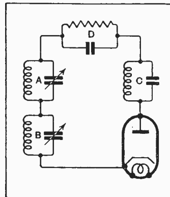
Non-radiating first detector stage for a superheterodyne receiver
