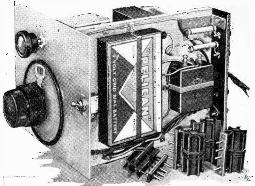
The grid battery, telephone RF chokes, condenser C8, filament and HT wiring are all accommodated below the base-board.
