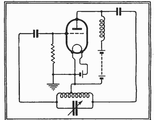
Fig. 5.—The parallel-fed arrangement.
