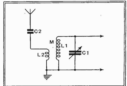
Fig. 2.—Aerial input circuit of a typical receiver ; there is no standardisation of the various constants.
