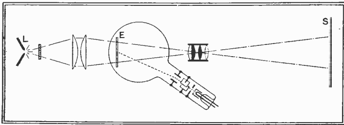
Using a cathode-ray tube for controlling a beam of light from an external source.
