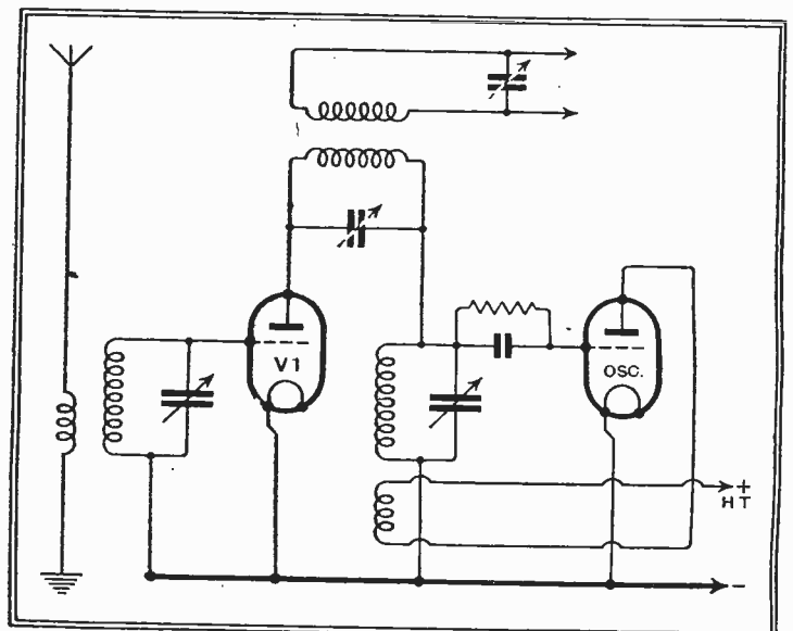
Fig. 4.—“Ultra-dyne” circuit in which V1 is not a grid detector, but virtually an RF amplifier with anode rectification of the oscillator voltage, which is applied in place of the usual steady HT voltage.
