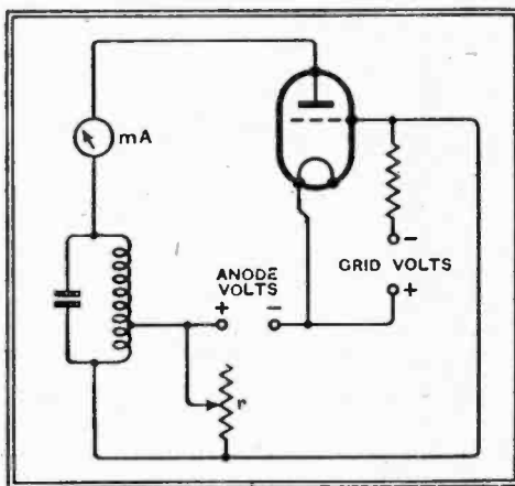
Fig. 12.—A simple form of valve tester, giving direct readings of mutual conductance, based on the information given on the curve sheet, Fig. 11.
