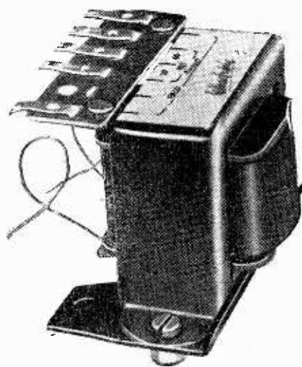
Wharfedale three-ratio replacement output transformer.
