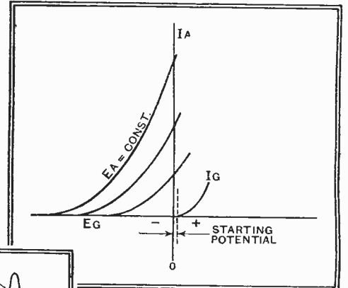
Fig. 3.—The starting potential in early valves was generally in the positive region of grid potentials.
