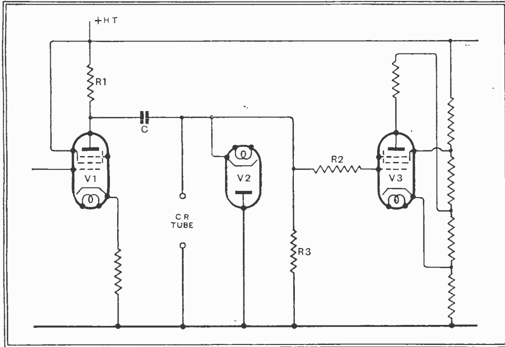
Fig. 24.—In this circuit the DC component is lost because of the condenser C, but is restored artificially by the diode V2. This arrangement is quite practicable and gives very good synchronising.
