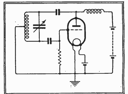
Fig. 6.—The popular parallel-fed Hartley circuit in more recognisable form.
