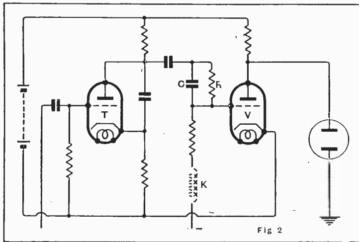
Fig. 2.—Frequency compensated amplifier for television scanning circuit.
