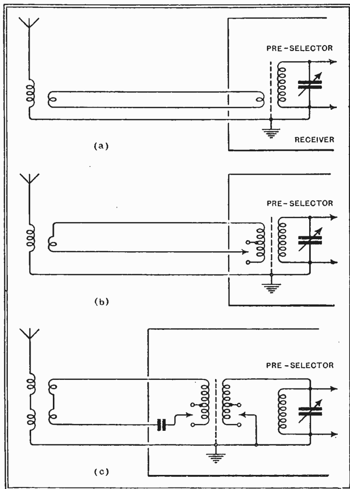
Fig. 5.—Illustrating the use of the receiver input circuit in place of the usual "set transformer" of the normal screened aerial equipment.
