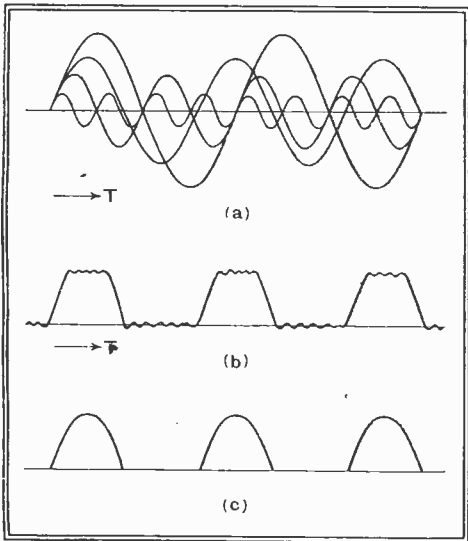
Fig. 2.—From the point of view of interference, the simple square-topped wave form of Fig. 1 (b) may be replaced by the complex curves of diagrams (a) and (b). The rounded wave form of diagram (c) would cause interference mainly with long-wave reception.
