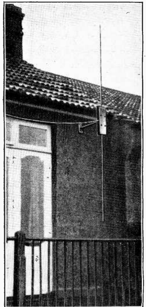
TELEVISION AERIAL. A practical interpretation of a di-pole television aerial with centre-connected feeder as shown in Fig. 1(a) on page 506 of this issue.
