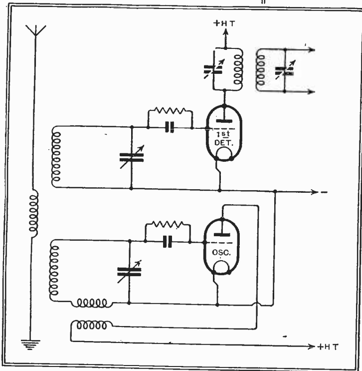
Fig. 1.—The classical frequency-changing circuit.
