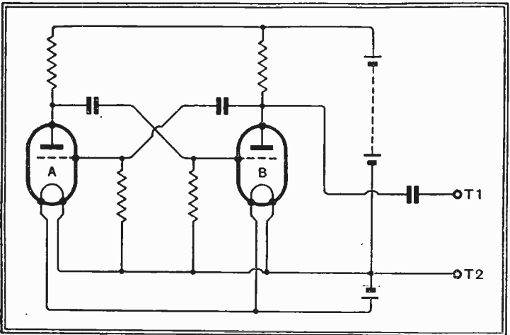
Fig. 2.—A multi-vibrator circuit giving an output of better wave form.
