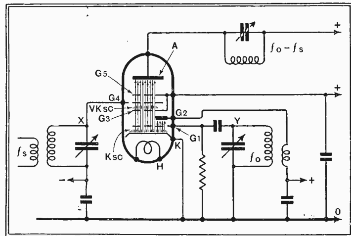
Fig. 13.—Showing the virtual cathode space charge between first positive screen and second control grid. The oscillator frequency is transferred to G_4 by virtue of influence.
