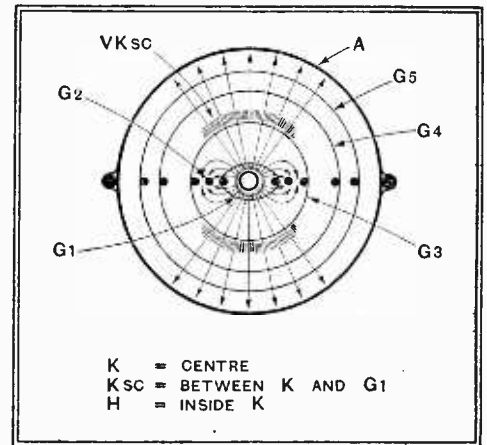
Fig. 14.—Representation of a section through a heptode.
