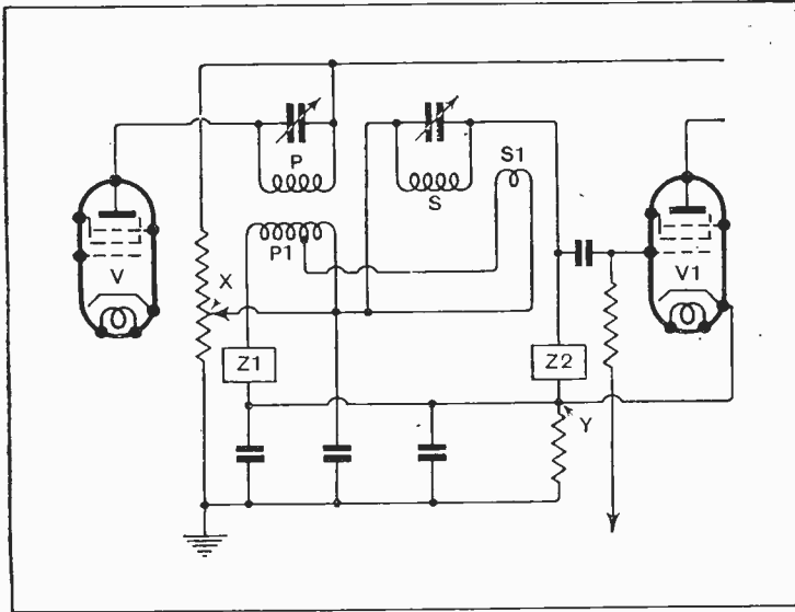
Circuit arrangement for automatic selectivity control.
