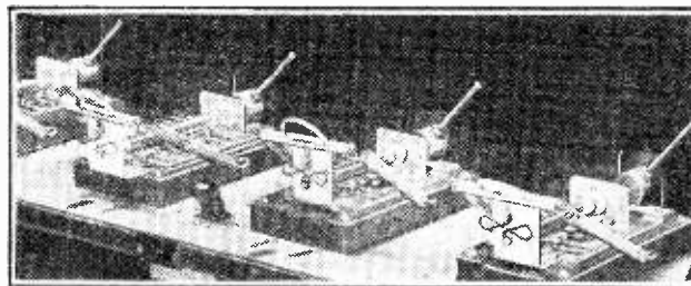
(Above) A bank of waverange switches being "run in" by a special machine. (Right) Checking contact pressure with calibrated spring tongs. Contact, which must be maintained against the opening force of the test tongs, is indicated by the meter in the background.
