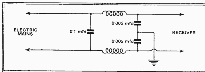
Fig. 6.—A choke-condenser filter applicable to general use.
