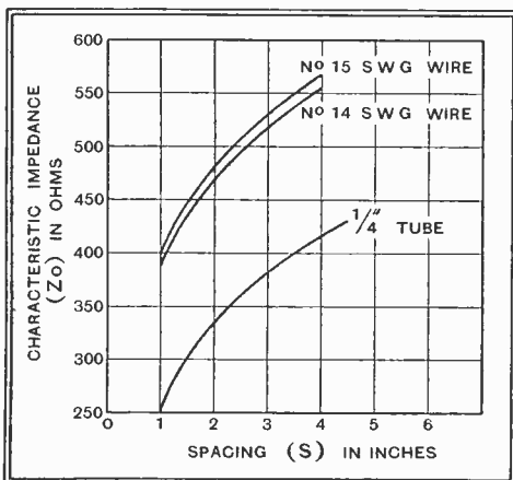
Fig. 4.—The characteristic impedance of quarter-wave matching transformers using wires or tube of the sizes given here and with different spacings between conductors can be obtained from these curves.
