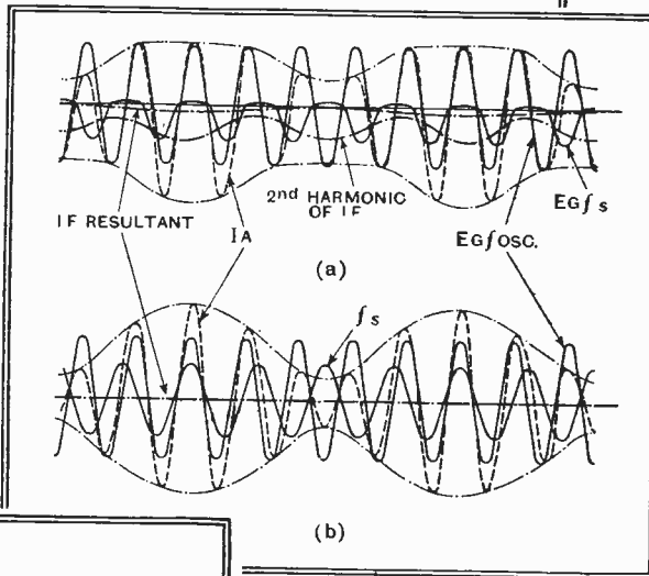
Fig. 2.—Diagram (a) shows additive mixing in grid-rectifying 1st detector; no beat-frequency is produced by additive mixing when rectification is absent as in diagram (b).
