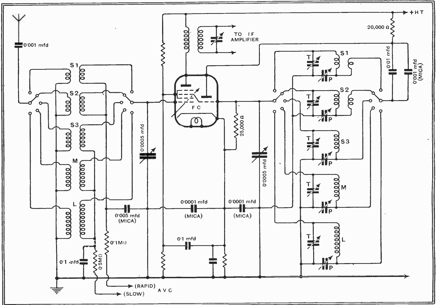
Fig. 16.—A modern frequency-changing circuit for a five-waveband receiver. The non-inductive properties of the mica condensers as shown are important on the shorter wavebands.
