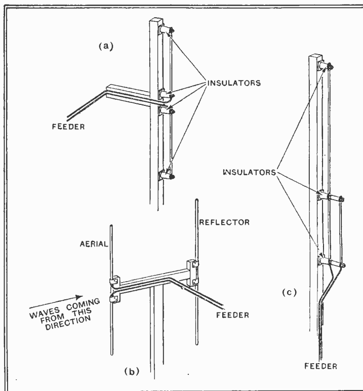
Fig. 1.—Three popular di-pole aerial systems. In (a) a low-impedance feeder is joined to the centre of the aerial. Sometimes a reflector is used when the aerial takes the form shown in (b). The feeder can be joined to one end by adding an impedance matching section as shown in (c).
