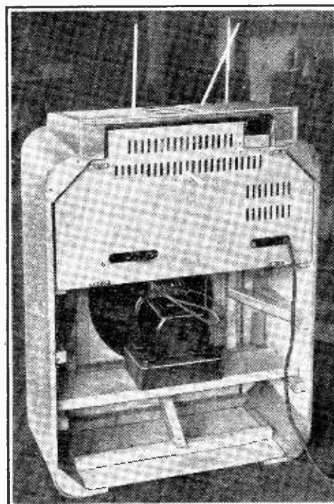
Testing an experimental layout in one of the latest console cabinets for heat distribution. The thermometers indicate the temperature in the vicinity of the oscillator coils, the gang condenser, the electrolytic smoothing condensers and the mains transformer.
