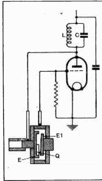
Method of mounting a piezo-electric crystal to "wobble" the frequency of a master oscillator stage.
