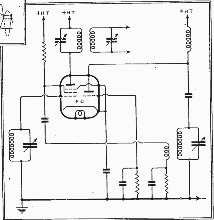
Fig. 8.—Cathode-coupled circuit with triode-pentode valve.
