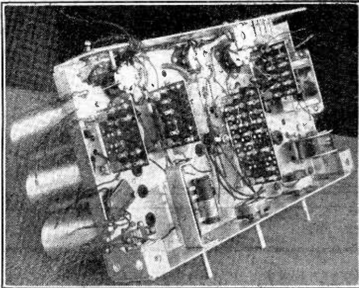
Underside of chassis in course of wiring, showing liberal use of sub-assembly panels. Note paper washers under soldered joints on valveholders near top edge of chassis.
