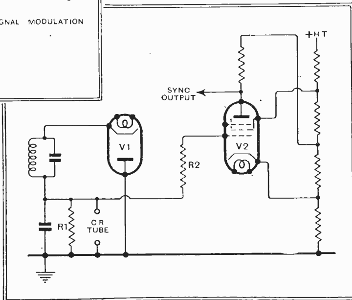
Fig. 19.—Sync separation can be carried out on the VF signal across the diode load resistance R1; the separator valve is V2.
