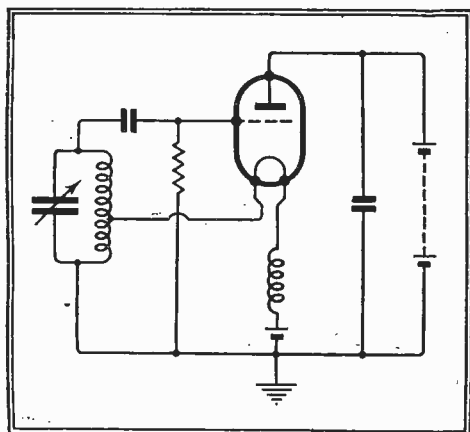
Fig. 8.—Earthing the anode end of the tuned circuit.
