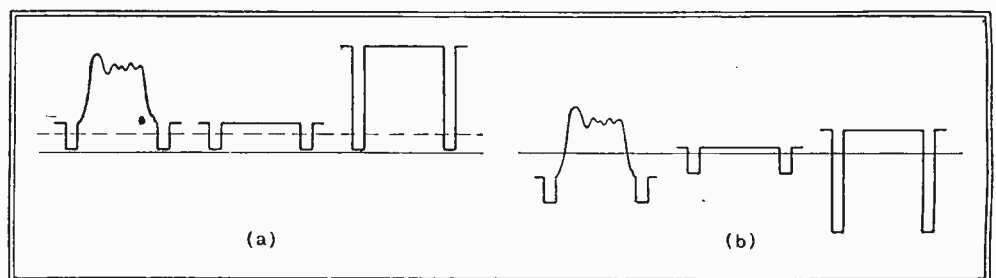
Fig. 23.—Three typical signals are shown at (a), the first corresponding to a normal line, the second to a black line, and the third to a white line. The same signals are shown at (b) with the DC component removed.
