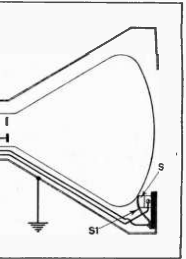
Automatic voltage cut-out for cathode-ray tubes.
