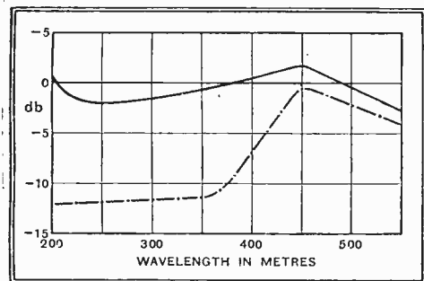
Fig. 4.—The full line shows losses introduced by a transformer system into the receiver for which it was designed; the dash-dot line represents losses with another set.
