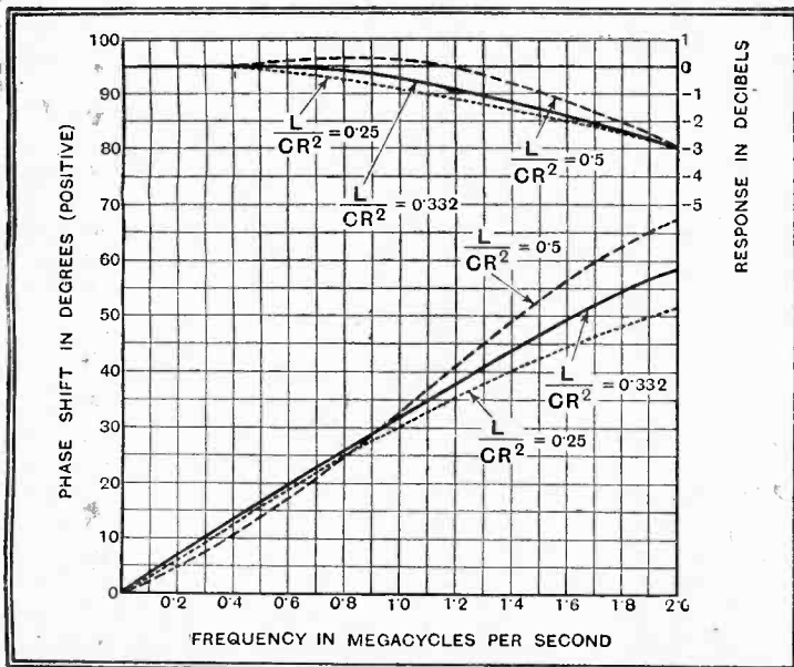
Fig. 28.—These curves are the same as those of Fig. 27, but with a frequency scale and resonance frequencies such that the response at 2.0 Mc/s is -3.0 db.
