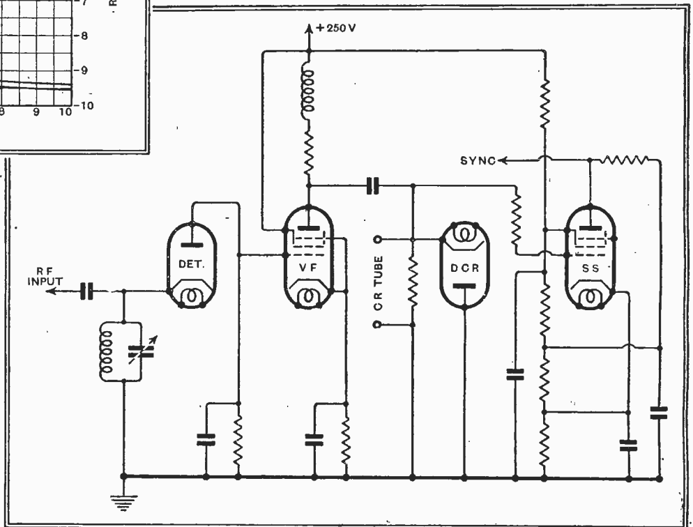
Fig. 32.—The complete circuit of the end of a television receiver showing the detector, VF amplifier, DC restorer, and sync separator.
