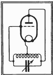
(Below) Fig. 1.— The Hartley oscillator in its simplest possible form.
