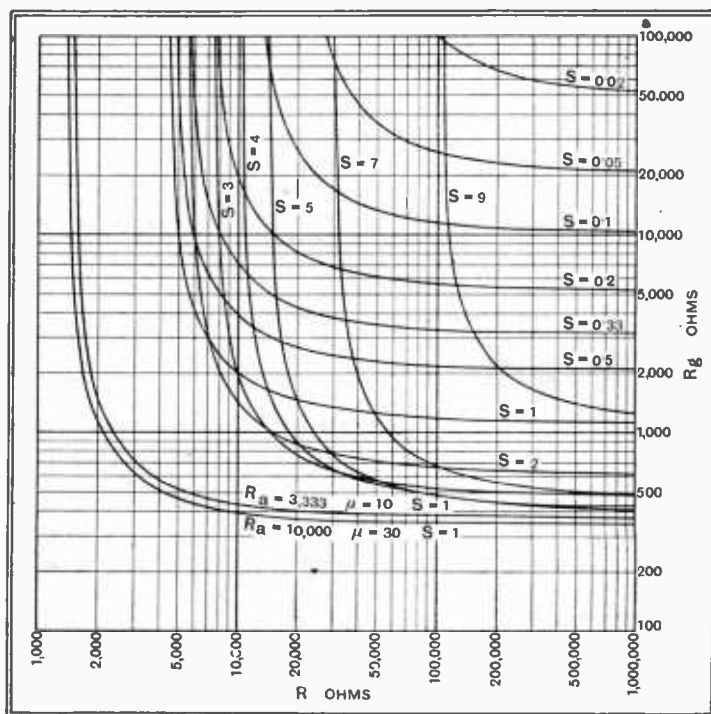
Fig. 11.—Diagram from which the best tapping point on the oscillator coil can be determined for various conditions. Other uses of the curves are explained, and still others can easily be thought of.
