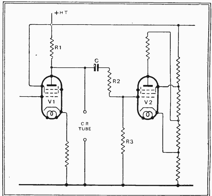
Fig. 22.—This circuit is the same as that of Fig. 21 save for the insertion of the condenser C. This removes the trouble of inconsistent operation, but proper synchronisation cannot be obtained because the condenser removes the DC component of the signal.
