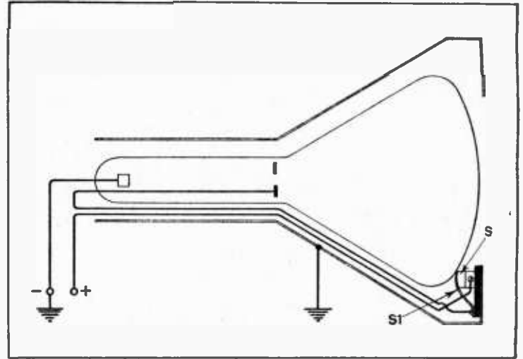
Automatic voltage cut-out for cathode-ray tubes.
