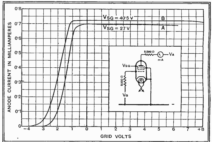
Fig. 9.—The characteristics of the Cossor MS Pen measured under the conditions indicated are shown here. For good operation at V_{SG} = 27 volts, the input should not be less than 10 volts peak on 100 per cent. modulation.
