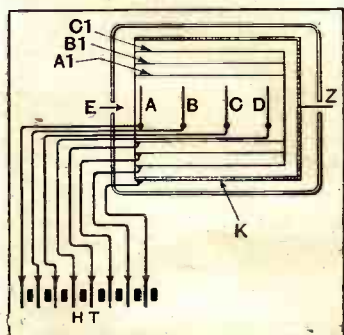
Electrode assembly in the cold cathode-ray-type amplifying valve.
