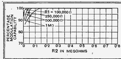
Fig. 11.—The modulation capability of the detector is shown here for the case when R1 is centre-tapped to feed R2 through C2.
