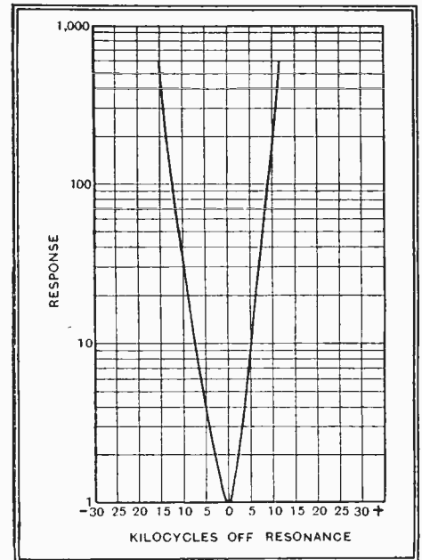
Fig. 3. Frequency response of the two IF stages including the eight tuned circuits. The intermediate frequency is 465 kc/s.
