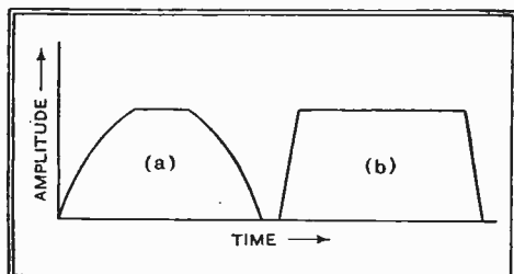
Fig. 8.—When the picture amplitude is small, a single IF half-cycle takes the form of (a) in the synch. separator, but when it is large it is more like (b). This results in the vision signal having some effect on the synchronisation.
