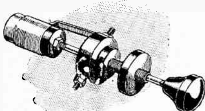
This "on and off" switch avoids applying maximum filament potential in the process of switching on. The filament current is slowly brought up to the correct value without adjusting the setting of the filament rheostats
