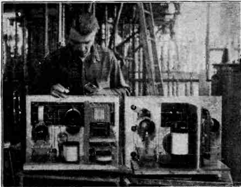
CRYSTAL TRANSMITTING CONTROL. An engineer at WGY, Schenectady, holding the piece of quartz crystal, less than an inch square and barely 1/8 in. thick, which controls the 50 kilowatt output of the famous station. The crystal maintains the frequency at exactly 790 kilocycles.
