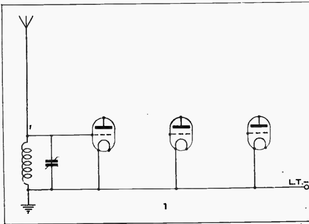
H.F., detector and L.F. amplifying valves. A tuned oscillatory circuit, with aerial and earth, is connected between grid and filament of the first (H.F.) valve. For the sake of simplicity, the complete filament circuits have been omitted.
