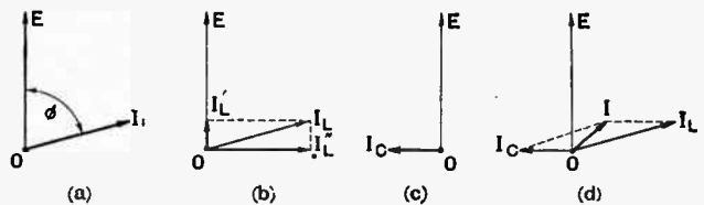
Fig. 2.—Vector diagrams (a) and (b) for the inductive branch of the circuits in Fig. 1; (c) for the condenser branch, and (d) for the complete circuit
