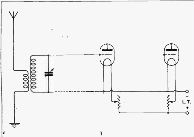
The conventional arrangement of two valves, with normal filament connections. The secondary of an "untuned aerial" coupler is connected across the grid and filament of the first valve, which has in its anode circuit—
