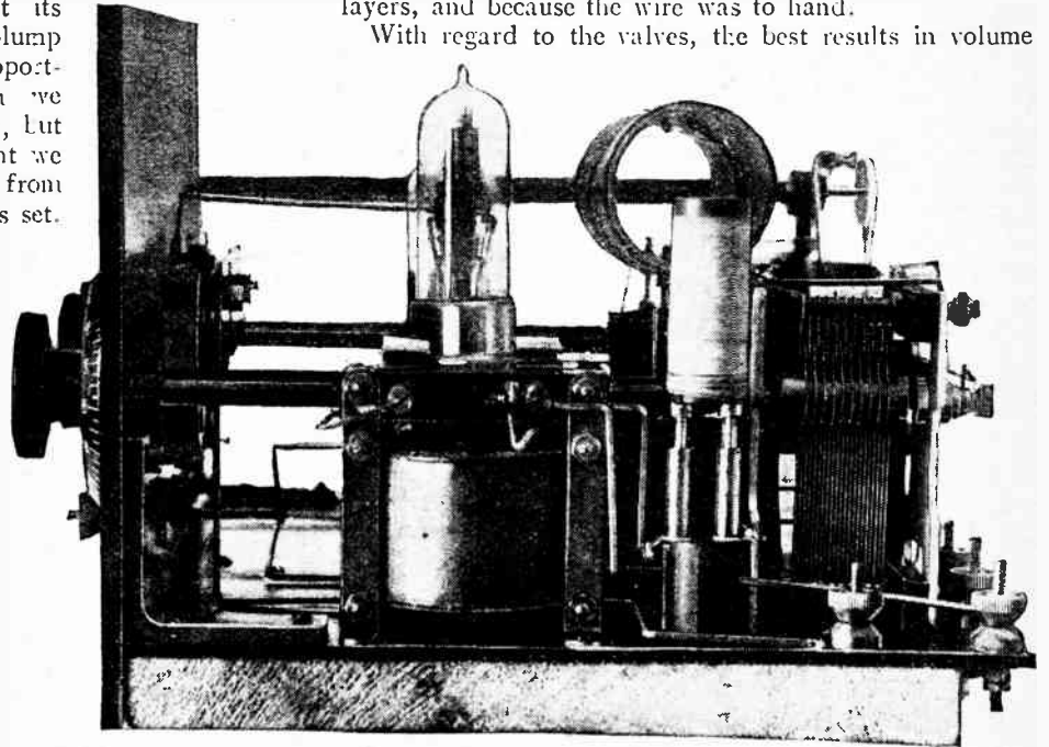
End view, showing one of the H.F. chokes.
