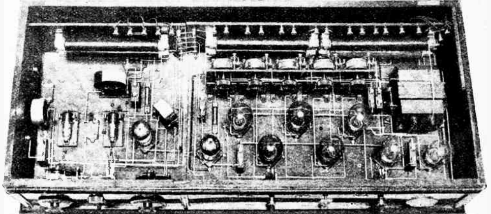
A HOSPITAL SET. An eleven-valve instrument presented to the King's College Hospital, Denmark Hill, by the "Daily News" Hospital Wireless Fund. It will be seen that the set embodies two portions, the first consisting of a H.F. and Detector Unit with optional L.F. resistance capacity coupled amplifier, and the second comprising an eight-valve amplifier. It was constructed by the Oxford Wireless Telegraphy Co., Ltd.
