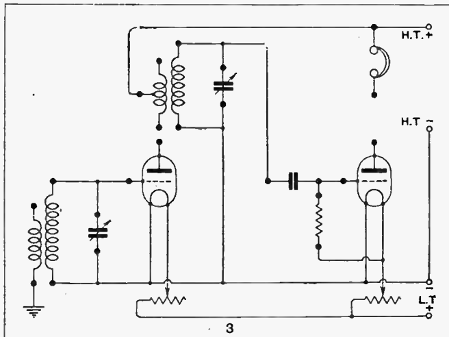
The high-potential sections of the first and second grid circuits are connected up.
