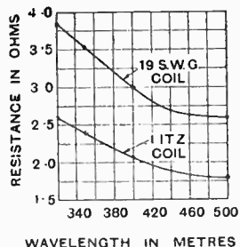
Variation of the H.F. resistance with wavelength and frequency.
