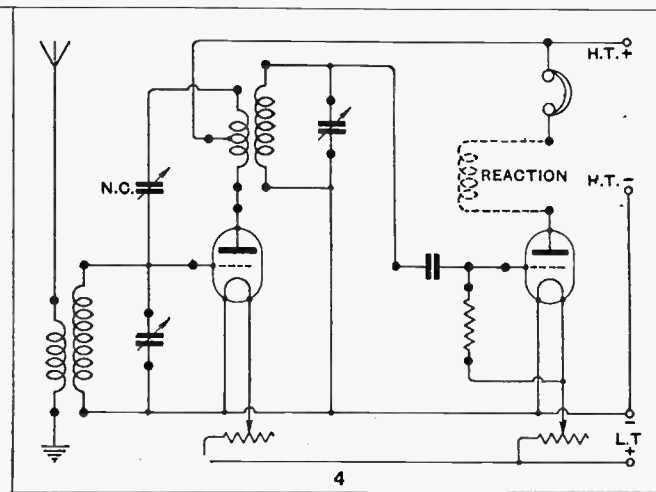
The plate circuits of both valves are completed. Aerial and neutralising connections are added.
