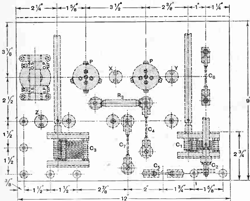
Fig. 2.—Layout of components on the baseboard, which is cut from 1/8in. ebonite sheet. The ebonite base is screwed to a wooden baseboard 12in. x 9in., leaving 1in. overhanging at the back for the terminals.
