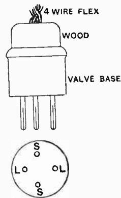
Fig. 9.—Connections of the valve base adaptor.
