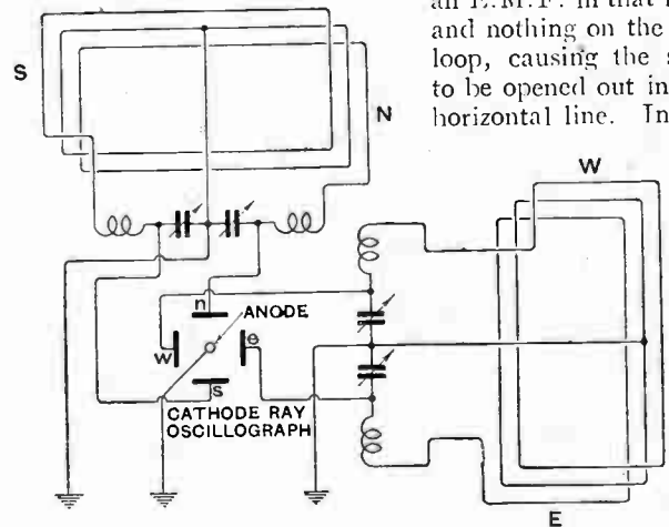
Fig. 1.—Directional frame aerials connected directly to the oscillograph for recording strong atmospherics.
