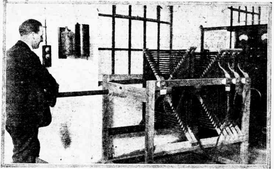
Another form of variometer used in the aerial tuning circuit.
