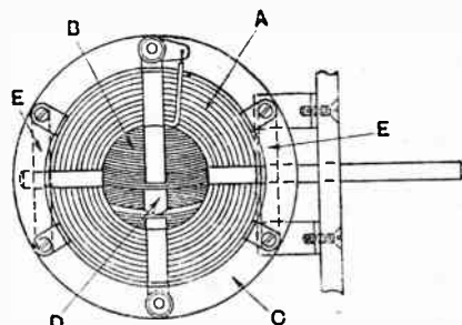
Variometer construction. (No. 244,879.)
