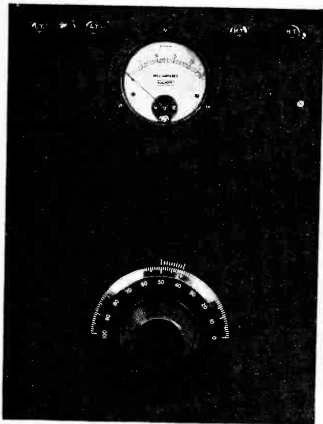
The front panel has a clean appearance owing to the absence of screw heads. The components, which are attached to the underside, are light in weight and are secured in position by means of screws and blind holes. The two screws in the top right-hand corner may be blued or treated with camera black to render them less conspicuous.
