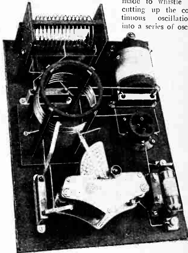
The components are arranged so that connecting up is carried out by means of short direct leads, an important feature in wavemeter design.
