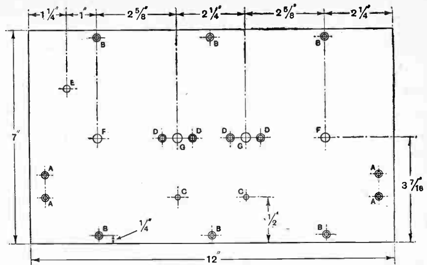
Fig. 3.—Drilling details of the front panel. Sizes of holes are as follow: A, 1/8in. dia., countersunk for No. 6 B.A. screws; B, 1/8in. dia., countersunk for No. 4 wood screws; C, 5/32in. dia.; D, 5/32in. dia., countersunk for No. 4 B.A. screws; E, 7/32in. dia.; F, 9/32in. dia.; G, 5/16in. dia.
