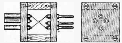
Valve adaptor to prevent filament sag.
