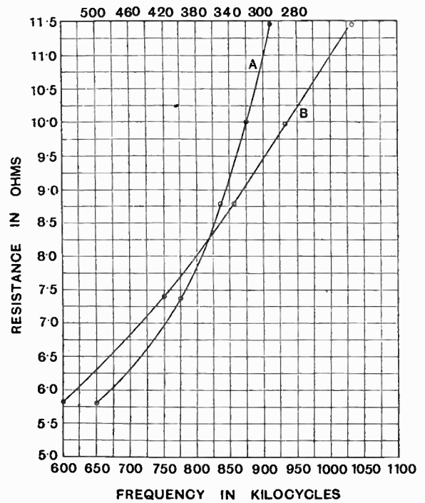
Curves for the Toroidal coil, curve A showing the variation of H.F. resistance with wavelength, and B, with frequency.
