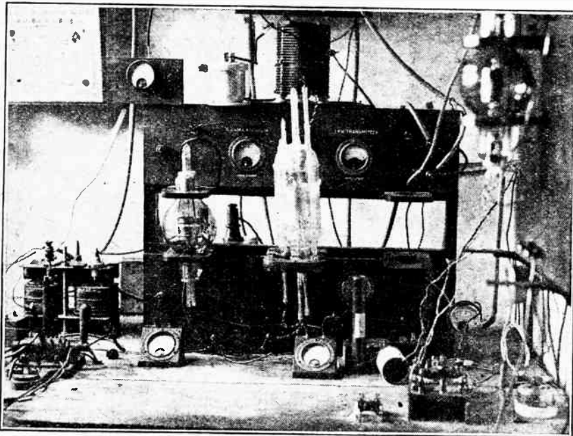
PROGRESS AT 2NM.—Mr. Gerald Marcuse avails himself of his well-earned facilities in regard to the use of high power for world wide telephony tests. This recent photograph shows the installation of a Mullard 1-kW. valve.
