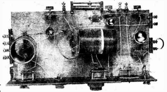
Layout of components in the experimental receiver. The various components will be readily identified with the symbols of the circuit in Fig. 2.
