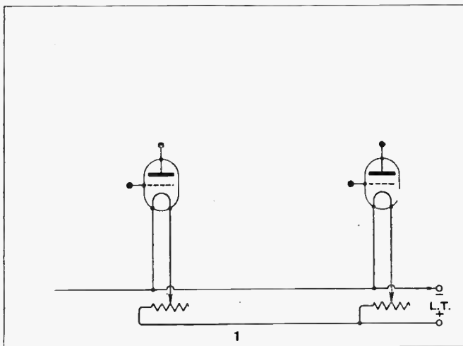
The filament circuits are completed in the usual manner. All these are low potential wires, and may be run close together.
