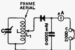
Fig. 5.—Frame aerial circuit with which the curves of Figs. 6, 7 and 8 were obtained.
