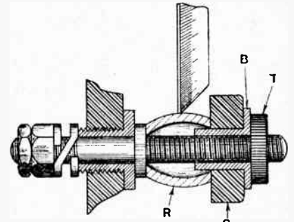
Improvised vernier movement.
