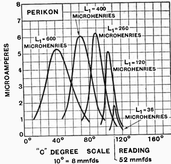
Fig. 8.—Tuning curves obtained with Perikon with various values of L_1 (frame circuit).
