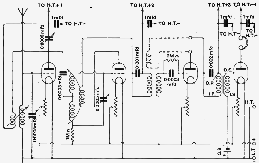
Fig. 1.—Four valve circuit giving very high selectivity.
