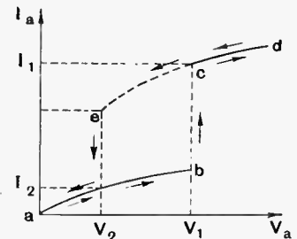
Fig. 4.—Characteristic curve of the valve in Fig. 3.
