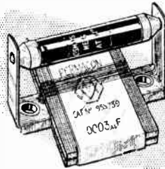
The Cosmos Permacon grid condenser and leak.
