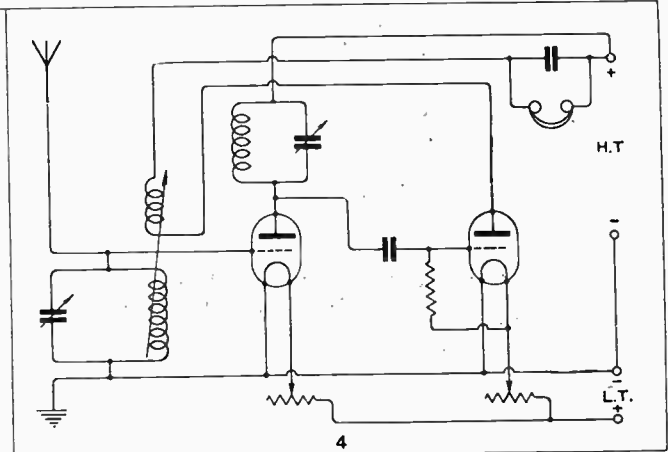
The addition of the grid leads (also a high potential), completes the receiver.
