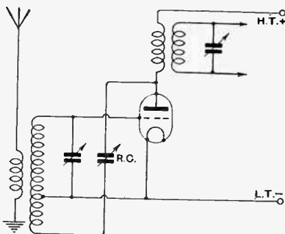
Fig. 2.—Capacity reaction.
