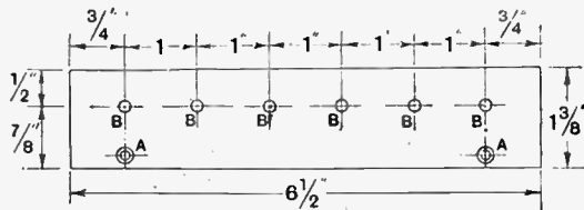
Fig. 10.—The terminal panel A, 5/32in. dia.; B, 1/8in. dia countersunk.
