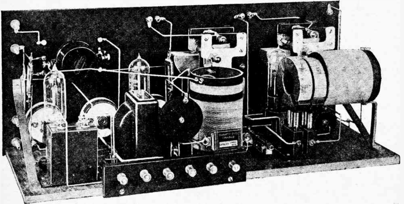
The receiver adapted for long-wave reception with loading and reaction coils in position.
