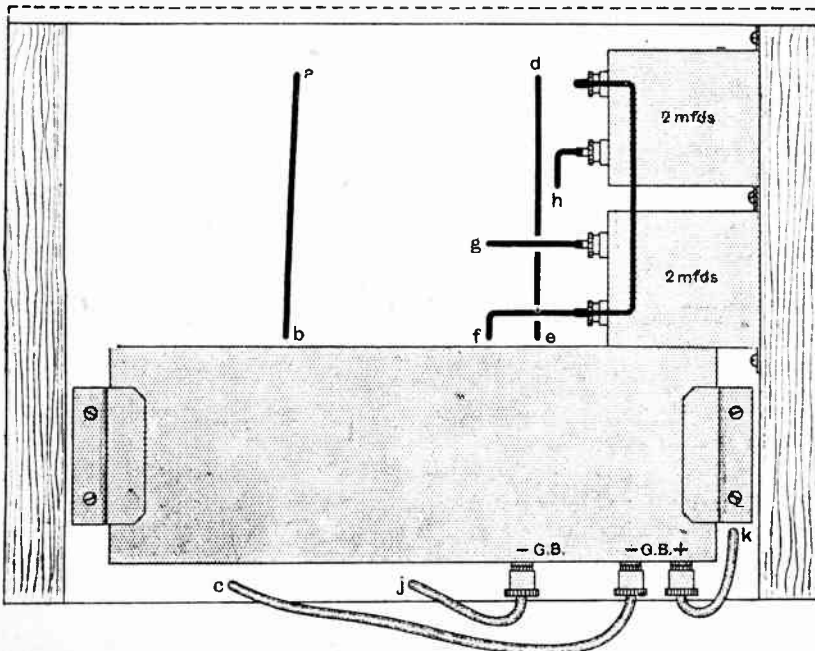
Fig. 5.—Details of underside of baseboard.
