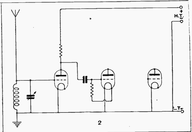
The anode circuit is completed through a high resistance and the H.T. battery. Voltage variations across this resistance are applied to the grid of the detector valve through a condenser, with leak connected to the positive filament lead.
