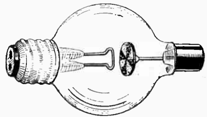
Two-electrode tungar rectifier valve.
