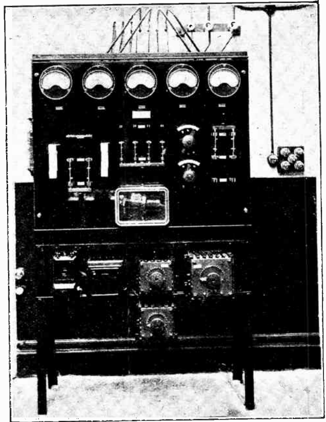
Main battery switchboard in the control room
