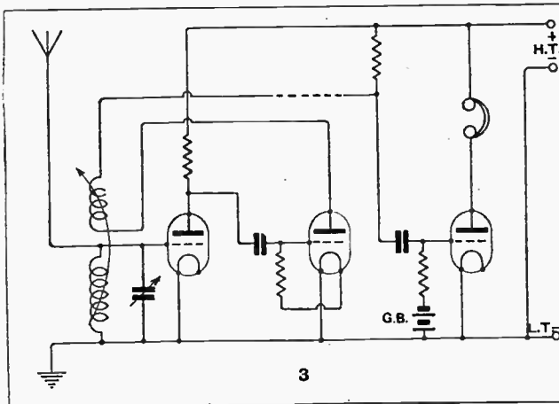
The anode circuit of the detector is connected through reaction coil and resistance to the H.T. battery. L.F. voltages are impressed on the grid through a large condenser, a negative bias being applied through the leak. Phones are inserted in the anode circuit of the L.F. valve.
