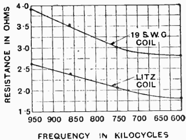
Variation of the H.F. resistance with wavelength and frequency.
