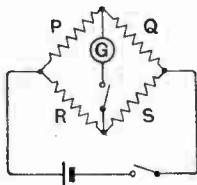
Wheatstone bridge method of measuring resistance.
