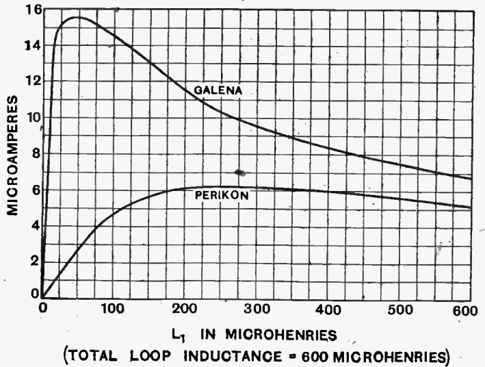
Fig. 6.—Curves showing the optimum values of detector circuit tapping point with galena and Perikon crystals. (Reactance of total loop inductance = 3,130 \text{ ohms} .)
