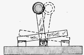
Change-over switch with limited movement.
