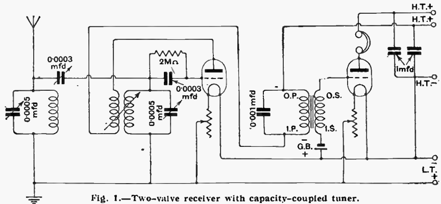
Fig. 1.—Two-valve receiver with capacity-coupled tuner.
