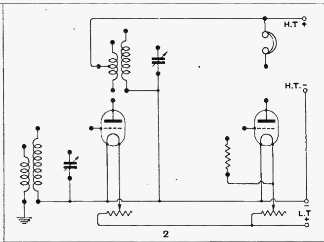
The remainder of the low potential leads are indicated above. Coils and condensers, etc., are added for the sake of clearness.
