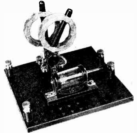
An easily constructed crystal set making use of variometer tuning, constructed in accordance with the Blackadda service sheet No. 1.
