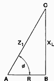
Fig. 4.—Impedance triangle for a tuning coil.
