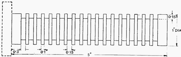
Fig. 2.—Constructional details of the anode resistance.
