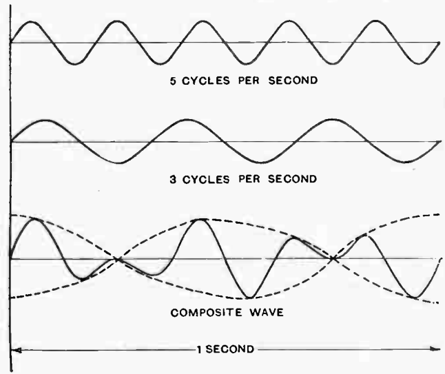
Fig. 3.—A beat frequency of 2 cycles per second produced by the combination of waves with frequencies of 5 and 3 cycles per second respectively.
