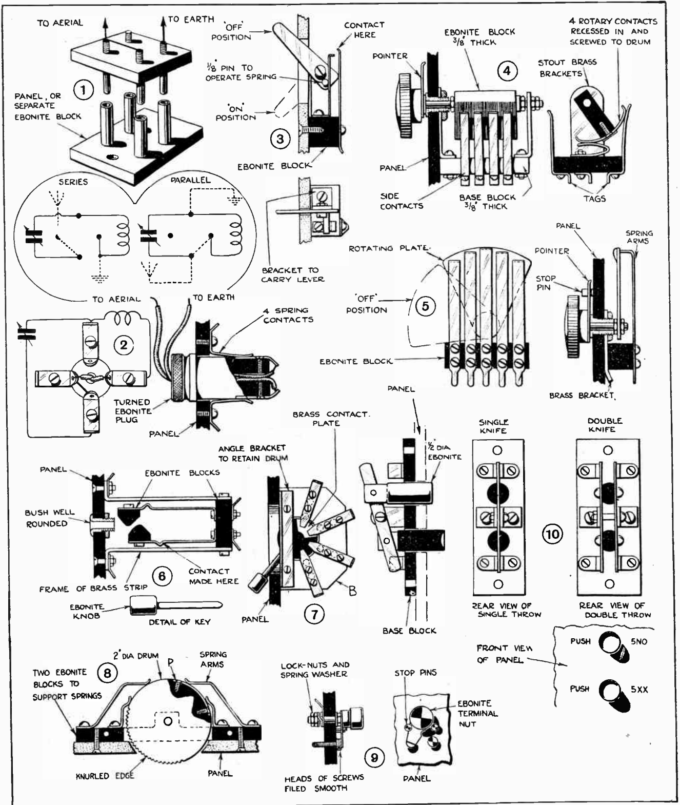
SWITCHES FOR HOME CONSTRUCTION. (1) and (2) Series-parallel switches. (3) Single-pole lever switch. (4) Four-pole change-over switch. (5) Dead-end short-circuiting switch. (6) Key switch (7) Drum switch with side contacts. (8) Drum switch. (9) Single-way switch (10) Single- and two-pole press switches.
