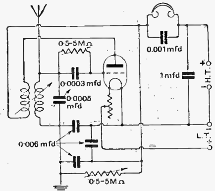
Fig. 3.—The Flewelling super-regenerative circuit.
