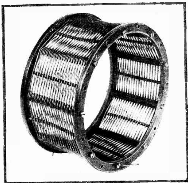
A very good coil, only slightly less efficient than the winning coil. Bare wire is used, and the turns are carefully spaced.
