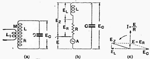
Fig. 2.—(a) Circuit in which the applied E.M.F. is induced into the inductive coil. (b) Series circuit which is electrically equivalent to (a). (c) Vector diagram for complete resonance where E_L = E_C
