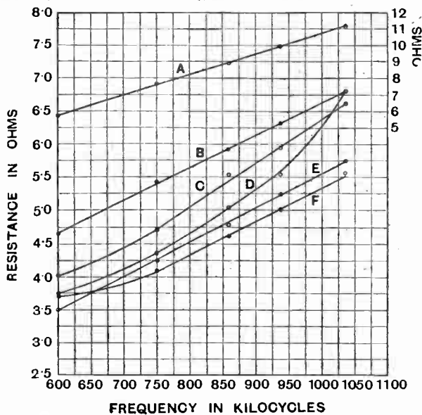
Curve A—3in. diameter space-wound coil of No. 25 D.S.C. wire, with 0.6 megohm shunt resistance, the scale being indicated on the right-hand side of the curve; B—3in. diameter tight-wound coil of No. 26 D.C.C. wire; C—3in. diameter Litz coil; D—3in. diameter tight-wound coil of No. 24 D.C.C. wire; E—3in. diameter space-wound coil of No. 24 D.S.C. wire; F—3in. diameter space-wound coil of No. 25 D.S.C. wire.
