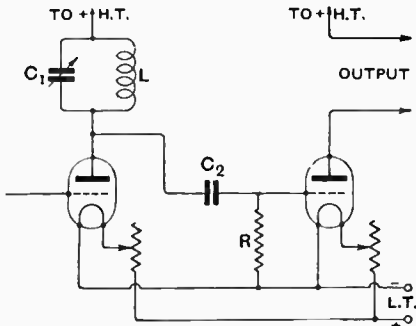
Tuned anode high-frequency valve coupling.
