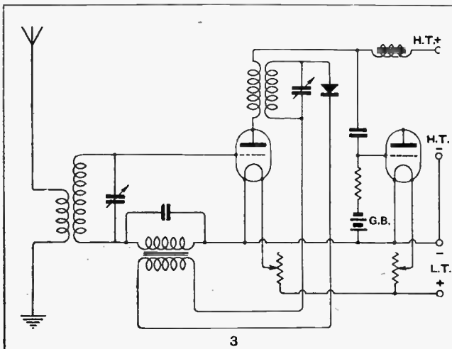
A choke is inserted in the anode circuit of the first valve, L.F. voltages set up across it being applied to the second grid through a condenser, which insulates the grid from the H.T. battery. A leak and bias battery are connected as shown.
