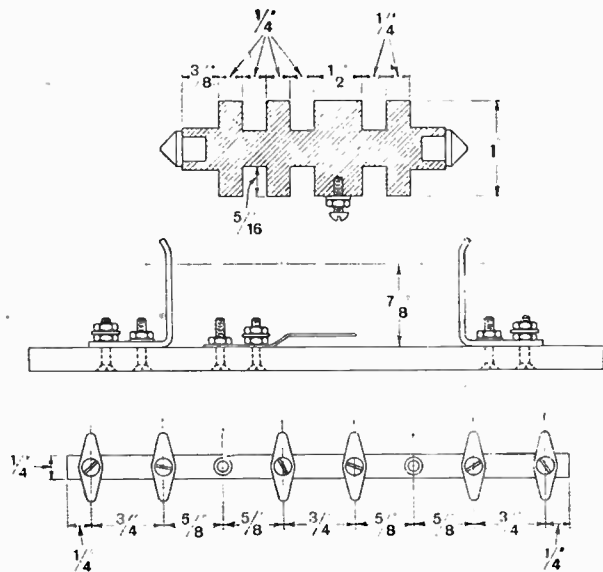
Fig. 8.—Details of the resistance coil former, mounting and terminal strip.
