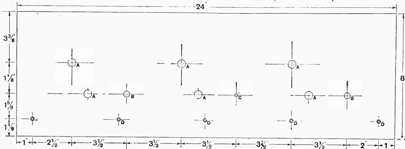
Fig. 3.—Dimensioned drawing of the ebonite front panel. A, 1" dia.; B, 3/8" dia.; C, 1/8" dia.; D, 1/2" dia., and countersunk for No. 4 wood screws.
