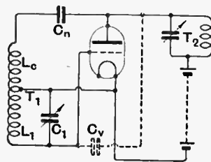
Fig. 1.—Method of neutralising adopted in the receiver.
