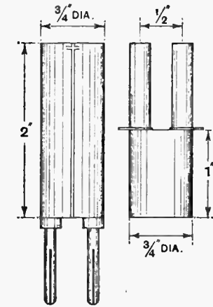
Fig. 4.—Former and socket mounting for H.F. choke coils.
