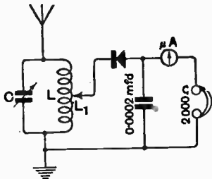
Fig. 1.—Circuit used in obtaining the curves of Figs. 2, 3 and 4.
