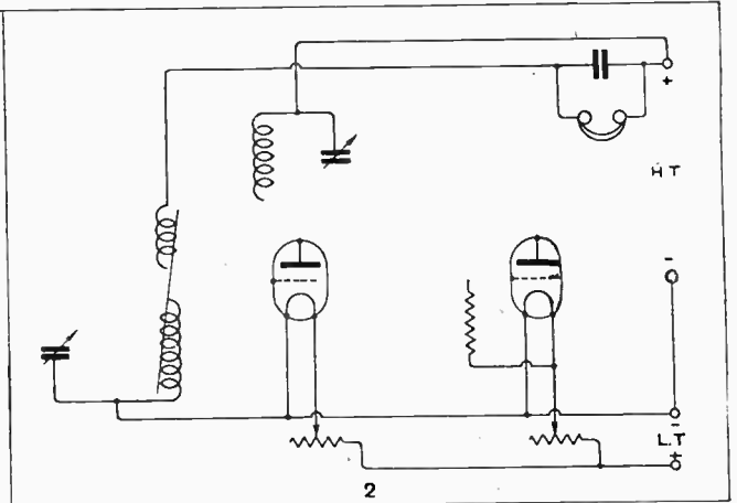
The remainder of the low-potential leads are put on. This diagram should be studied in conjunction with the complete circuit (No. 4).
