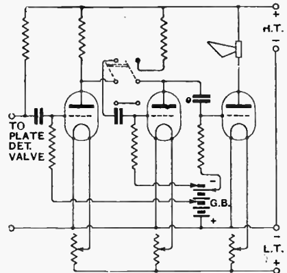
Fig. 1.—Switching a three-valve resistance-capacity coupled amplifier.
