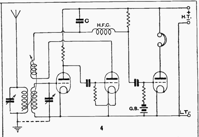
Resistance-coupled H.F. amplification affords no selectivity in itself; therefore the addition of a coupled aerial circuit as shown is particularly desirable. H.F. impulses in the detector anode circuit are deflected through the by-pass condenser C by the insertion of a choke.
