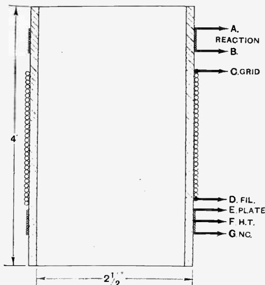
Fig. 4.—Construction of the H.F. transformer.
