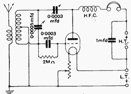
Fig. 3.—A well-known transmitter circuit adapted for reception.
