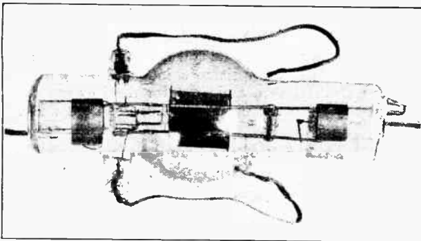
NEW SHORT-WAVE TRANSMITTING VALVE. Of American manufacture, the electrodes of this new valve have been designed so that the total capacity of the circuit will not necessarily lie mainly within the valve itself. Under normal conditions the plate can be operated at a dull red and plate voltages between 1,000 and 3,000 used with a current from 40 to 50 milliamperes.
