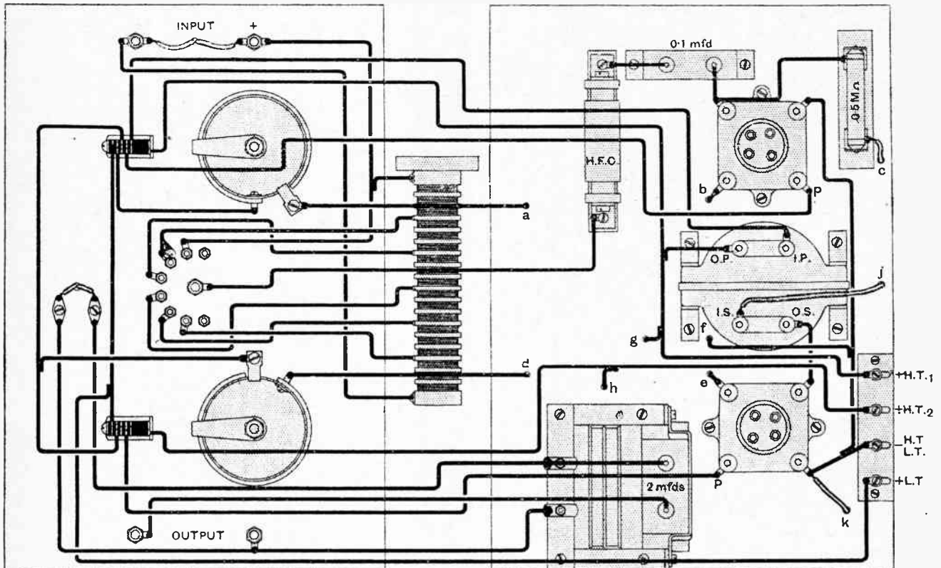
Fig. 6.—The practical wiring diagram.
