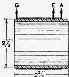
Fig. 3—Construction of the aerial grid coil.
