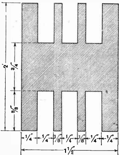
Fig. 1.—Former for I.F. transformers.
