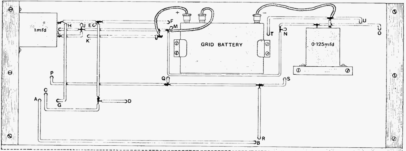
Wiring connections on the underside of the baseboard.
