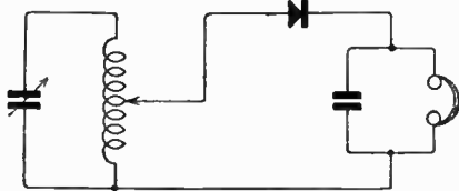
Fig. 1.—Crystal connections.
