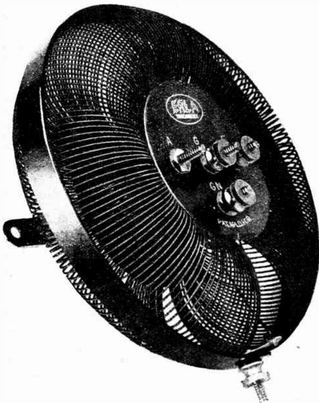
A Toroidal coil, known as the "Erla" Balloon Circloid. Its inductance is 218 microhenries and it has 173 turns of No. 26 D.S.C. wire, a diameter of 1 1/2 in. and an outside diameter of 5 in.
