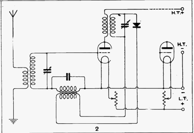
—an H.F. transformer, across the secondary of which is connected a crystal detector. Rectified pulses are passed back through the primary of an L.F. transformer; the secondary is shunted by a by-pass condenser and inserted in the grid circuit.
