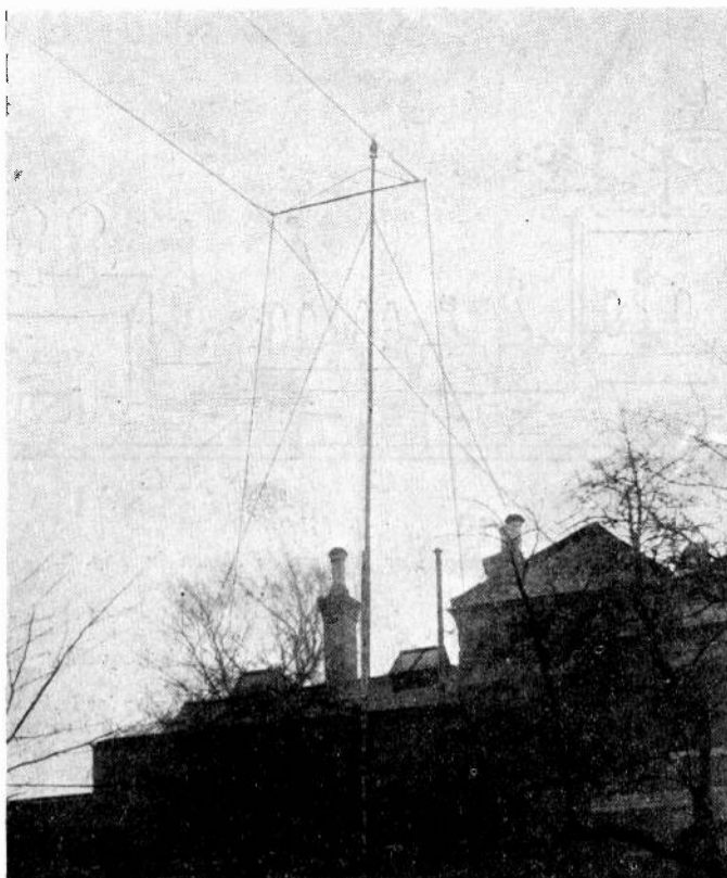
Fig. 1. Aerials used by A.E. Greenslade and E. McT. Reece at the British School of Telegraphy.
