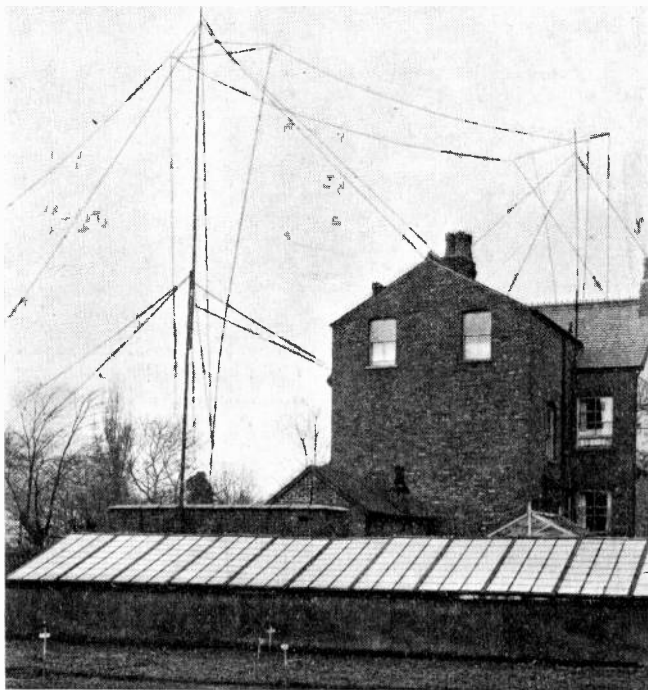
Fig. 1. The Aerials.
