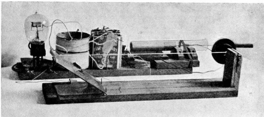
Fig. 4. The Separate Heterodyne.
