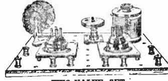
TWO-VALVE SET
