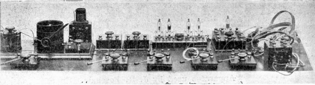
Fig. 4. Simplified Apparatus used by A. E. Greenlade and E. McT. Reece.
