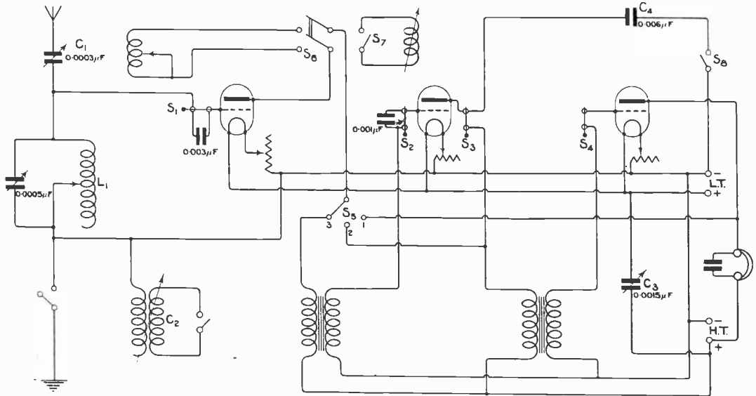
Fig. 6. Circuit Diagram of Mr. Corsham's Apparatus.
