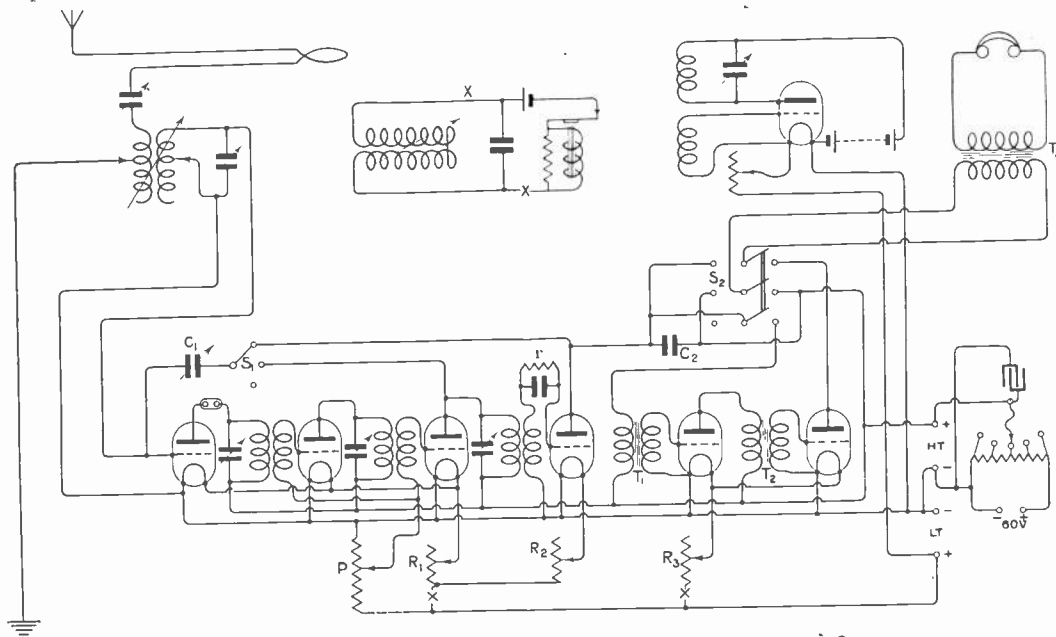
Fig. 10. Circuit Diagram of Mr. Spence's Apparatus.
