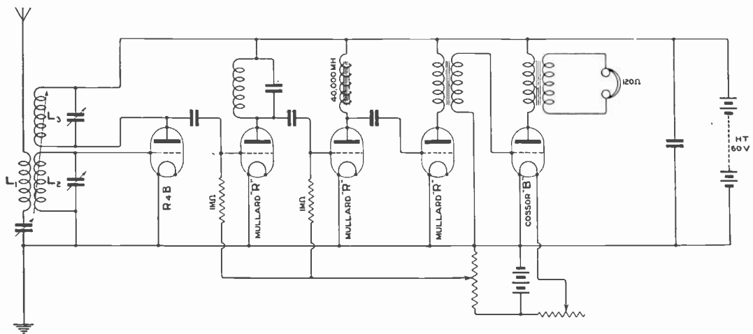
Fig. 2. Circuit Diagram of the Apparatus.
