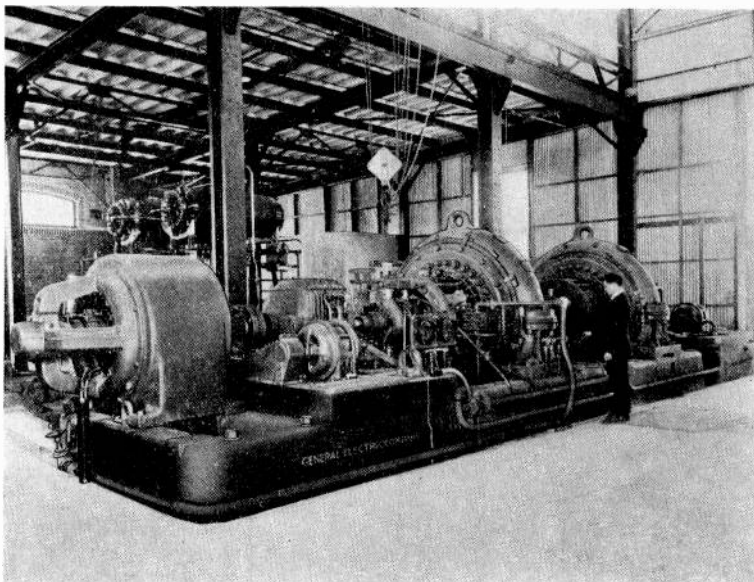
Fig. 4 Two of the 200 kW. Alternators.
