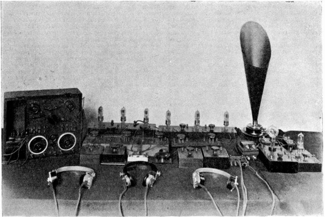
Fig. 2. The Apparatus used by Mr. Burne.
