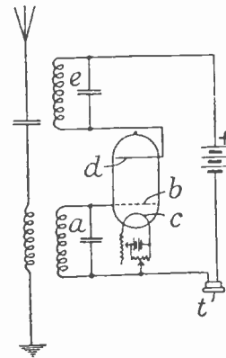
Reproduction of Figure from abridged specification of Patent No. 28,413 of 1913.
