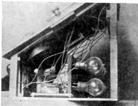
Fig. 9. Side view of the Amplifier.
