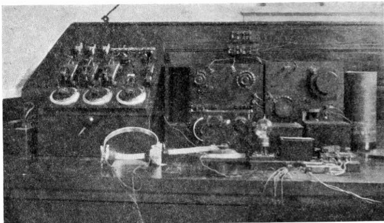
Fig. 7. General view of Receiving Gear.
