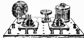
TWO-VALVE SET
