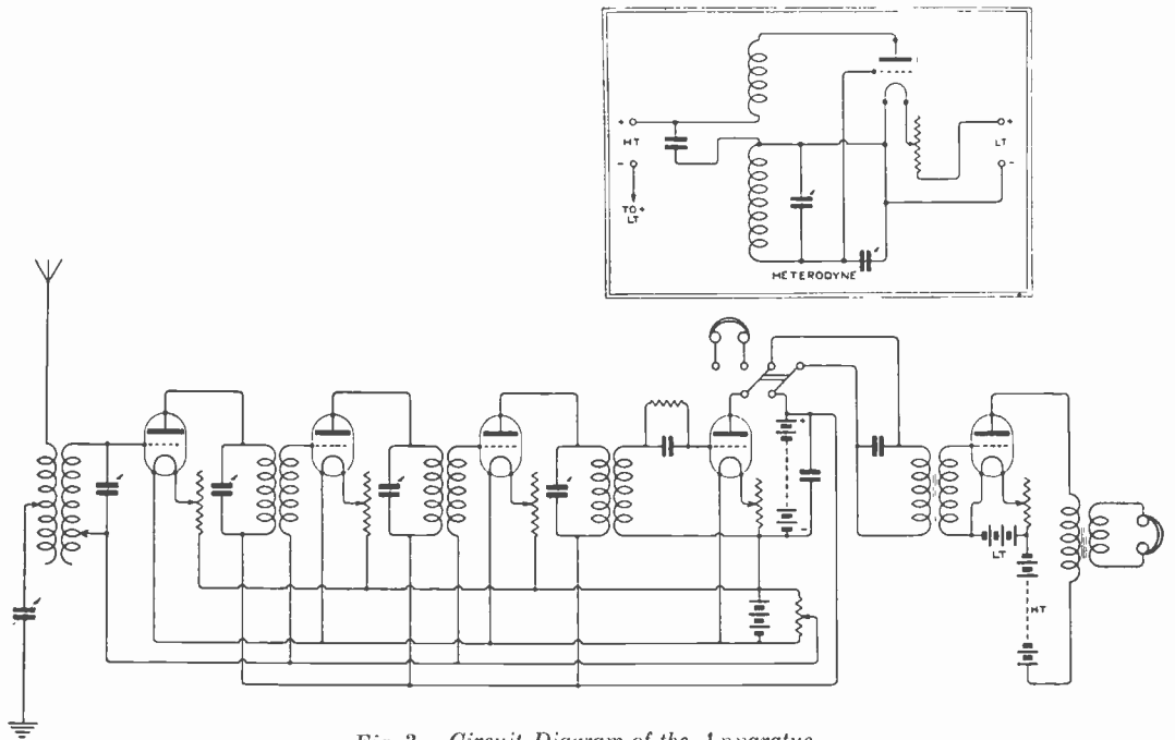
Fig. 3. Circuit Diagram of the Apparatus.
