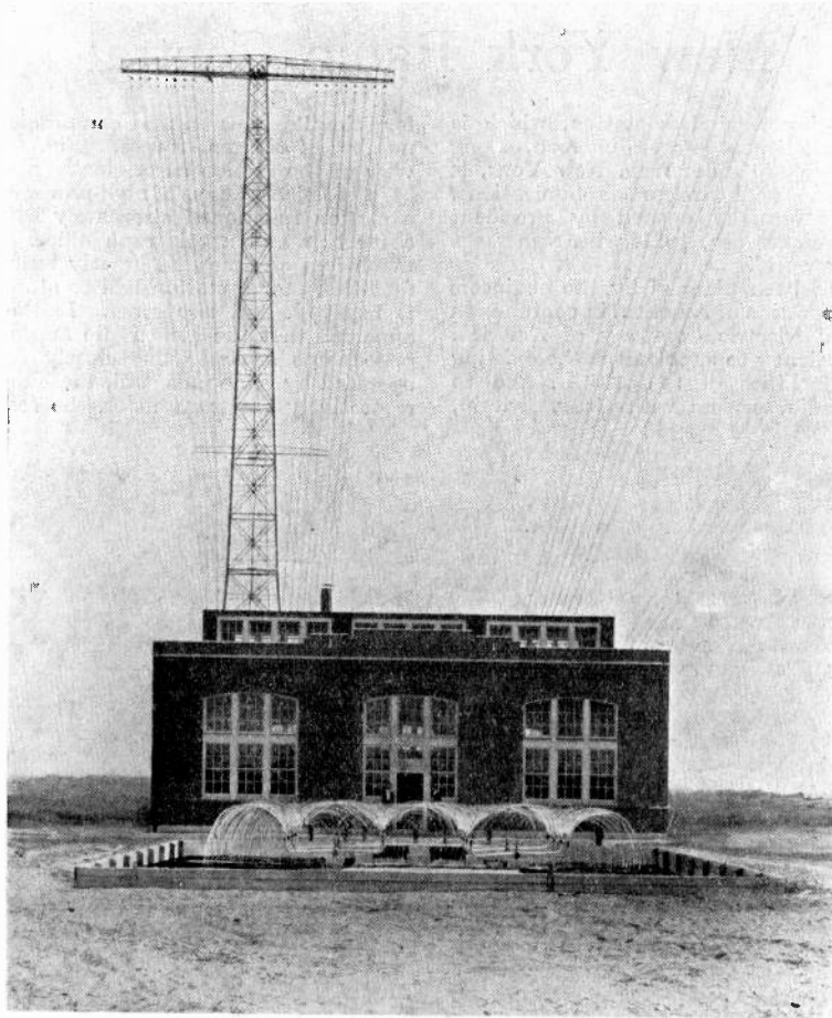
Fig. 2. View of the Power House showing the Cooling Pond in foreground.
