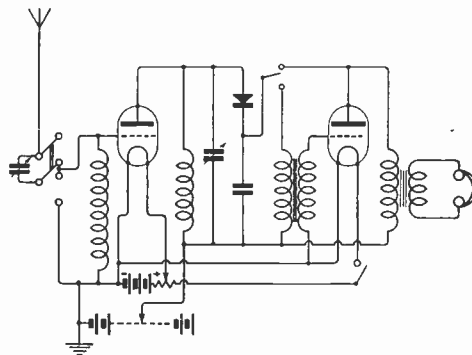
Fig. 6. Circuit diagram of arrangement used by J. R. Forshaw. Both the inductances shown had 30 turns: and the Aerial Tuning Condenser was used in series with the Aerial Circuit.
