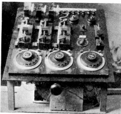
Fig. 8. A near view of the Amplifier.
