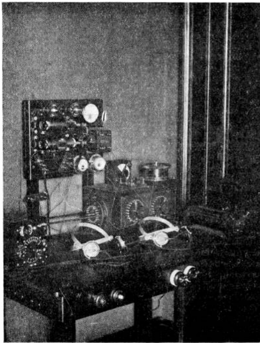
Fig. 1. Mr. J. R. Hoult's Station.
