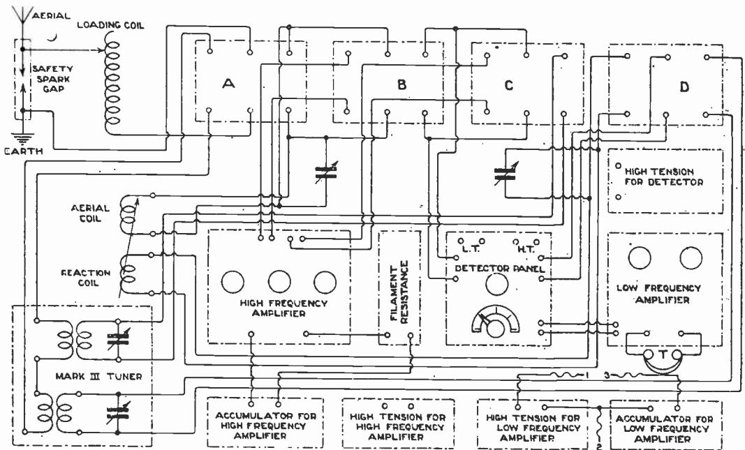
Circuit diagram of the Station.
