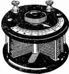
VARIABLE CONDENSERS Die Cast Pattern Enclosed in Celluloid Case, top and base of Bakelite. '0006 ... 25/- '0011 ... 32/6
