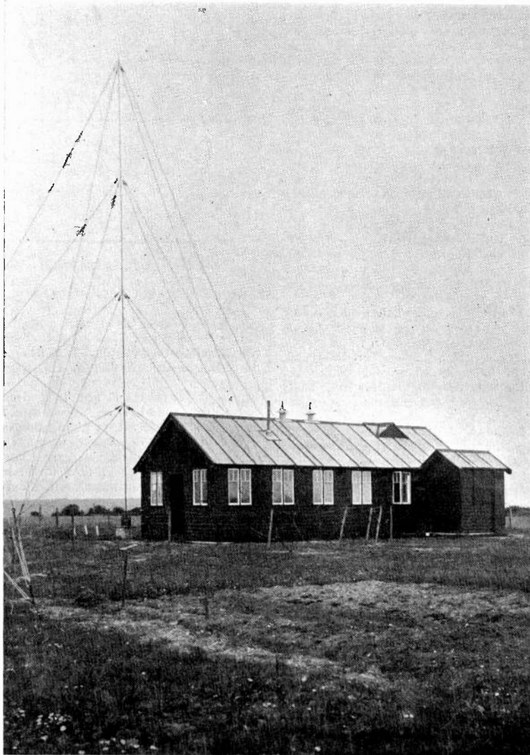
Transmitting Station at Southwold showing mast.
