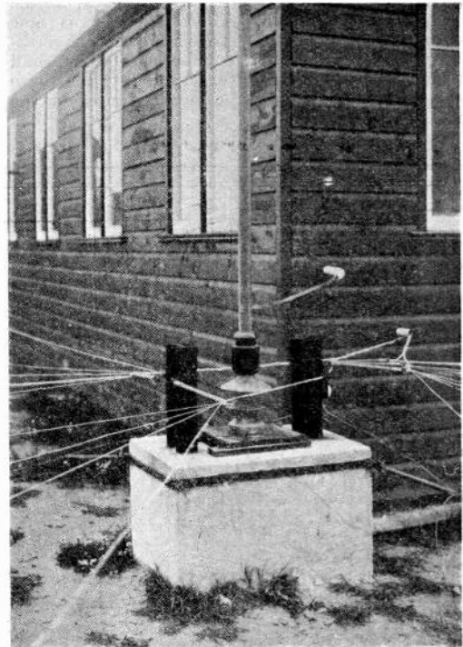
Base of insulated Transmitting Mast at Southwold.
