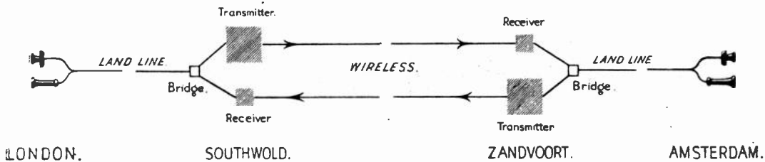
Diagrammatic sketch of the London-Amsterdam circuit.
