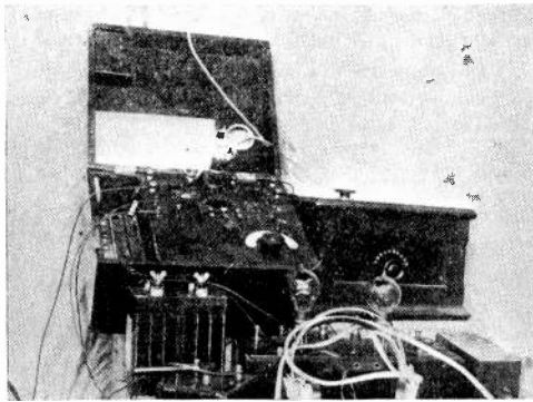
Fig. 1. Apparatus of the 10th Wimbledon Scouts.
