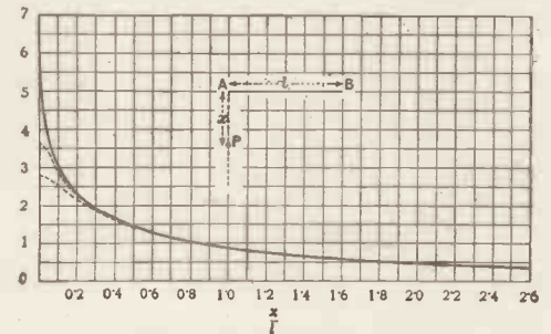
Fig. 24.— \sinh^{-1} \frac{l}{x} = Potential at P due to Unit Charge per Centimetre on AB.
