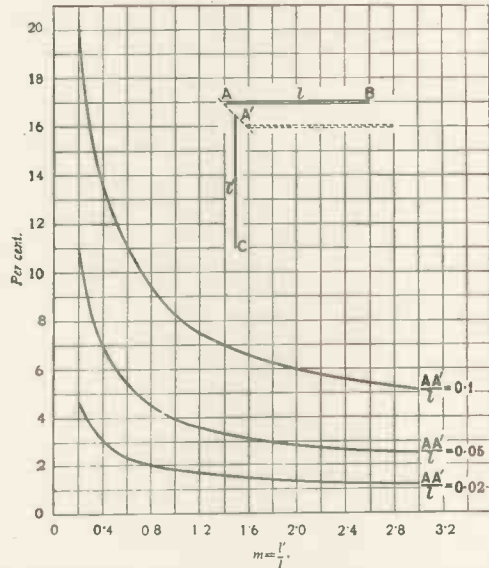
Fig. 26.—The Curves give the Decrease of the Average Potential of A'C Due to the Charge on AB when A and A' do not Coincide.
