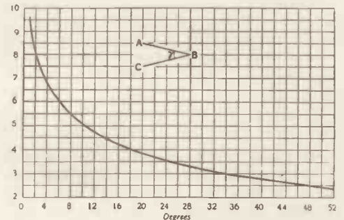
Fig. 28.—Average Potential of AB due to Unit Charge per Centimetre on BC.
