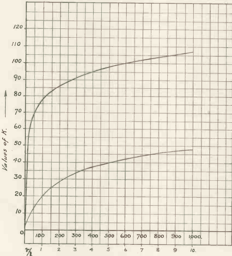
Fig. 1.—Calculation of Induction of a Coil.
