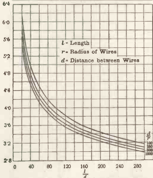
Fig. 12.—Flat Antenna with Seven Wires. Capacity per Foot in Millionths of a Microfarad.
