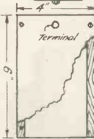
Plan and end view of Stationary plates
