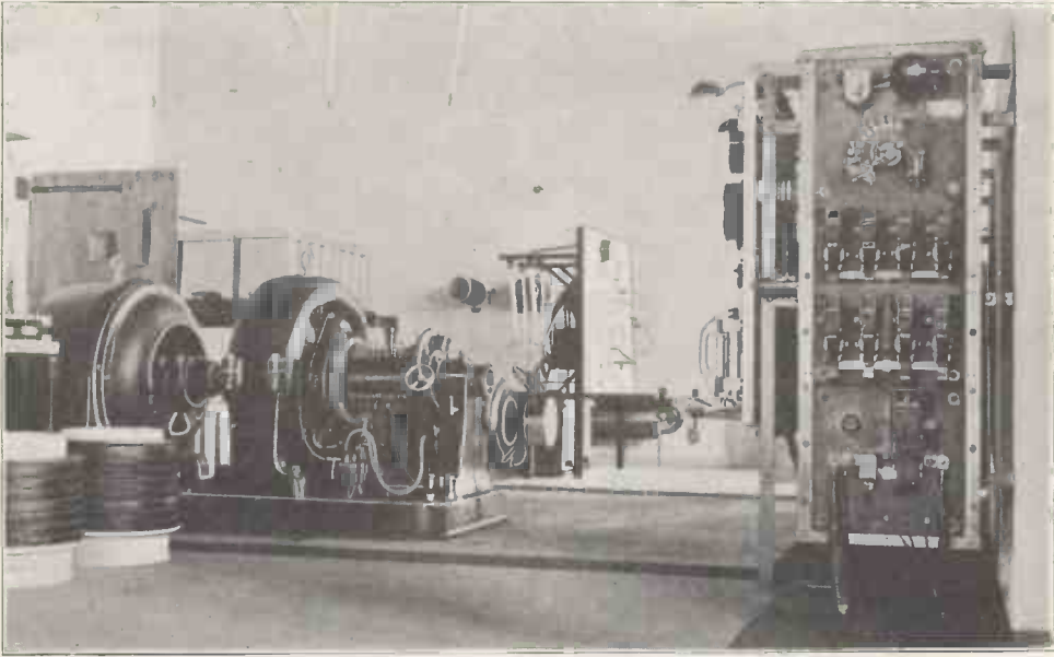
100 k.w. Motor Alternator ; 5 k.w. Transmitter ; A.C. Switchboards, etc.
