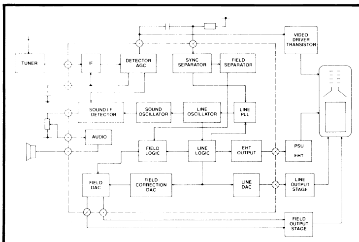
TV block diagram showing integrated circuit and associated components
