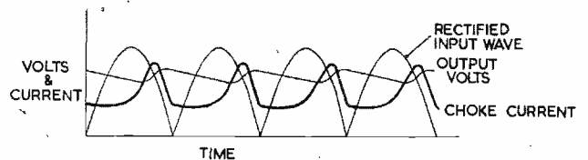
Fig. 3. Conditions of working with the input choke partially saturated
