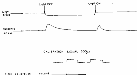
Fig. 3. Shows the response of the eye of a frog to switching off and on the normal room lighting. An upward deflexion signifies the front of the eye is positive with respect to the back. Amplifier A.C. coupled
