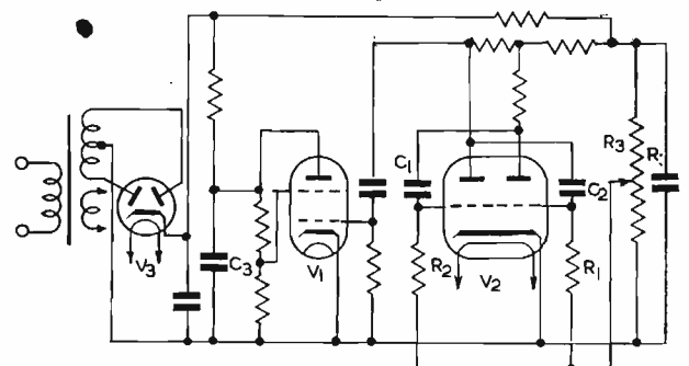
Fig. 2. Circuit diagram of standard commercial pattern Electronic Stroboscope
