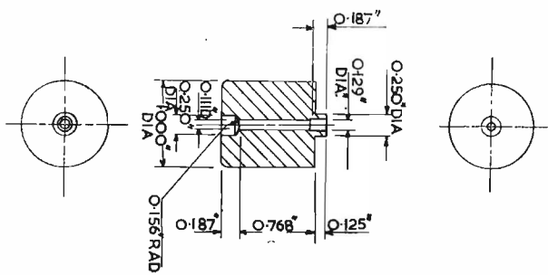
Fig. 19. Acoustic coupler for insert type receivers and 1½cc artificial ear
