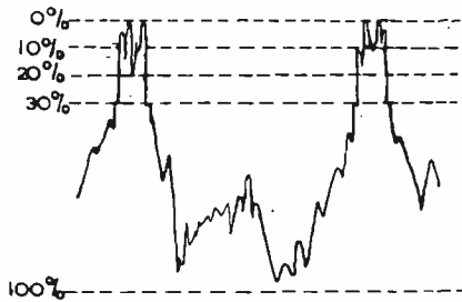
Fig. 14. Typical video signal in the presence of noise modulation
