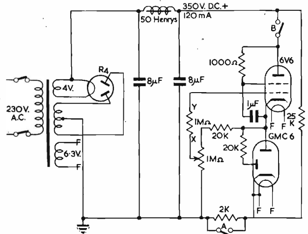
Fig. 3. Typical circuit for modulating a glow tube or crater lamp
