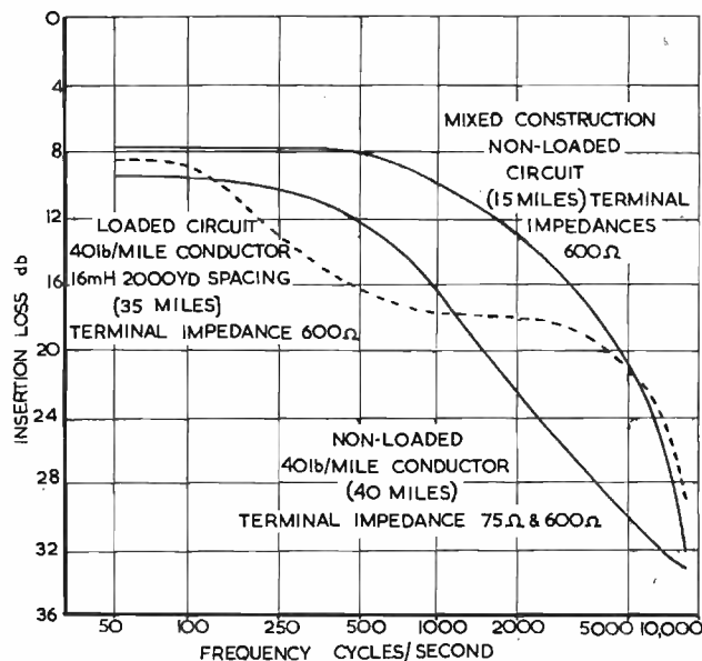
Fig. 2. Insertion loss characteristic
