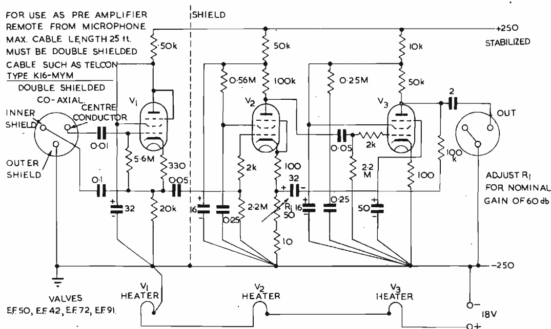
Fig. 15. Microphone pre-amplifier
