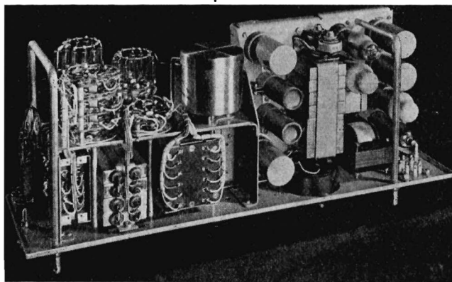
Fig. 9.—Rear view (upper side) of the portable repeater
