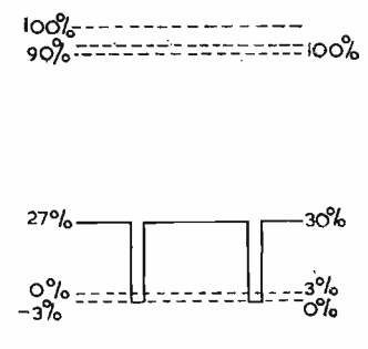
Fig. 12. Restored all black signals when resistance ratio is taken to minimum tolerable
