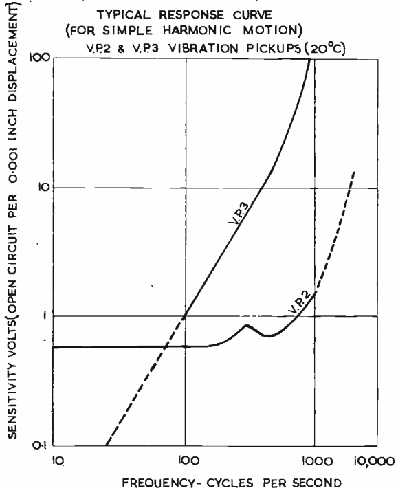
Fig. 17. Frequency response vibration pick-ups
