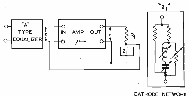
Fig. 5. Basic negative feedback arrangement of the repeater
